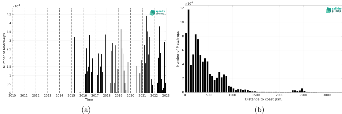
Figure 2: Number of match-ups between TSG (CSIC-UTM) and SMAP SSS L3 v5.3 - 8-Day running (RSS) SSS as a function of time (a) and as function of the distance to coast (b) over the Atlantic Ocean Pi-MEP region and for the full satellite product period.
