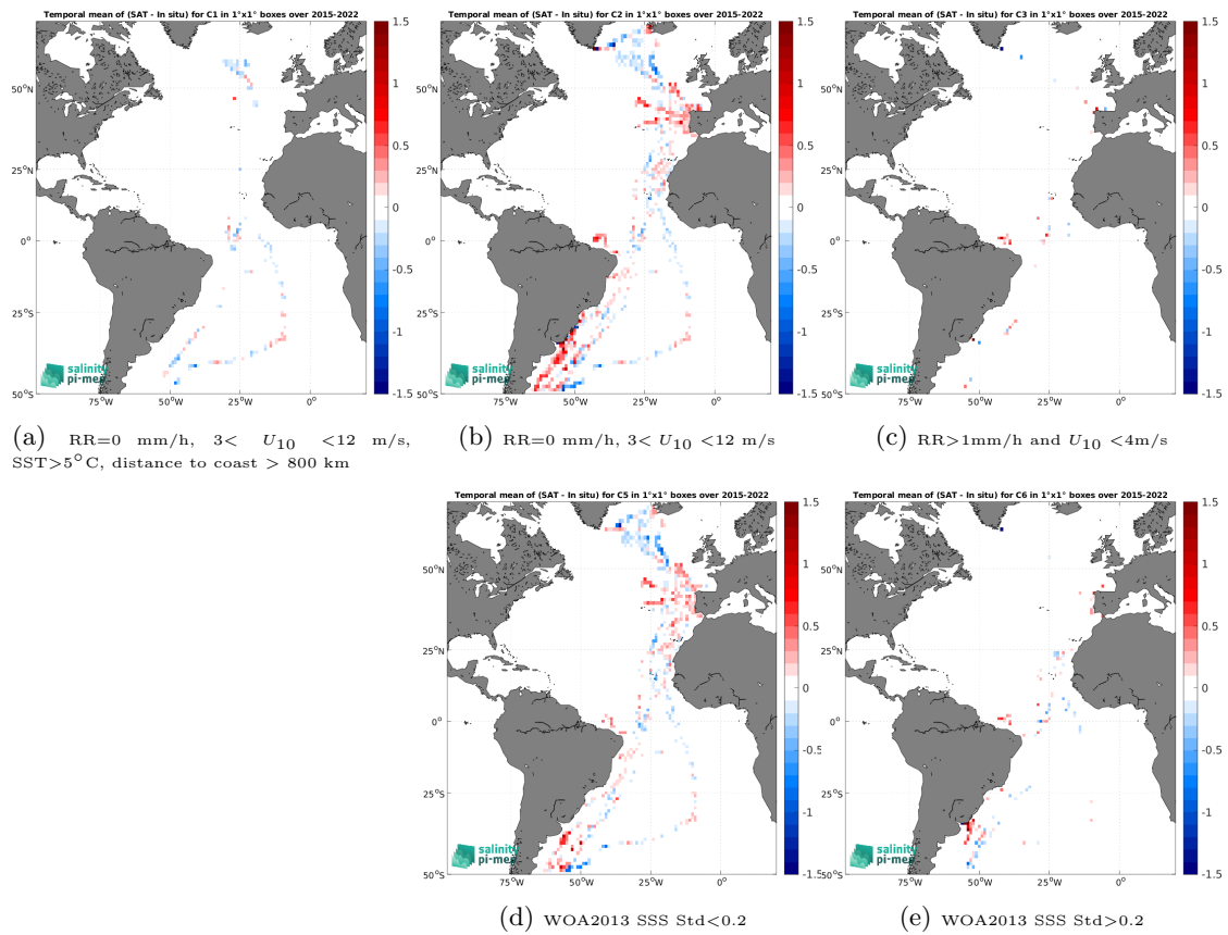
Figure 14: Temporal mean gridded over spatial boxes of size 1^\circ \times 1^\circ of \Delta\text{SSS} (SMAP SSS L3 v5.3 - 8-Day running (RSS) - TSG (CSIC-UTM)) for 5 different subdatasets corresponding to:RR=0 mm/h, 3 < U_{10} < 12 m/s, SST>5°C, distance to coast > 800 km (a), RR=0 mm/h, 3 < U_{10} < 12 m/s (b), RR>1mm/h and U_{10} < 4 m/s (c), WOA2013 SSS Std<0.2 (d), WOA2013 SSS Std>0.2 (e).
