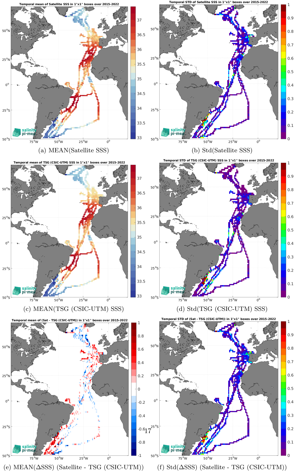
Figure 7: Temporal mean (left) and Std (right) of SSS from SMAP SSS L3 v5.3 - 8-Day running (RSS) (top), TSG (CSIC-UTM) (middle), and of \Delta SSS (Satellite - TSG (CSIC-UTM)). Only match-up pairs are used to generate these maps.
