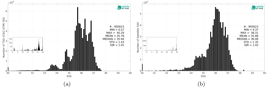
Figure 3: Histograms of SSS from TSG (CSIC-UTM) (a) and SMAP SSS L3 v5.3 - 8-Day running (RSS) (b) considering all match-up pairs per bins of 0.1 over the Atlantic Ocean Pi-MEP region and for the full satellite product period.
