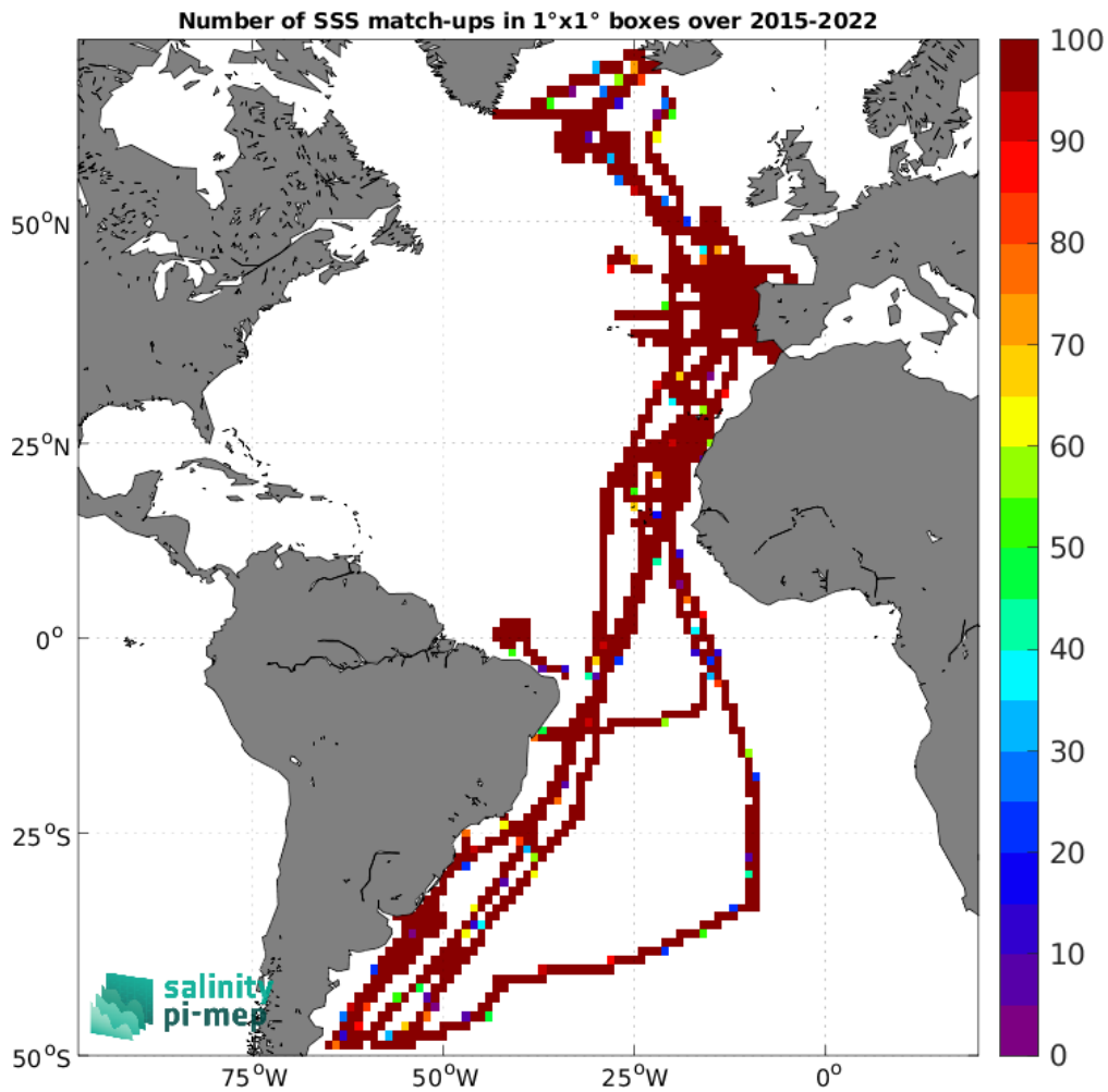
Figure 5: Number of SSS match-ups between TSG (CSIC-UTM) SSS and the SMAP SSS L3 v5.3 - 8-Day running (RSS) SSS product for the Atlantic Ocean Pi-MEP region over 1°×1° boxes and for the full satellite product period.
