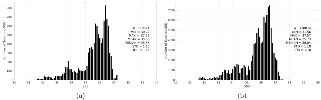
Figure 3: Histograms of SSS from Sairdrone (a) and SMAP SSS L3 v5.3 - 8-Day running (RSS) (b) considering all match-up pairs per bins of 0.1 over the Atlantic Ocean Pi-MEP region and for the full satellite product period.
