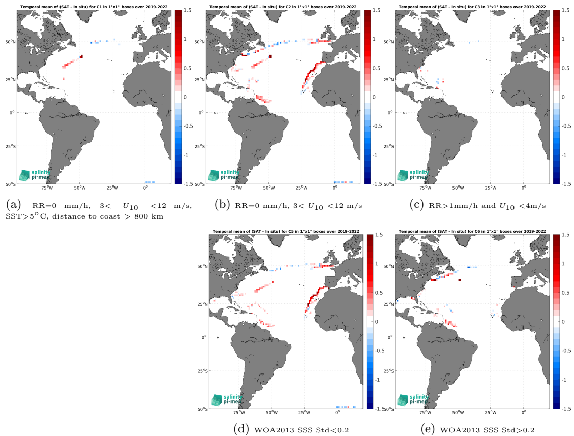
Figure 14: Temporal mean gridded over spatial boxes of size 1^\circ \times 1^\circ of \Delta SSS (SMAP SSS L3 v5.3 - 8-Day running (RSS) - Saildrone) for 5 different subdatasets corresponding to:RR=0 mm/h, 3 < U_{10} < 12 m/s, SST>5°C, distance to coast > 800 km (a), RR=0 mm/h, 3 < U_{10} < 12 m/s (b), RR>1mm/h and U_{10} < 4 m/s (c), WOA2013 SSS Std<0.2 (d), WOA2013 SSS Std>0.2 (e).
