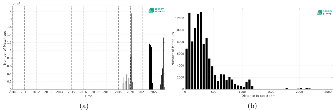
Figure 2: Number of match-ups between Saildrone and SMAP SSS L3 v5.3 - 8-Day running (RSS) SSS as a function of time (a) and as function of the distance to coast (b) over the Atlantic Ocean Pi-MEP region and for the full satellite product period.
