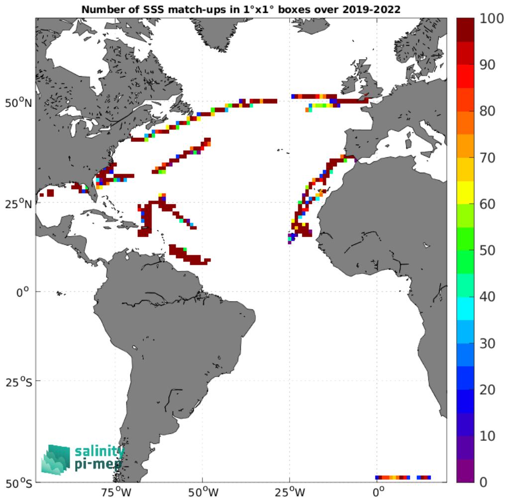
Figure 5: Number of SSS match-ups between Saildrone SSS and the SMAP SSS L3 v5.3 - 8-Day running (RSS) SSS product for the Atlantic Ocean Pi-MEP region over 1^{\circ} \times 1^{\circ} boxes and for the full satellite product period.
