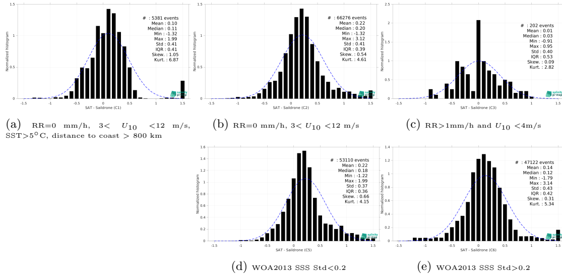
Figure 15: Normalized histogram of \Delta\text{SSS} (SMAP SSS L3 v5.3 - 8-Day running (RSS) - Saildrone) for 5 different subdatasets corresponding to: RR=0 mm/h, 3 < U_{10} < 12 m/s, SST>5°C, distance to coast > 800 km (a), RR=0 mm/h, 3 < U_{10} < 12 m/s (b), RR>1mm/h and U_{10} < 4 m/s (c), WOA2013 SSS Std<0.2 (d), WOA2013 SSS Std>0.2 (e).
