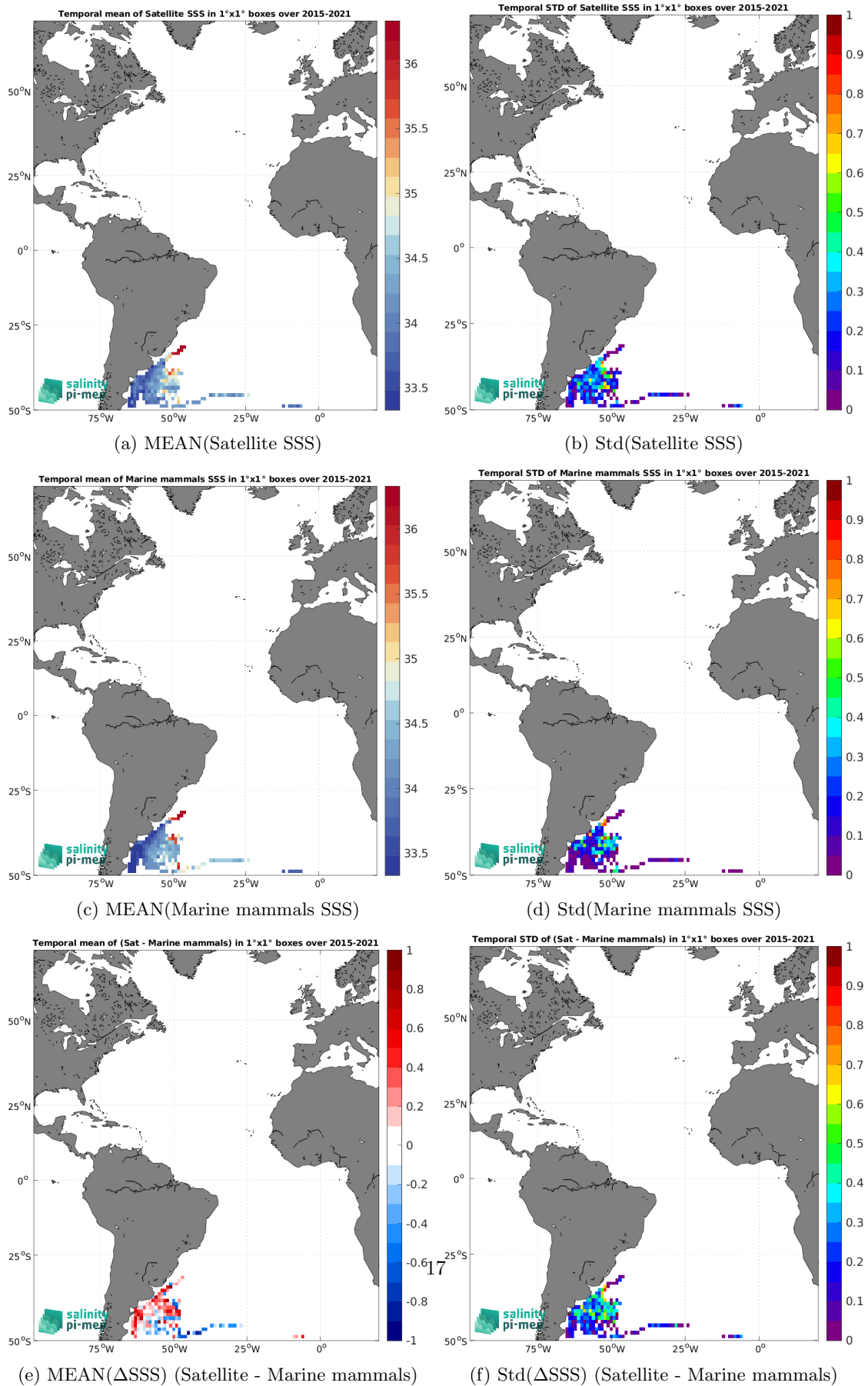
Figure 7: Temporal mean (left) and Std (right) of SSS from SMAP SSS L3 v5.3 - 8-Day running (RSS) (top), Marine mammals (middle), and of \Delta SSS (Satellite - Marine mammals). Only match-up pairs are used to generate these maps.
