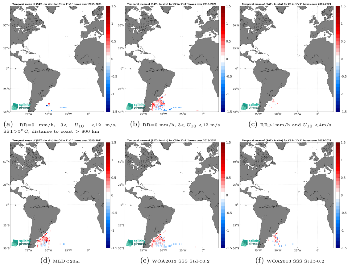
Figure 14: Temporal mean gridded over spatial boxes of size 1^\circ \times 1^\circ of \Delta SSS (SMAP SSS L3 v5.3 - 8-Day running (RSS) - Marine mammals) for 6 different subdatasets corresponding to:RR=0 mm/h, 3 < U_{10} < 12 m/s, SST > 5^\circ\text{C} , distance to coast > 800 km (a), RR=0 mm/h, 3 < U_{10} < 12 m/s (b), RR > 1 mm/h and U_{10} < 4 m/s (c),MLD < 20 m (d),WOA2013 SSS Std < 0.2 (e),WOA2013 SSS Std > 0.2 (f).
