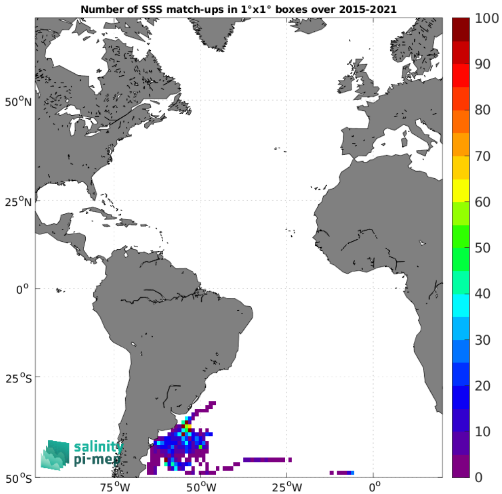
Figure 5: Number of SSS match-ups between Marine mammals SSS and the SMAP SSS L3 v5.3 - 8-Day running (RSS) SSS product for the Atlantic Ocean Pi-MEP region over 1^{\circ} \times 1^{\circ} boxes and for the full satellite product period.
