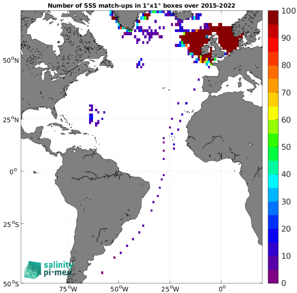
Figure 5: Number of SSS match-ups between ICES SSS and the SMAP SSS L3 v5.3 - 8-Day running (RSS) SSS product for the Atlantic Ocean Pi-MEP region over 1^{\circ} \times 1^{\circ} boxes and for the full satellite product period.
