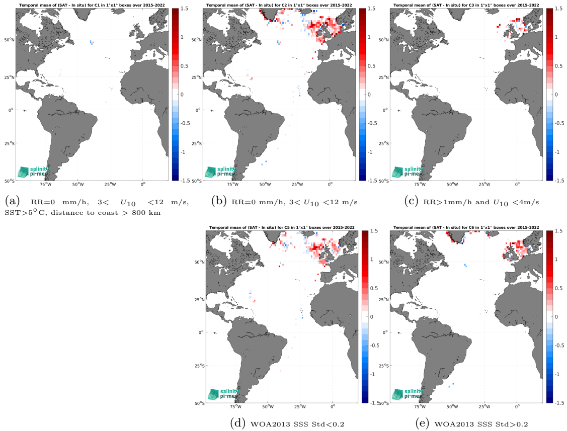
Figure 14: Temporal mean gridded over spatial boxes of size 1^\circ \times 1^\circ of \Delta SSS (SMAP SSS L3 v5.3 - 8-Day running (RSS) - ICES) for 5 different subdatasets corresponding to:RR=0 mm/h, 3 < U_{10} < 12 m/s, SST >5^\circ\text{C} , distance to coast > 800 km (a), RR=0 mm/h, 3 < U_{10} < 12 m/s (b), RR >1 mm/h and U_{10} < 4 m/s (c), WOA2013 SSS Std <0.2 (d), WOA2013 SSS Std >0.2 (e).
