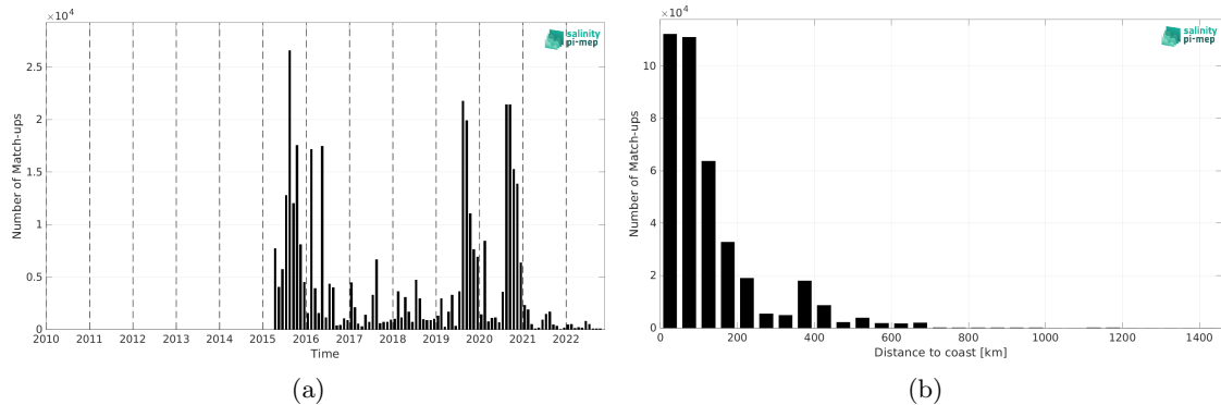
Figure 2: Number of match-ups between ICES and SMAP SSS L3 v5.3 - 8-Day running (RSS) SSS as a function of time (a) and as function of the distance to coast (b) over the Atlantic Ocean Pi-MEP region and for the full satellite product period.
