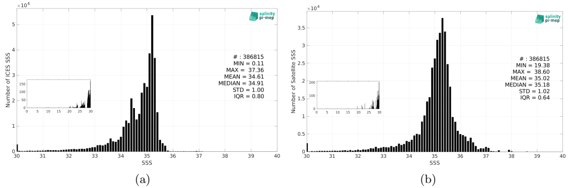
Figure 3: Histograms of SSS from ICES (a) and SMAP SSS L3 v5.3 - 8-Day running (RSS) (b) considering all match-up pairs per bins of 0.1 over the Atlantic Ocean Pi-MEP region and for the full satellite product period.
