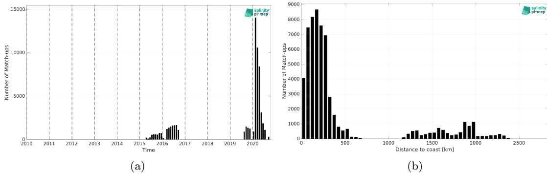
Figure 2: Number of match-ups between Surface drifters and SMAP SSS L3 v5.3 - 8-Day running (RSS) SSS as a function of time (a) and as function of the distance to coast (b) over the Atlantic Ocean Pi-MEP region and for the full satellite product period.
