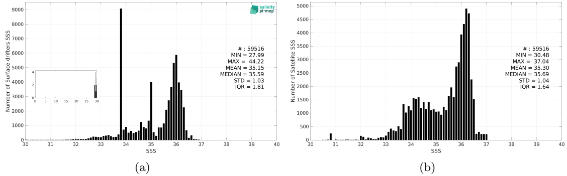
Figure 3: Histograms of SSS from Surface drifters (a) and SMAP SSS L3 v5.3 - 8-Day running (RSS) (b) considering all match-up pairs per bins of 0.1 over the Atlantic Ocean Pi-MEP region and for the full satellite product period.
