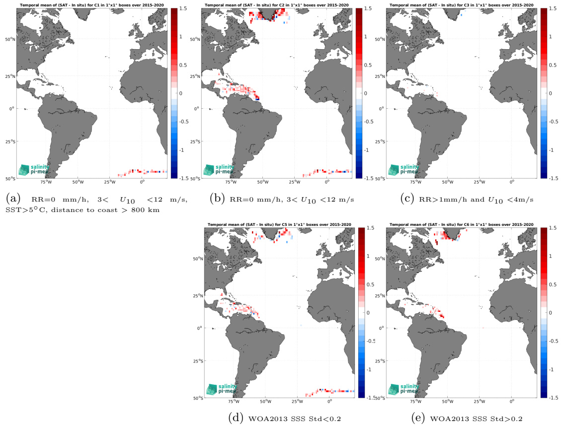
Figure 13: Temporal mean gridded over spatial boxes of size 1^\circ \times 1^\circ of \Delta SSS (SMAP SSS L3 v5.3 - 8-Day running (RSS) - Surface drifters) for 5 different subdatasets corresponding to:RR=0 mm/h, 3 < U_{10} < 12 m/s, SST >5^\circ\text{C} , distance to coast > 800 km (a), RR=0 mm/h, 3 < U_{10} < 12 m/s (b), RR >1 mm/h and U_{10} < 4 m/s (c), WOA2013 SSS Std <0.2 (d), WOA2013 SSS Std >0.2 (e).
