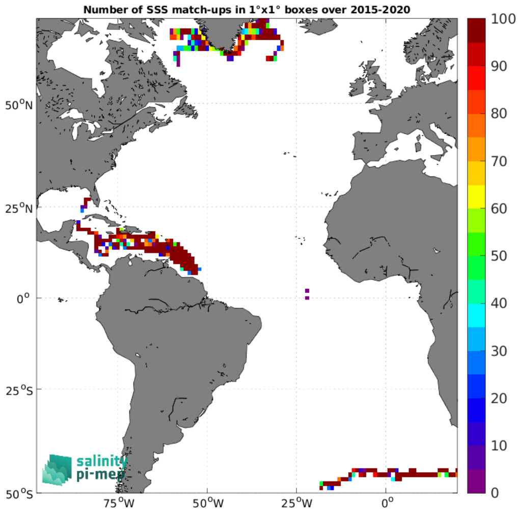
Figure 4: Number of SSS match-ups between Surface drifters SSS and the SMAP SSS L3 v5.3 - 8-Day running (RSS) SSS product for the Atlantic Ocean Pi-MEP region over 1°×1° boxes and for the full satellite product period.
