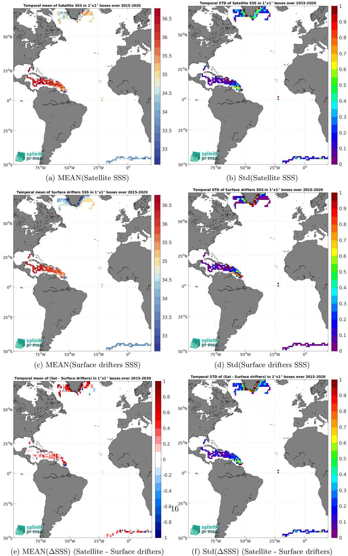
Figure 6: Temporal mean (left) and Std (right) of SSS from SMAP SSS L3 v5.3 - 8-Day running (RSS) (top), Surface drifters (middle), and of \Delta SSS (Satellite - Surface drifters). Only match-up pairs are used to generate these maps.
