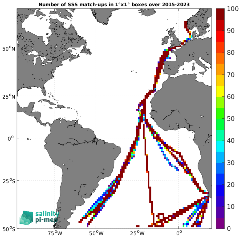
Figure 5: Number of SSS match-ups between TSG (Polarstern) SSS and the SMAP SSS L3 v5.3 - Monthly (RSS) SSS product for the Atlantic Ocean Pi-MEP region over 1°x1° boxes and for the full satellite product period.
