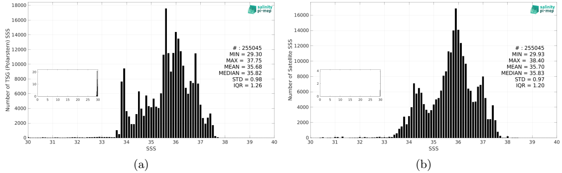
Figure 3: Histograms of SSS from TSG (Polarstern) (a) and SMAP SSS L3 v5.3 - Monthly (RSS) (b) considering all match-up pairs per bins of 0.1 over the Atlantic Ocean Pi-MEP region and for the full satellite product period.
