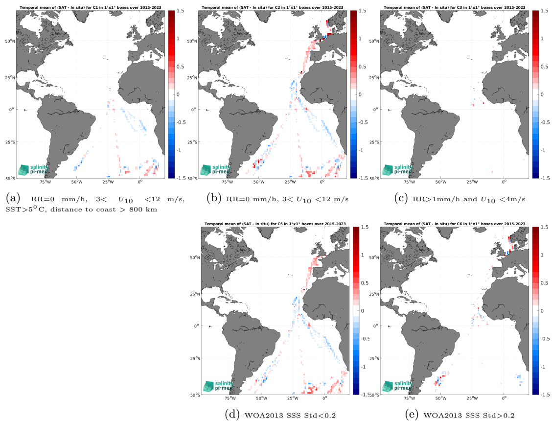
Figure 14: Temporal mean gridded over spatial boxes of size 1^\circ \times 1^\circ of \Delta\text{SSS} (SMAP SSS L3 v5.3 - Monthly (RSS) - TSG (Polarstern)) for 5 different subdatasets corresponding to:RR=0 mm/h, 3 < U_{10} < 12 m/s, SST >5^\circ\text{C} , distance to coast > 800 km (a), RR=0 mm/h, 3 < U_{10} < 12 m/s (b), RR >1 mm/h and U_{10} < 4 m/s (c), WOA2013 SSS Std <0.2 (d), WOA2013 SSS Std >0.2 (e).
