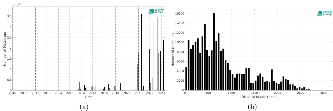
Figure 2: Number of match-ups between TSG (Polarstern) and SMAP SSS L3 v5.3 - Monthly (RSS) SSS as a function of time (a) and as function of the distance to coast (b) over the Atlantic Ocean Pi-MEP region and for the full satellite product period.
