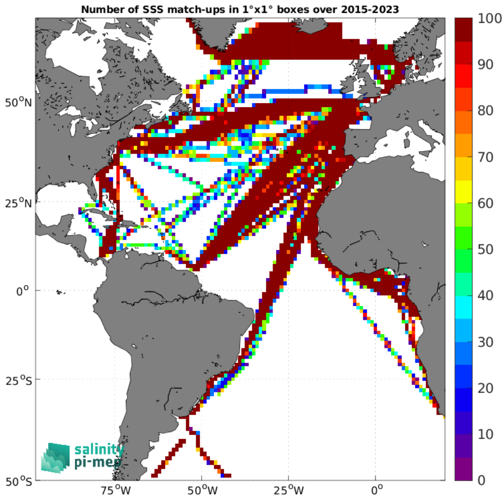
Figure 5: Number of SSS match-ups between TSG (LEGOS-DM) SSS and the SMAP SSS L3 v5.3 - Monthly (RSS) SSS product for the Atlantic Ocean Pi-MEP region over 1^\circ \times 1^\circ boxes and for the full satellite product period.
