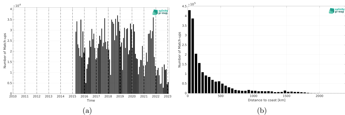
Figure 2: Number of match-ups between TSG (LEGOS-DM) and SMAP SSS L3 v5.3 - Monthly (RSS) SSS as a function of time (a) and as function of the distance to coast (b) over the Atlantic Ocean Pi-MEP region and for the full satellite product period.
