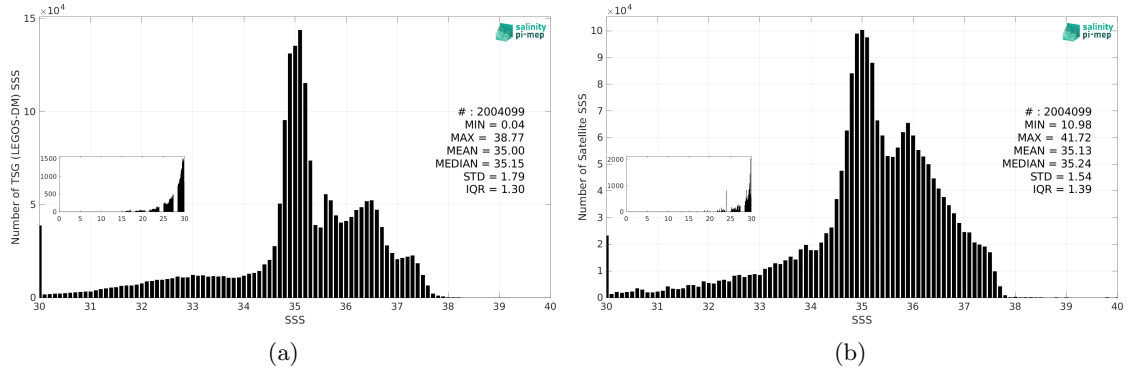
Figure 3: Histograms of SSS from TSG (LEGOS-DM) (a) and SMAP SSS L3 v5.3 - Monthly (RSS) (b) considering all match-up pairs per bins of 0.1 over the Atlantic Ocean Pi-MEP region and for the full satellite product period.
