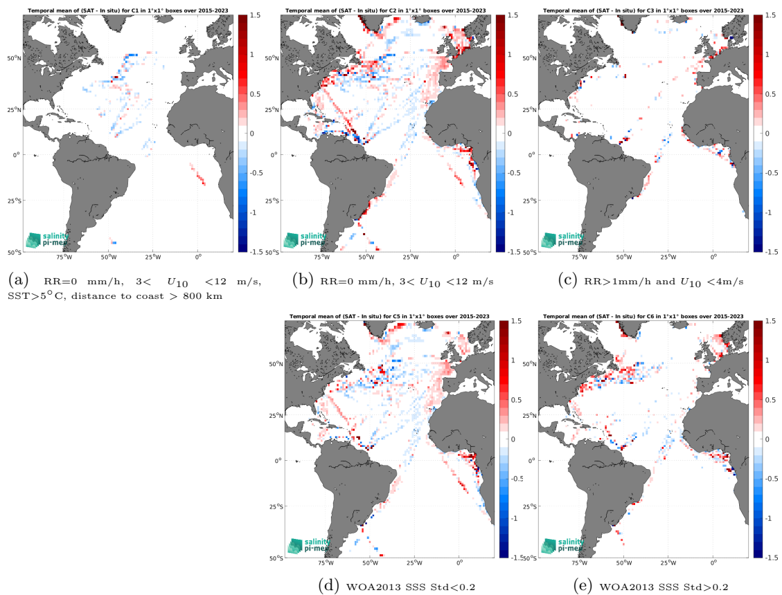
Figure 14: Temporal mean gridded over spatial boxes of size 1^\circ \times 1^\circ of \Delta\text{SSS} (SMAP SSS L3 v5.3 - Monthly (RSS) - TSG (LEGOS-DM)) for 5 different subdatasets corresponding to:RR=0 mm/h, 3 < U_{10} < 12 m/s, SST>5°C, distance to coast > 800 km (a), RR=0 mm/h, 3 < U_{10} < 12 m/s (b), RR>1mm/h and U_{10} < 4 m/s (c), WOA2013 SSS Std<0.2 (d), WOA2013 SSS Std>0.2 (e).
