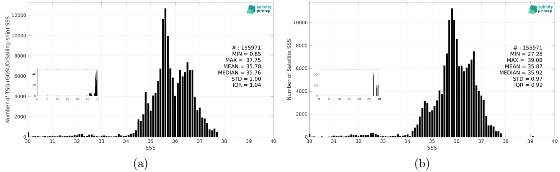
Figure 3: Histograms of SSS from TSG (GOSUD-Sailing-ship) (a) and SMAP SSS L3 v5.3 - Monthly (RSS) (b) considering all match-up pairs per bins of 0.1 over the Atlantic Ocean Pi-MEP region and for the full satellite product period.
