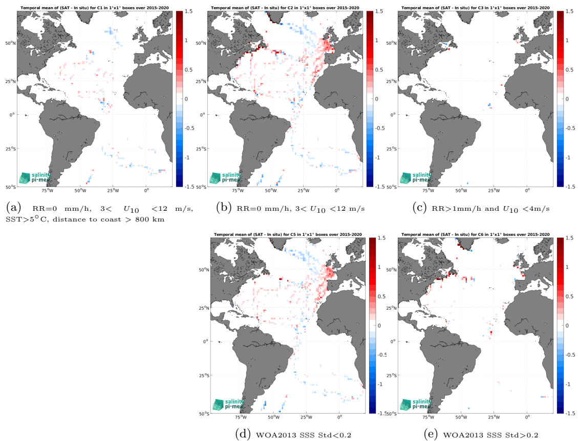
Figure 14: Temporal mean gridded over spatial boxes of size 1^\circ \times 1^\circ of \Delta\text{SSS} (SMAP SSS L3 v5.3 - Monthly (RSS) - TSG (GOSUD-Sailing-ship)) for 5 different subdatasets corresponding to:RR=0 mm/h, 3 < U_{10} < 12 m/s, SST >5^\circ\text{C} , distance to coast > 800 km (a), RR=0 mm/h, 3 < U_{10} < 12 m/s (b), RR >1 mm/h and U_{10} < 4 m/s (c), WOA2013 SSS Std <0.2 (d), WOA2013 SSS Std >0.2 (e).
