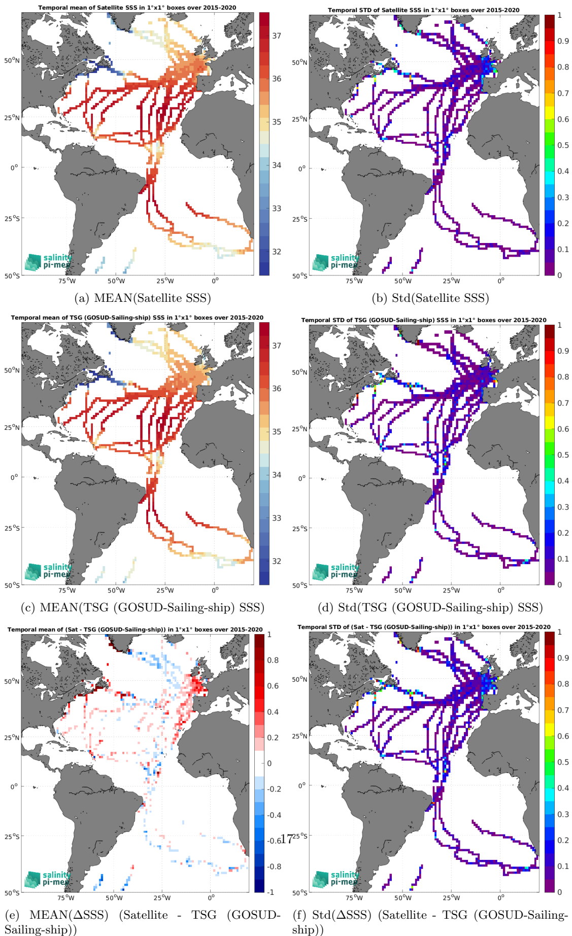
Figure 7: Temporal mean (left) and Std (right) of SSS from SMAP SSS L3 v5.3 - Monthly (RSS) (top), TSG (GOSUD-Sailing-ship) (middle), and of \Delta SSS (Satellite - TSG (GOSUD-Sailing-ship)). Only match-up pairs are used to generate these maps.
