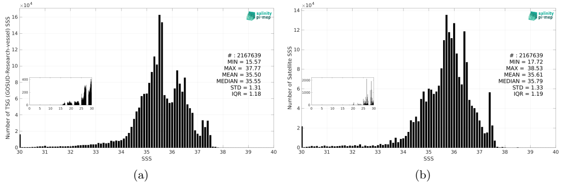
Figure 3: Histograms of SSS from TSG (GOSUD-Research-vessel) (a) and SMAP SSS L3 v5.3 - Monthly (RSS) (b) considering all match-up pairs per bins of 0.1 over the Atlantic Ocean Pi-MEP region and for the full satellite product period.
