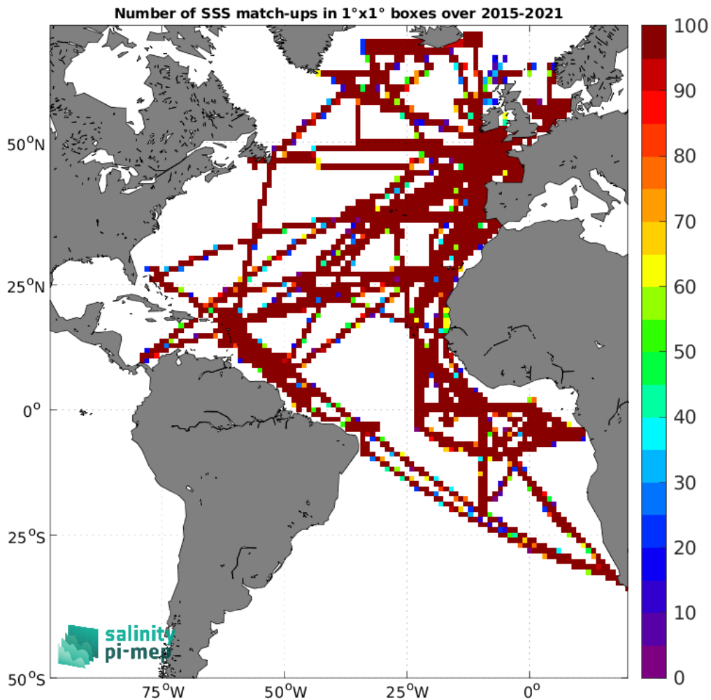
Figure 5: Number of SSS match-ups between TSG (GOSUD-Research-vessel) SSS and the SMAP SSS L3 v5.3 - Monthly (RSS) SSS product for the Atlantic Ocean Pi-MEP region over 1^\circ \times 1^\circ boxes and for the full satellite product period.
