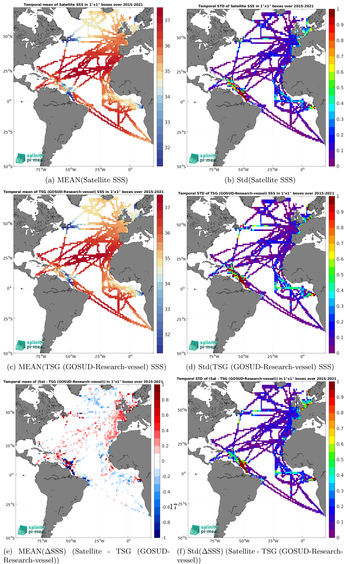
Figure 7: Temporal mean (left) and Std (right) of SSS from SMAP SSS L3 v5.3 - Monthly (RSS) (top), TSG (GOSUD-Research-vessel) (middle), and of \Delta SSS (Satellite - TSG (GOSUD-Research-vessel)). Only match-up pairs are used to generate these maps.
