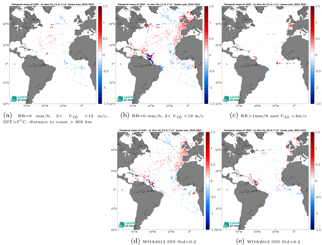
Figure 14: Temporal mean gridded over spatial boxes of size 1^\circ \times 1^\circ of \Delta\text{SSS} (SMAP SSS L3 v5.3 - Monthly (RSS) - TSG (GOSUD-Research-vessel)) for 5 different subdatasets corresponding to:RR=0 mm/h, 3 < U_{10} < 12 m/s, SST >5^\circ\text{C} , distance to coast > 800 km (a), RR=0 mm/h, 3 < U_{10} < 12 m/s (b), RR >1 mm/h and U_{10} < 4 m/s (c), WOA2013 SSS Std <0.2 (d), WOA2013 SSS Std >0.2 (e).
