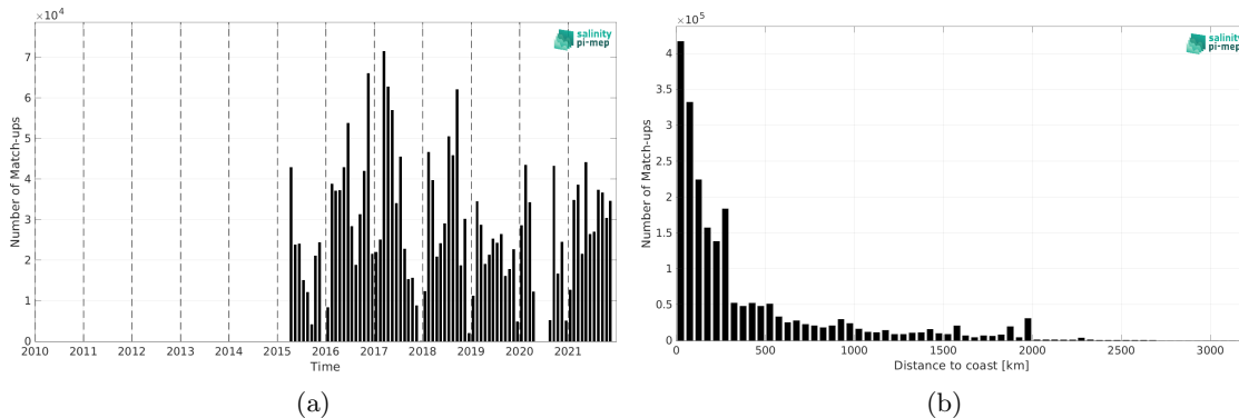
Figure 2: Number of match-ups between TSG (GOSUD-Research-vessel) and SMAP SSS L3 v5.3 - Monthly (RSS) SSS as a function of time (a) and as function of the distance to coast (b) over the Atlantic Ocean Pi-MEP region and for the full satellite product period.
