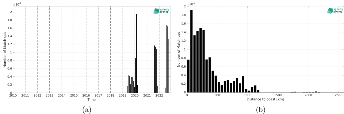
Figure 2: Number of match-ups between Saildrone and SMAP SSS L3 v5.3 - Monthly (RSS) SSS as a function of time (a) and as function of the distance to coast (b) over the Atlantic Ocean Pi-MEP region and for the full satellite product period.
