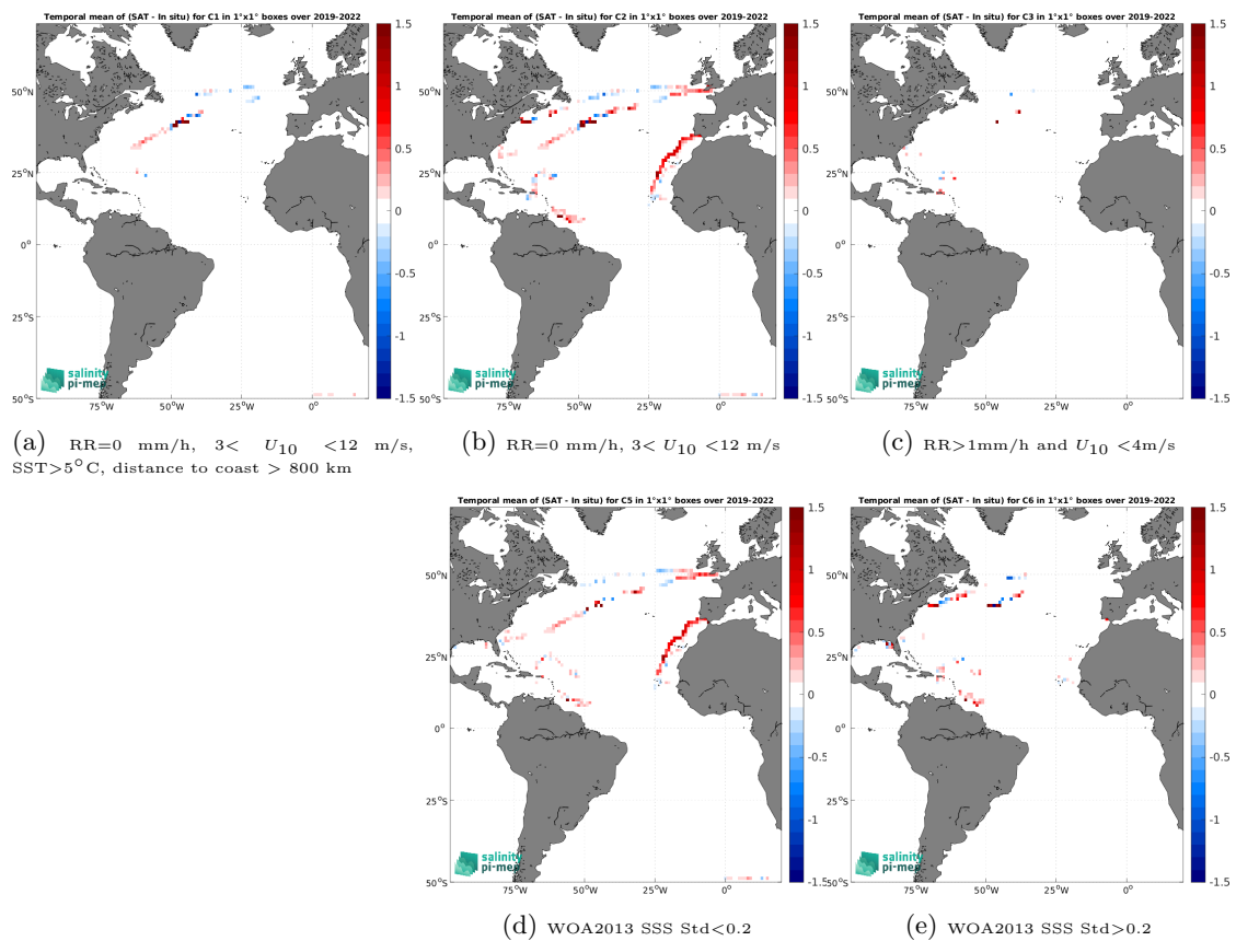
Figure 14: Temporal mean gridded over spatial boxes of size 1^\circ \times 1^\circ of \Delta SSS (SMAP SSS L3 v5.3 - Monthly (RSS) - Saildrone) for 5 different subdatasets corresponding to:RR=0 mm/h, 3 < U_{10} < 12 m/s, SST >5^\circ\text{C} , distance to coast > 800 km (a), RR=0 mm/h, 3 < U_{10} < 12 m/s (b), RR >1 mm/h and U_{10} < 4 m/s (c), WOA2013 SSS Std <0.2 (d), WOA2013 SSS Std >0.2 (e).
