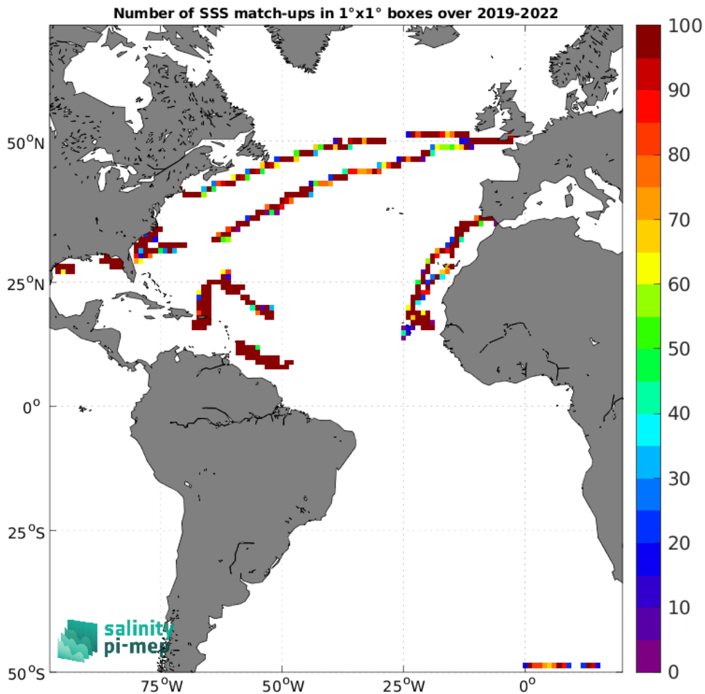
Figure 5: Number of SSS match-ups between Saildrone SSS and the SMAP SSS L3 v5.3 - Monthly (RSS) SSS product for the Atlantic Ocean Pi-MEP region over 1°x1° boxes and for the full satellite product period.
