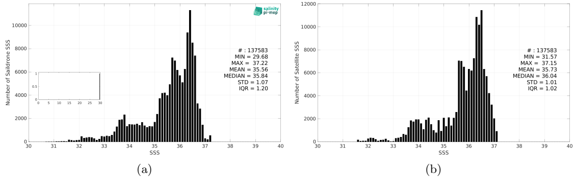
Figure 3: Histograms of SSS from Saildrone (a) and SMAP SSS L3 v5.3 - Monthly (RSS) (b) considering all match-up pairs per bins of 0.1 over the Atlantic Ocean Pi-MEP region and for the full satellite product period.
