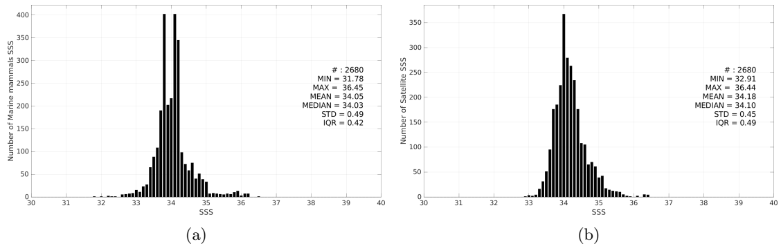
Figure 3: Histograms of SSS from Marine mammals (a) and SMAP SSS L3 v5.3 - Monthly (RSS) (b) considering all match-up pairs per bins of 0.1 over the Atlantic Ocean Pi-MEP region and for the full satellite product period.
