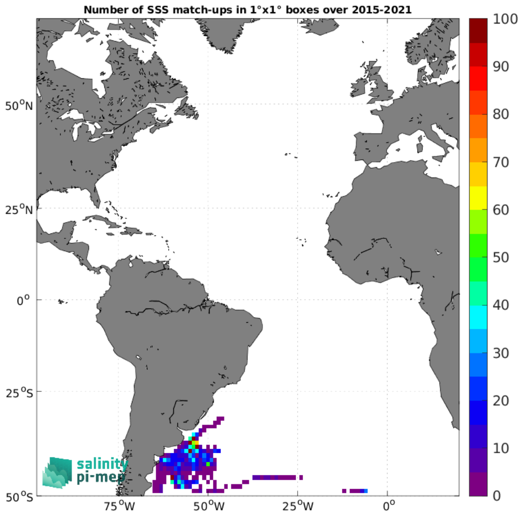
Figure 5: Number of SSS match-ups between Marine mammals SSS and the SMAP SSS L3 v5.3 - Monthly (RSS) SSS product for the Atlantic Ocean Pi-MEP region over 1°x1° boxes and for the full satellite product period.
