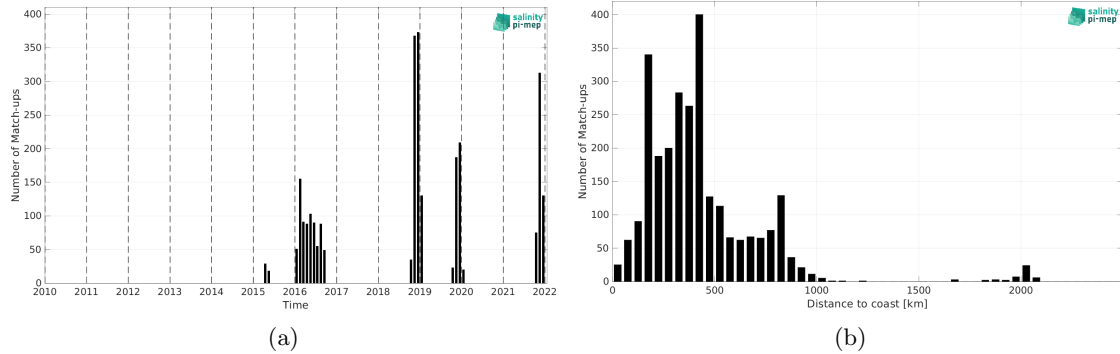
Figure 2: Number of match-ups between Marine mammals and SMAP SSS L3 v5.3 - Monthly (RSS) SSS as a function of time (a) and as function of the distance to coast (b) over the Atlantic Ocean Pi-MEP region and for the full satellite product period.
