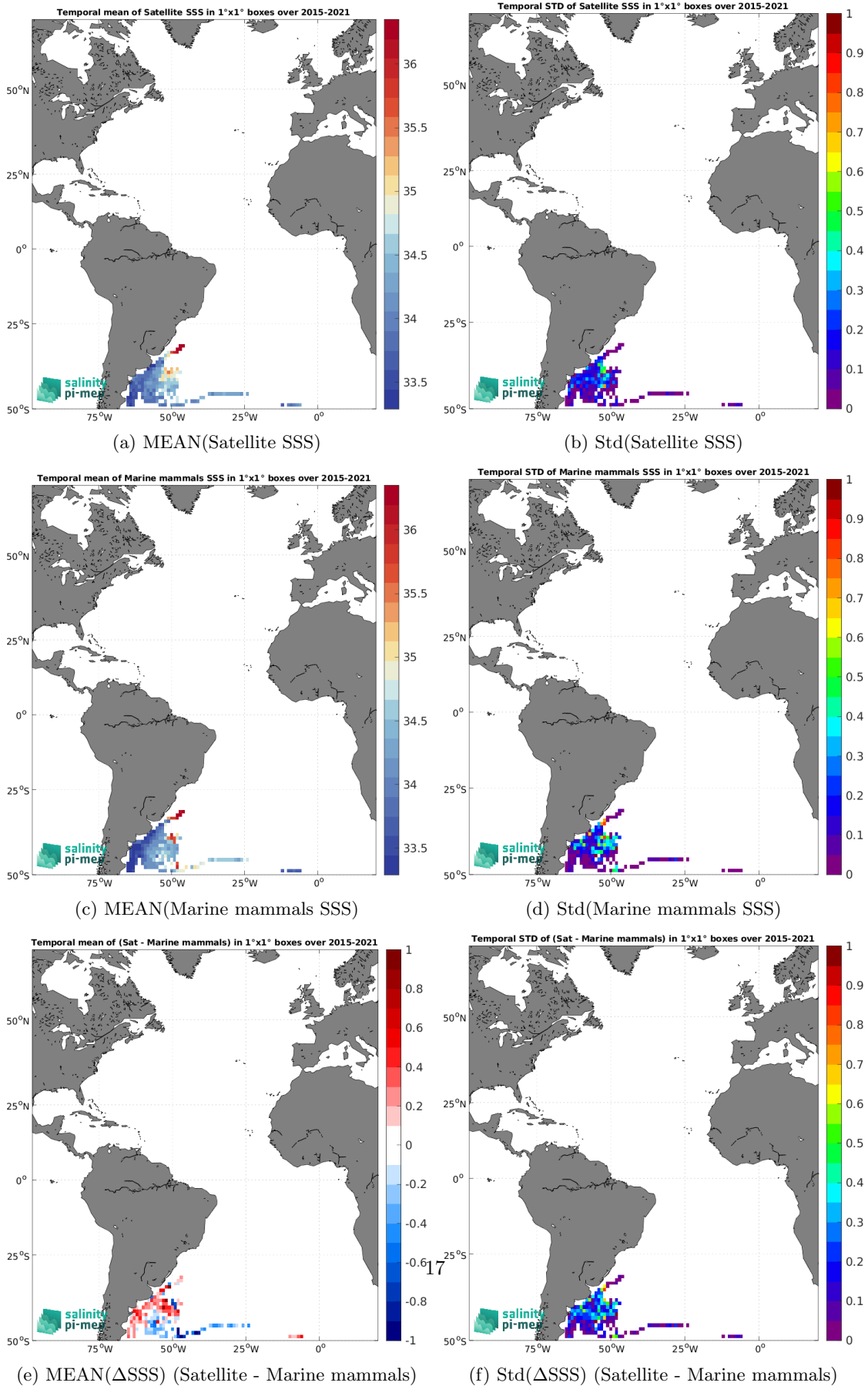
Figure 7: Temporal mean (left) and Std (right) of SSS from SMAP SSS L3 v5.3 - Monthly (RSS) (top), Marine mammals (middle), and of \Delta SSS (Satellite - Marine mammals). Only match-up pairs are used to generate these maps.
