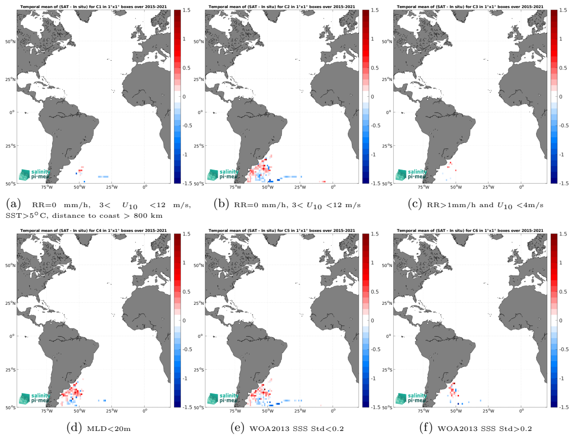
Figure 14: Temporal mean gridded over spatial boxes of size 1^\circ \times 1^\circ of \Delta SSS (SMAP SSS L3 v5.3 - Monthly (RSS) - Marine mammals) for 6 different subdatasets corresponding to: RR=0 mm/h, 3 < U_{10} < 12 m/s, SST > 5^\circ\text{C} , distance to coast > 800 km (a), RR=0 mm/h, 3 < U_{10} < 12 m/s (b), RR > 1 mm/h and U_{10} < 4 m/s (c), MLD < 20 m (d), WOA2013 SSS Std < 0.2 (e), WOA2013 SSS Std > 0.2 (f).
