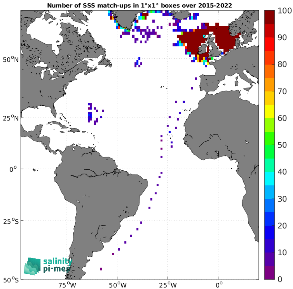
Figure 5: Number of SSS match-ups between ICES SSS and the SMAP SSS L3 v5.3 - Monthly (RSS) SSS product for the Atlantic Ocean Pi-MEP region over 1^{\circ} \times 1^{\circ} boxes and for the full satellite product period.
