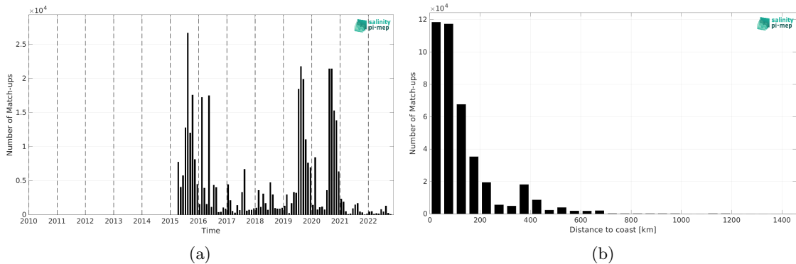
Figure 2: Number of match-ups between ICES and SMAP SSS L3 v5.3 - Monthly (RSS) SSS as a function of time (a) and as function of the distance to coast (b) over the Atlantic Ocean Pi-MEP region and for the full satellite product period.
