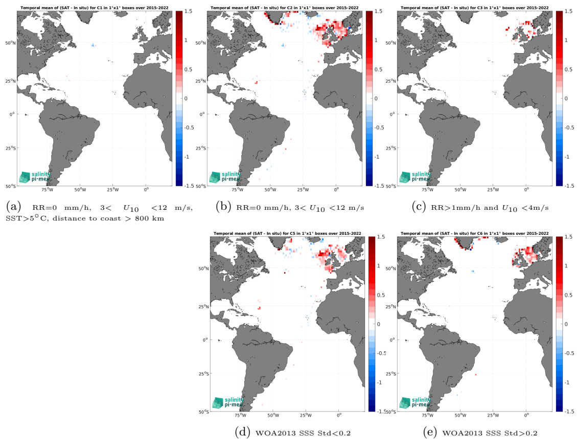
Figure 14: Temporal mean gridded over spatial boxes of size 1^\circ \times 1^\circ of \Delta\text{SSS} (SMAP SSS L3 v5.3 - Monthly (RSS) - ICES) for 5 different subdatasets corresponding to:RR=0 mm/h, 3 < U_{10} < 12 m/s, SST >5^\circ\text{C} , distance to coast > 800 km (a), RR=0 mm/h, 3 < U_{10} < 12 m/s (b), RR >1 mm/h and U_{10} < 4 m/s (c), WOA2013 SSS Std <0.2 (d), WOA2013 SSS Std >0.2 (e).
