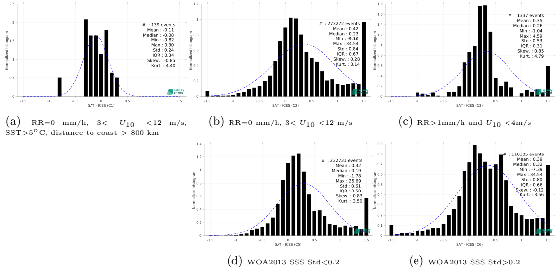
Figure 15: Normalized histogram of \Delta SSS (SMAP SSS L3 v5.3 - Monthly (RSS) - ICES) for 5 different subdatasets corresponding to: RR=0 mm/h, 3 < U_{10} < 12 m/s, SST>5°C, distance to coast > 800 km (a), RR=0 mm/h, 3 < U_{10} < 12 m/s (b), RR>1mm/h and U_{10} < 4 m/s (c), WOA2013 SSS Std<0.2 (d), WOA2013 SSS Std>0.2 (e).
