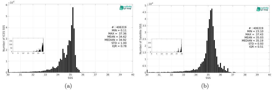
Figure 3: Histograms of SSS from ICES (a) and SMAP SSS L3 v5.3 - Monthly (RSS) (b) considering all match-up pairs per bins of 0.1 over the Atlantic Ocean Pi-MEP region and for the full satellite product period.
