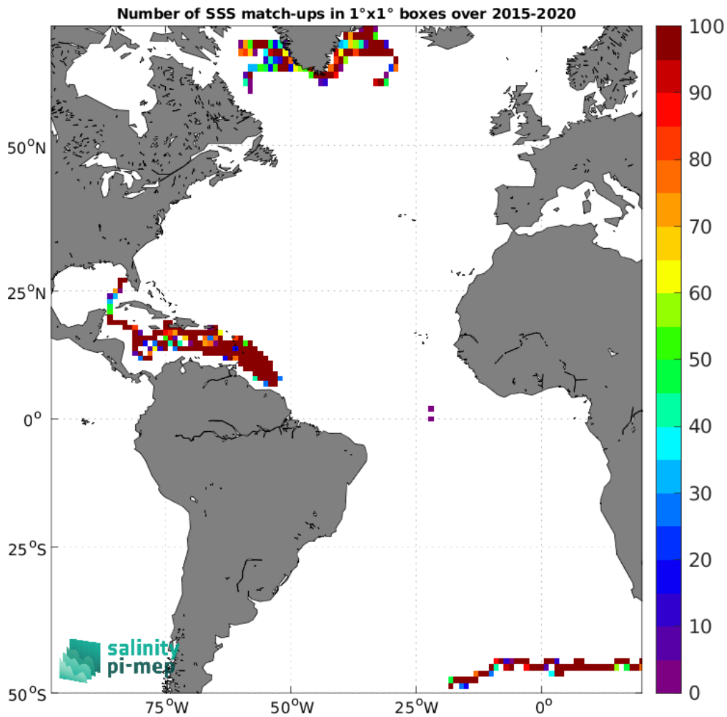
Figure 4: Number of SSS match-ups between Surface drifters SSS and the SMAP SSS L3 v5.3 - Monthly (RSS) SSS product for the Atlantic Ocean Pi-MEP region over 1^{\circ} \times 1^{\circ} boxes and for the full satellite product period.
