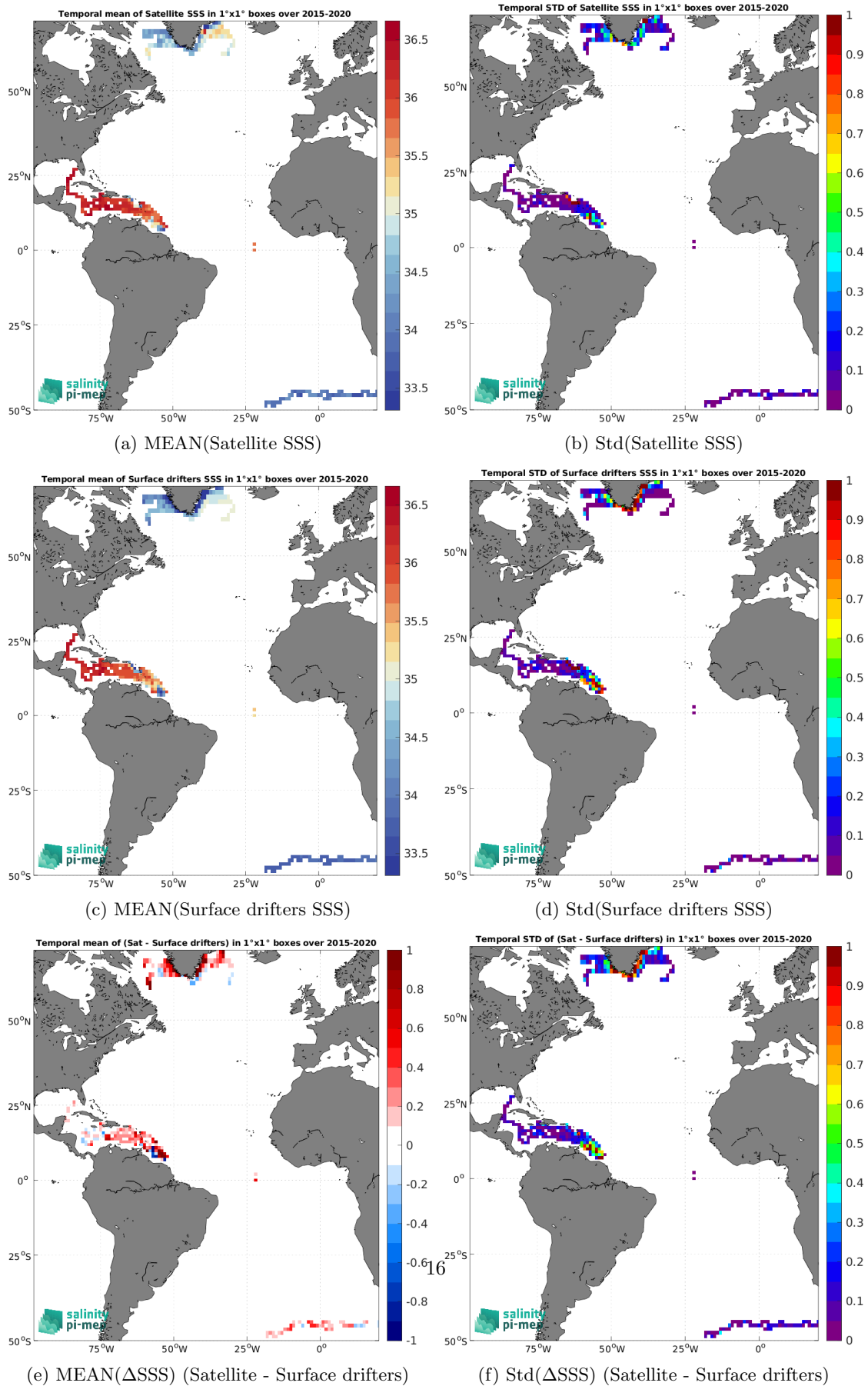
Figure 6: Temporal mean (left) and Std (right) of SSS from SMAP SSS L3 v5.3 - Monthly (RSS) (top), Surface drifters (middle), and of \Delta SSS (Satellite - Surface drifters). Only match-up pairs are used to generate these maps.
