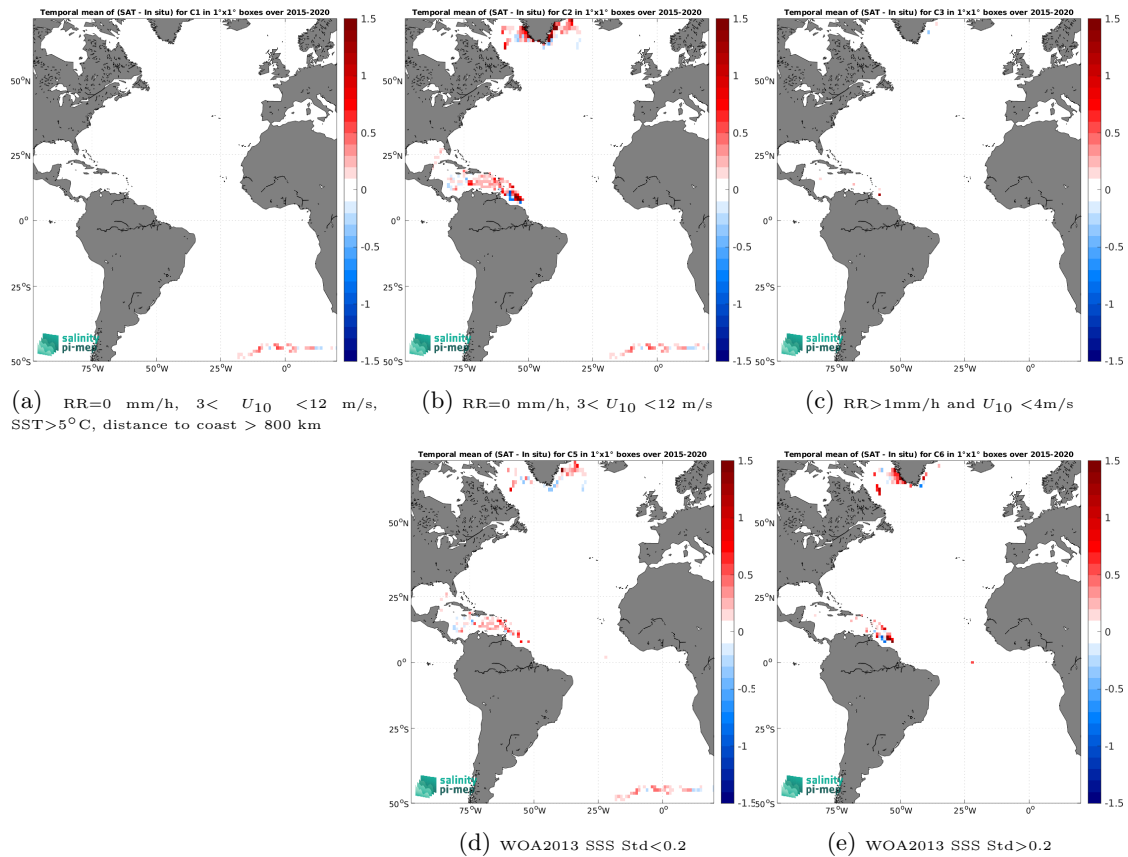
Figure 13: Temporal mean gridded over spatial boxes of size 1^\circ \times 1^\circ of \Delta SSS (SMAP SSS L3 v5.3 - Monthly (RSS) - Surface drifters) for 5 different subdatasets corresponding to:RR=0 mm/h, 3 < U_{10} < 12 m/s, SST >5^\circ\text{C} , distance to coast > 800 km (a), RR=0 mm/h, 3 < U_{10} < 12 m/s (b), RR >1 mm/h and U_{10} < 4 m/s (c), WOA2013 SSS Std <0.2 (d), WOA2013 SSS Std >0.2 (e).
