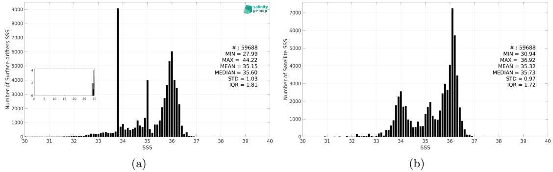
Figure 3: Histograms of SSS from Surface drifters (a) and SMAP SSS L3 v5.3 - Monthly (RSS) (b) considering all match-up pairs per bins of 0.1 over the Atlantic Ocean Pi-MEP region and for the full satellite product period.
