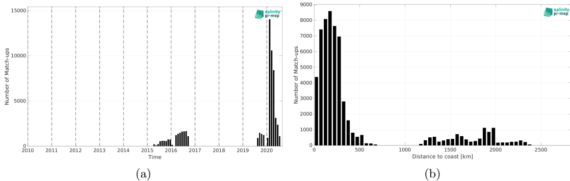
Figure 2: Number of match-ups between Surface drifters and SMAP SSS L3 v5.3 - Monthly (RSS) SSS as a function of time (a) and as function of the distance to coast (b) over the Atlantic Ocean Pi-MEP region and for the full satellite product period.
