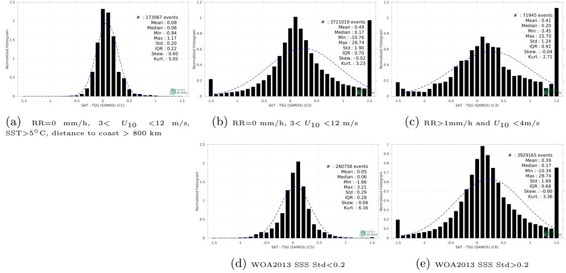
Figure 13: Normalized histogram of \Delta SSS (SMAP SSS L3 v5 - 8-Day running (RSS) - TSG (SAMOS)) for 5 different subdatasets corresponding to: RR=0 mm/h, 3 < U_{10} < 12 m/s, SST>5°C, distance to coast > 800 km (a), RR=0 mm/h, 3 < U_{10} < 12 m/s (b), RR>1mm/h and U_{10} < 4 m/s (c), WOA2013 SSS Std<0.2 (d), WOA2013 SSS Std>0.2 (e).
