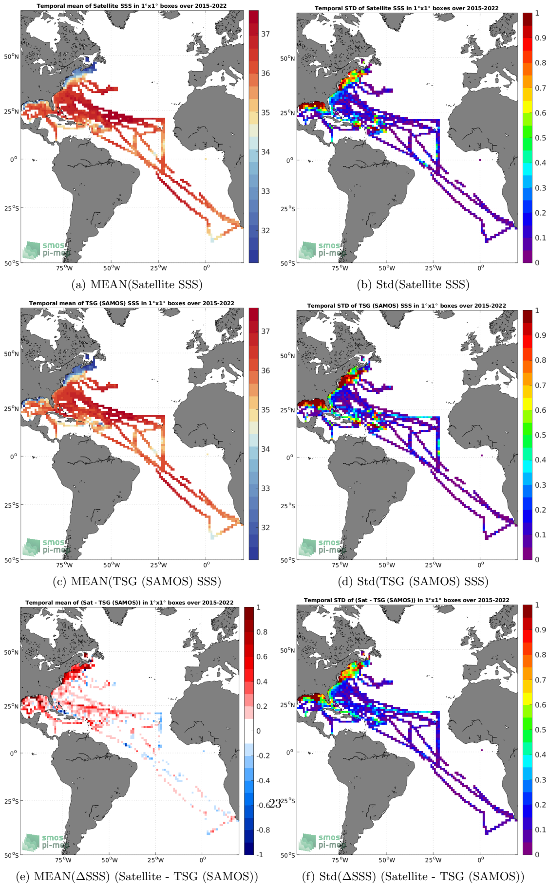
Figure 6: Temporal mean (left) and Std (right) of SSS from SMAP SSS L3 v5 - 8-Day running (RSS) (top), TSG (SAMOS) (middle), and of \Delta SSS (Satellite - TSG (SAMOS)). Only match-up pairs are used to generate these maps.
