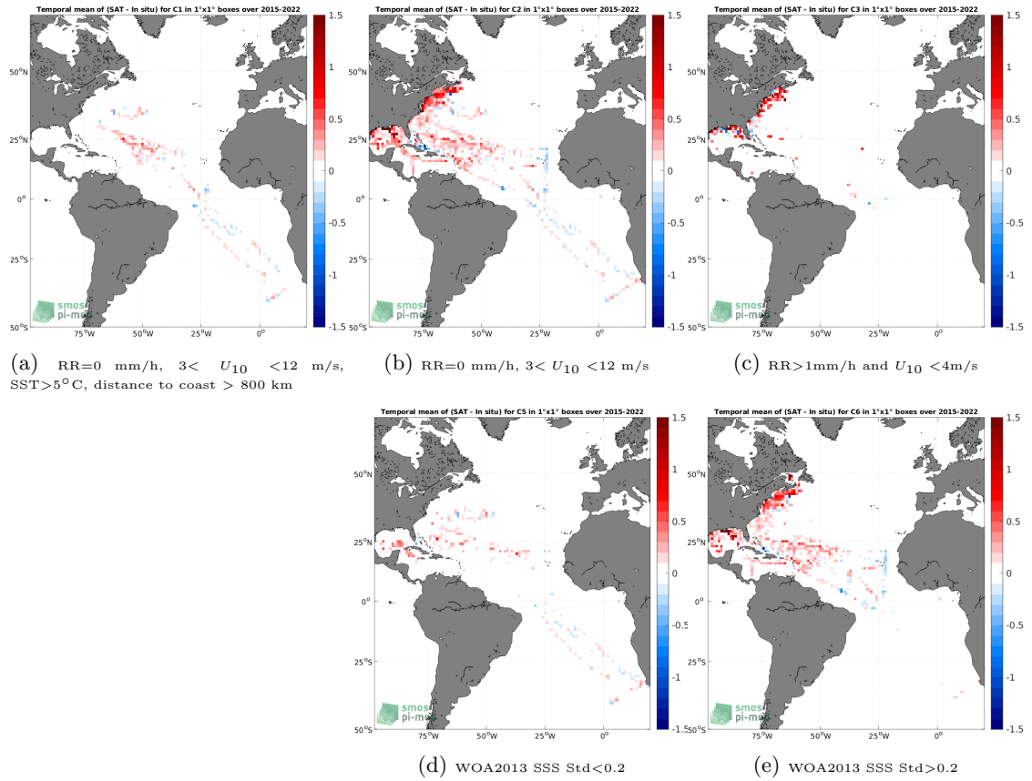
Figure 12: Temporal mean gridded over spatial boxes of size 1^\circ \times 1^\circ of \Delta SSS (SMAP SSS L3 v5 - 8-Day running (RSS) - TSG (SAMOS)) for 5 different subdatasets corresponding to:RR=0 mm/h, 3 < U_{10} < 12 m/s, SST >5^\circ\text{C} , distance to coast > 800 km (a), RR=0 mm/h, 3 < U_{10} < 12 m/s (b), RR >1 mm/h and U_{10} < 4 m/s (c), WOA2013 SSS Std <0.2 (d), WOA2013 SSS Std >0.2 (e).
