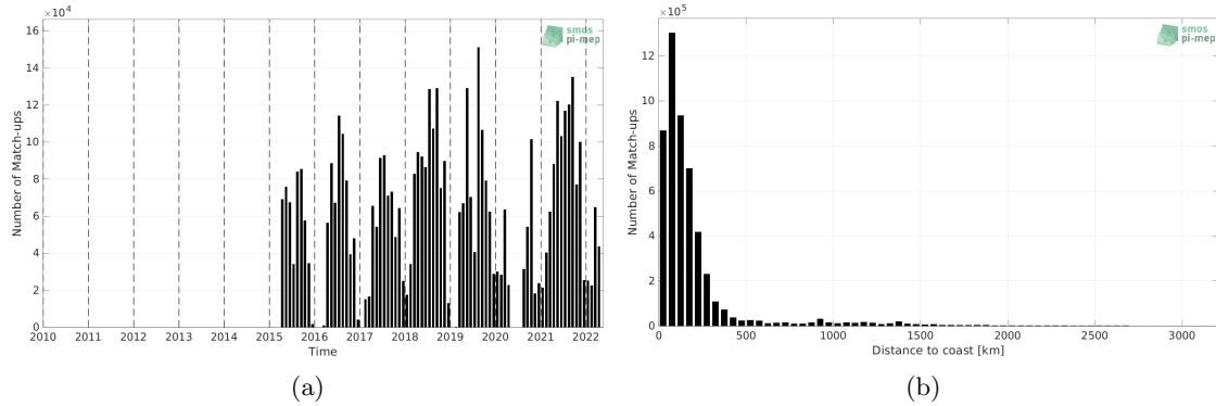
Figure 1: Number of match-ups between TSG (SAMOS) and SMAP SSS L3 v5 - 8-Day running (RSS) SSS as a function of time (a) and as function of the distance to coast (b) over the Atlantic Ocean Pi-MEP region and for the full satellite product period.
