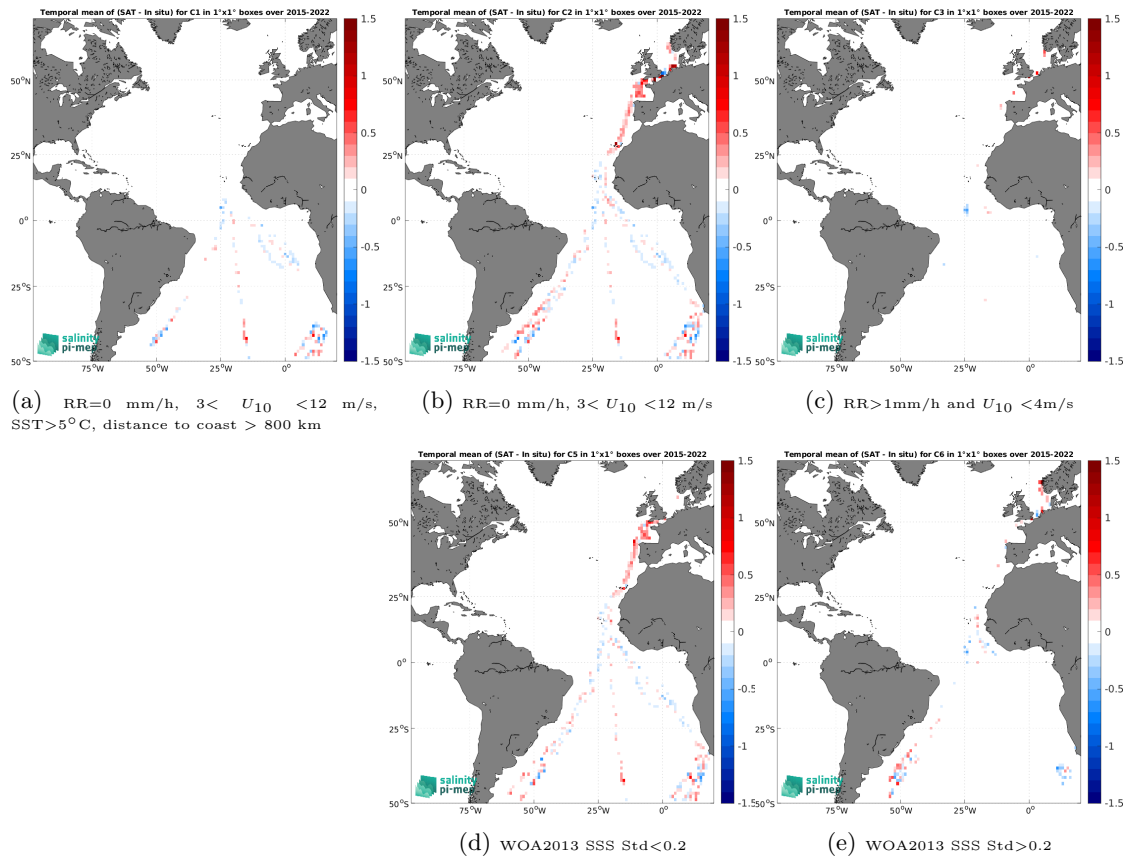
Figure 12: Temporal mean gridded over spatial boxes of size 1^\circ \times 1^\circ of \Delta\text{SSS} (SMAP SSS L3 v5 - 8-Day running (RSS) - TSG (Polarstern)) for 5 different subdatasets corresponding to:RR=0 mm/h, 3 < U_{10} < 12 m/s, SST >5^\circ\text{C} , distance to coast > 800 km (a), RR=0 mm/h, 3 < U_{10} < 12 m/s (b), RR >1 mm/h and U_{10} < 4 m/s (c), WOA2013 SSS Std <0.2 (d), WOA2013 SSS Std >0.2 (e).
