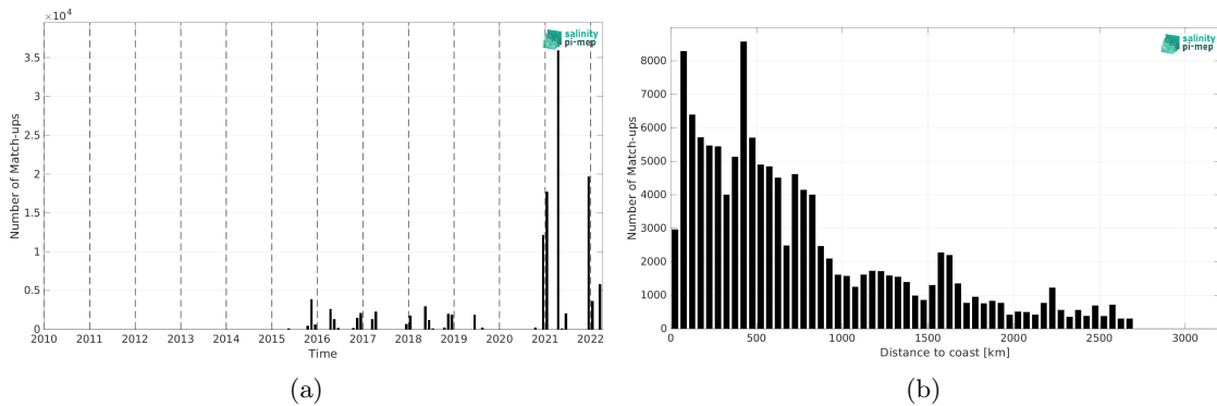
Figure 1: Number of match-ups between TSG (Polarstern) and SMAP SSS L3 v5 - 8-Day running (RSS) SSS as a function of time (a) and as function of the distance to coast (b) over the Atlantic Ocean Pi-MEP region and for the full satellite product period.
