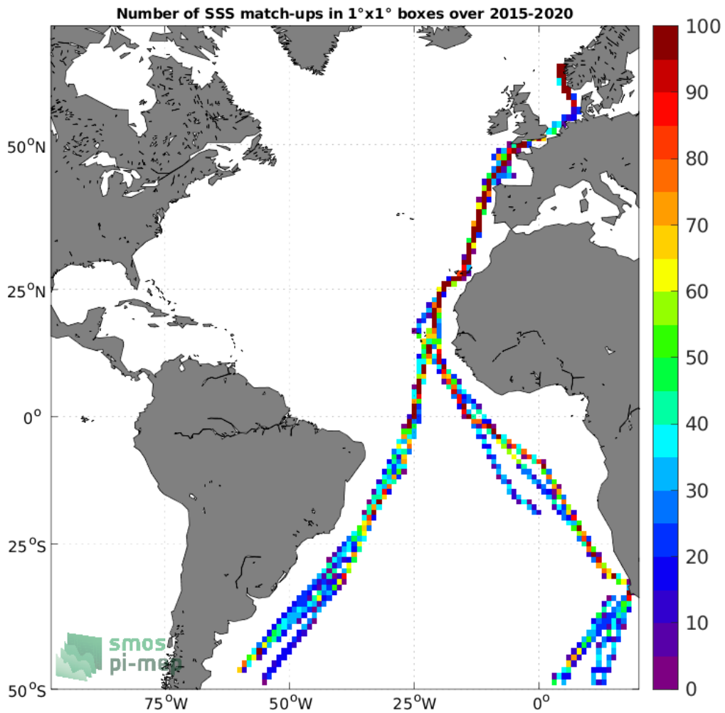
Figure 4: Number of SSS match-ups between TSG (Polarstern) SSS and the SMAP SSS L3 v5 - 8-Day running (RSS) SSS product for the Atlantic Ocean Pi-MEP region over 1°x1° boxes and for the full satellite product period.
