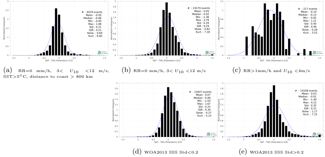
Figure 13: Normalized histogram of \Delta\text{SSS} (SMAP SSS L3 v5 - 8-Day running (RSS) - TSG (Polarstern)) for 5 different subdatasets corresponding to: RR=0 mm/h, 3 < U_{10} < 12 m/s, SST>5°C, distance to coast > 800 km (a), RR=0 mm/h, 3 < U_{10} < 12 m/s (b), RR>1mm/h and U_{10} < 4 m/s (c), WOA2013 SSS Std<0.2 (d), WOA2013 SSS Std>0.2 (e).
