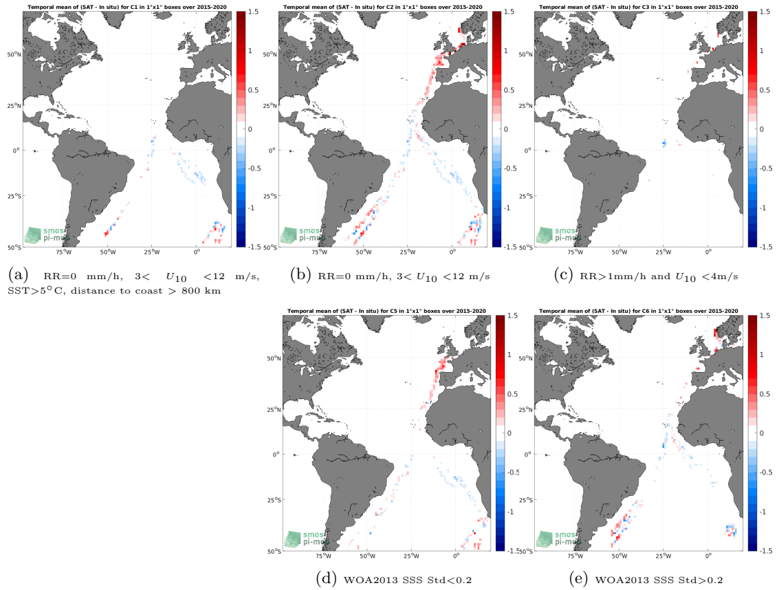
Figure 12: Temporal mean gridded over spatial boxes of size 1^\circ \times 1^\circ of \Delta\text{SSS} (SMAP SSS L3 v5 - 8-Day running (RSS) - TSG (Polarstern)) for 5 different subdatasets corresponding to:RR=0 mm/h, 3 < U_{10} < 12 m/s, SST >5^\circ\text{C} , distance to coast > 800 km (a), RR=0 mm/h, 3 < U_{10} < 12 m/s (b), RR >1 mm/h and U_{10} < 4 m/s (c), WOA2013 SSS Std <0.2 (d), WOA2013 SSS Std >0.2 (e).
