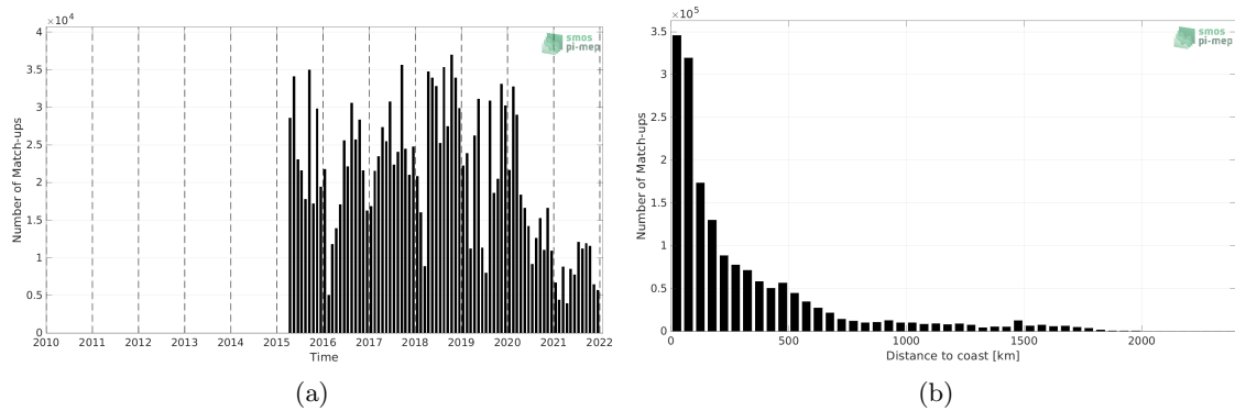
Figure 1: Number of match-ups between TSG (LEGOS-DM) and SMAP SSS L3 v5 - 8-Day running (RSS) SSS as a function of time (a) and as function of the distance to coast (b) over the Atlantic Ocean Pi-MEP region and for the full satellite product period.
