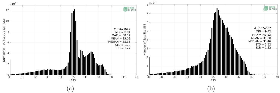
Figure 2: Histograms of SSS from TSG (LEGOS-DM) (a) and SMAP SSS L3 v5 - 8-Day running (RSS) (b) considering all match-up pairs per bins of 0.1 over the Atlantic Ocean Pi-MEP region and for the full satellite product period.
