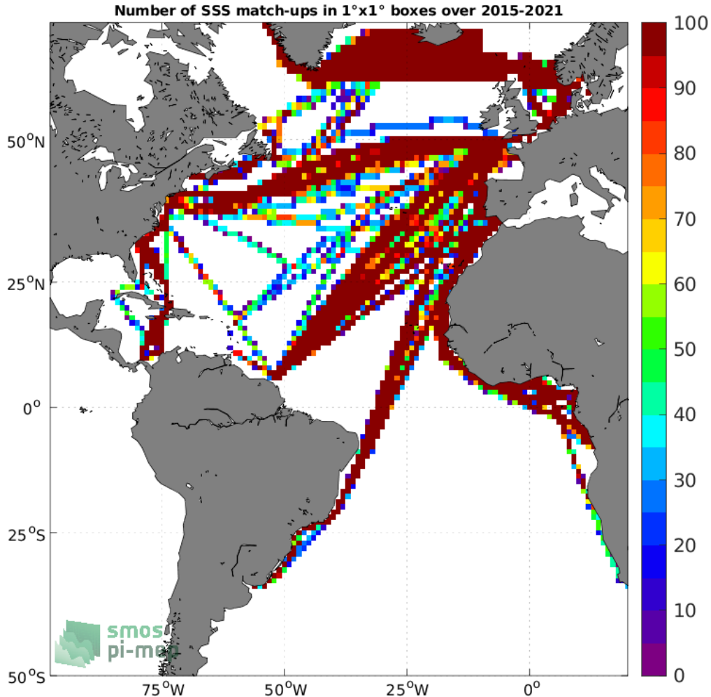
Figure 4: Number of SSS match-ups between TSG (LEGOS-DM) SSS and the SMAP SSS L3 v5 - 8-Day running (RSS) SSS product for the Atlantic Ocean Pi-MEP region over 1^\circ \times 1^\circ boxes and for the full satellite product period.
