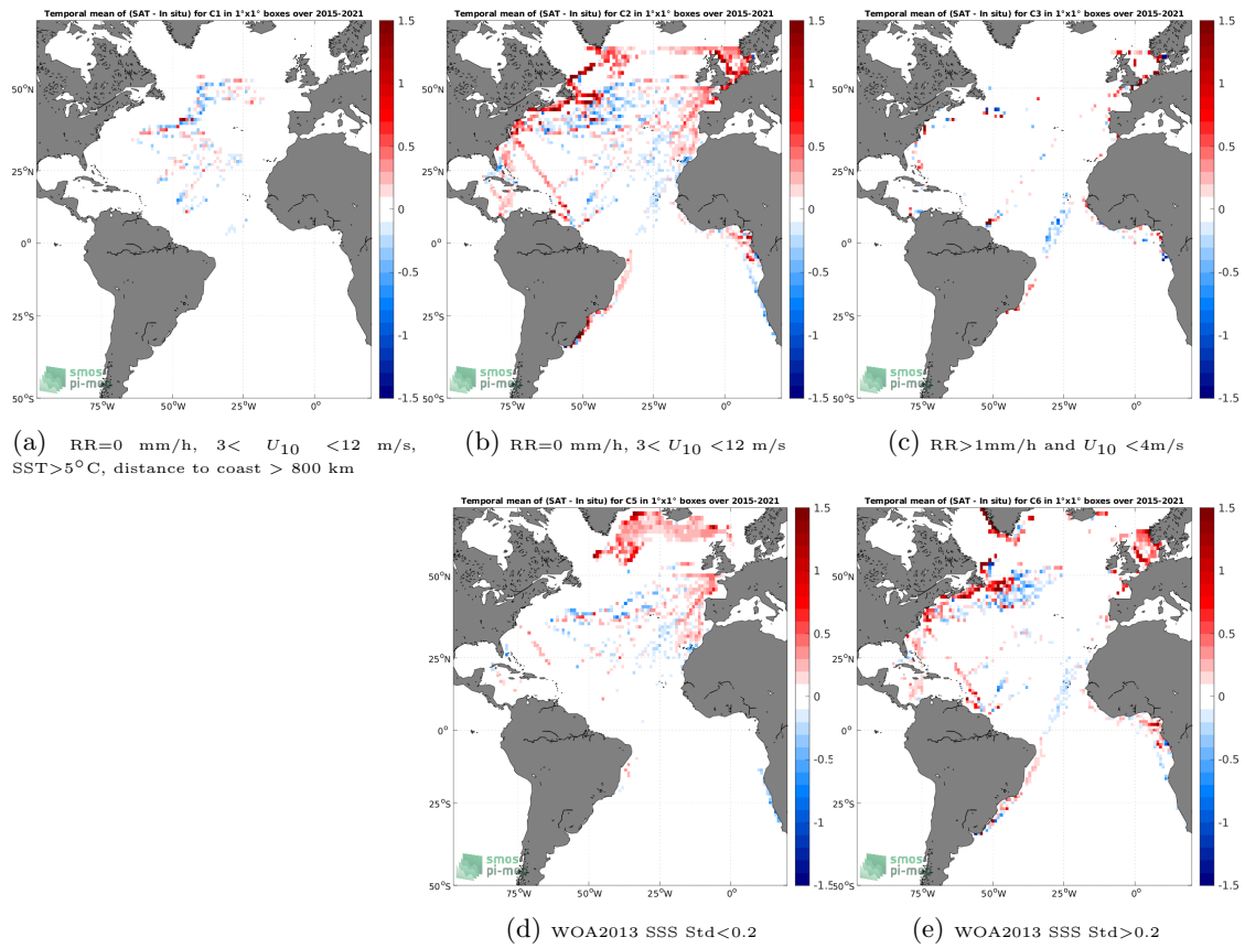
Figure 12: Temporal mean gridded over spatial boxes of size 1^\circ \times 1^\circ of \Delta SSS (SMAP SSS L3 v5 - 8-Day running (RSS) - TSG (LEGOS-DM)) for 5 different subdatasets corresponding to:RR=0 mm/h, 3 < U_{10} < 12 m/s, SST >5^\circ\text{C} , distance to coast > 800 km (a), RR=0 mm/h, 3 < U_{10} < 12 m/s (b), RR >1 mm/h and U_{10} < 4 m/s (c), WOA2013 SSS Std <0.2 (d), WOA2013 SSS Std >0.2 (e).
