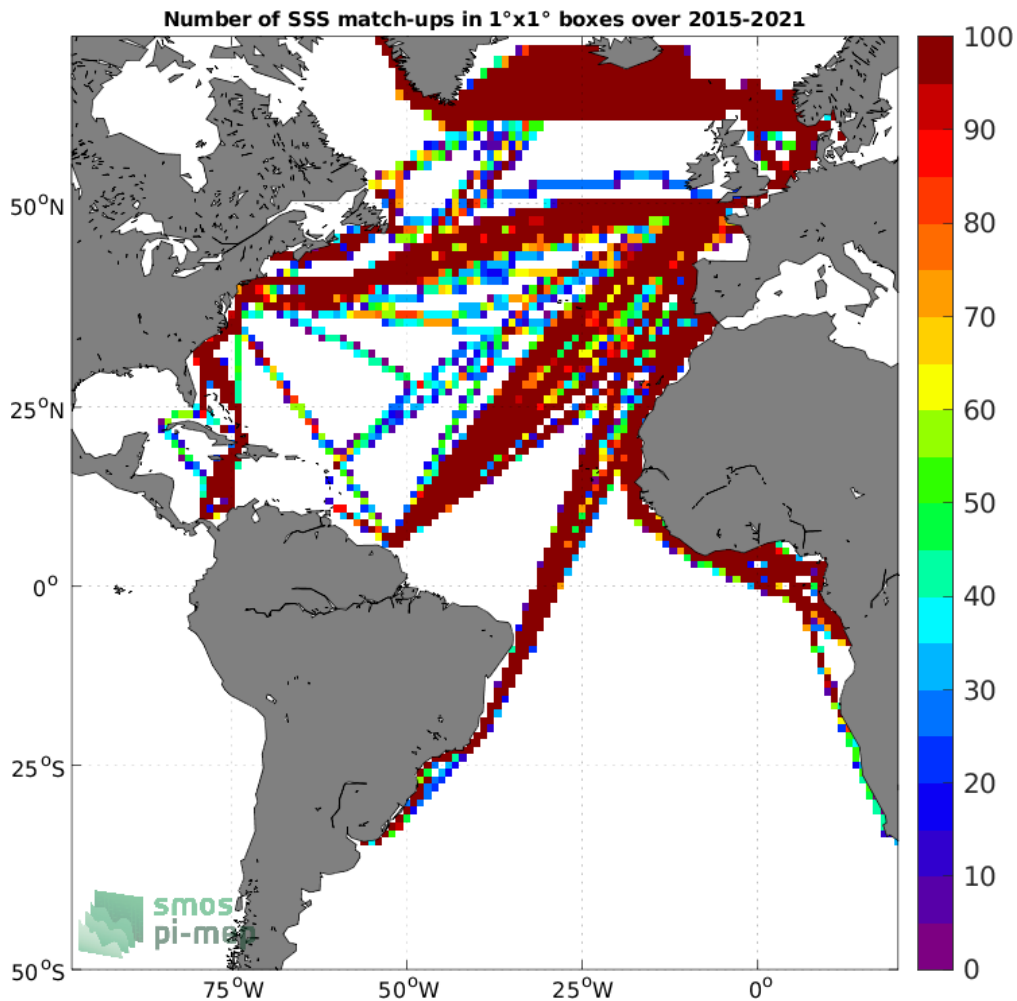
Figure 4: Number of SSS match-ups between TSG (LEGOS-DM) SSS and the SMAP SSS L3 v5 - 8-Day running (RSS) SSS product for the Atlantic Ocean Pi-MEP region over 1°x1° boxes and for the full satellite product period.
