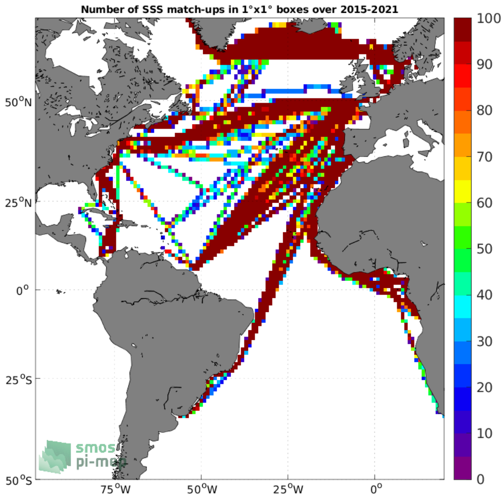
Figure 4: Number of SSS match-ups between TSG (LEGOS-DM) SSS and the SMAP SSS L3 v5 - 8-Day running (RSS) SSS product for the Atlantic Ocean Pi-MEP region over 1°×1° boxes and for the full satellite product period.
