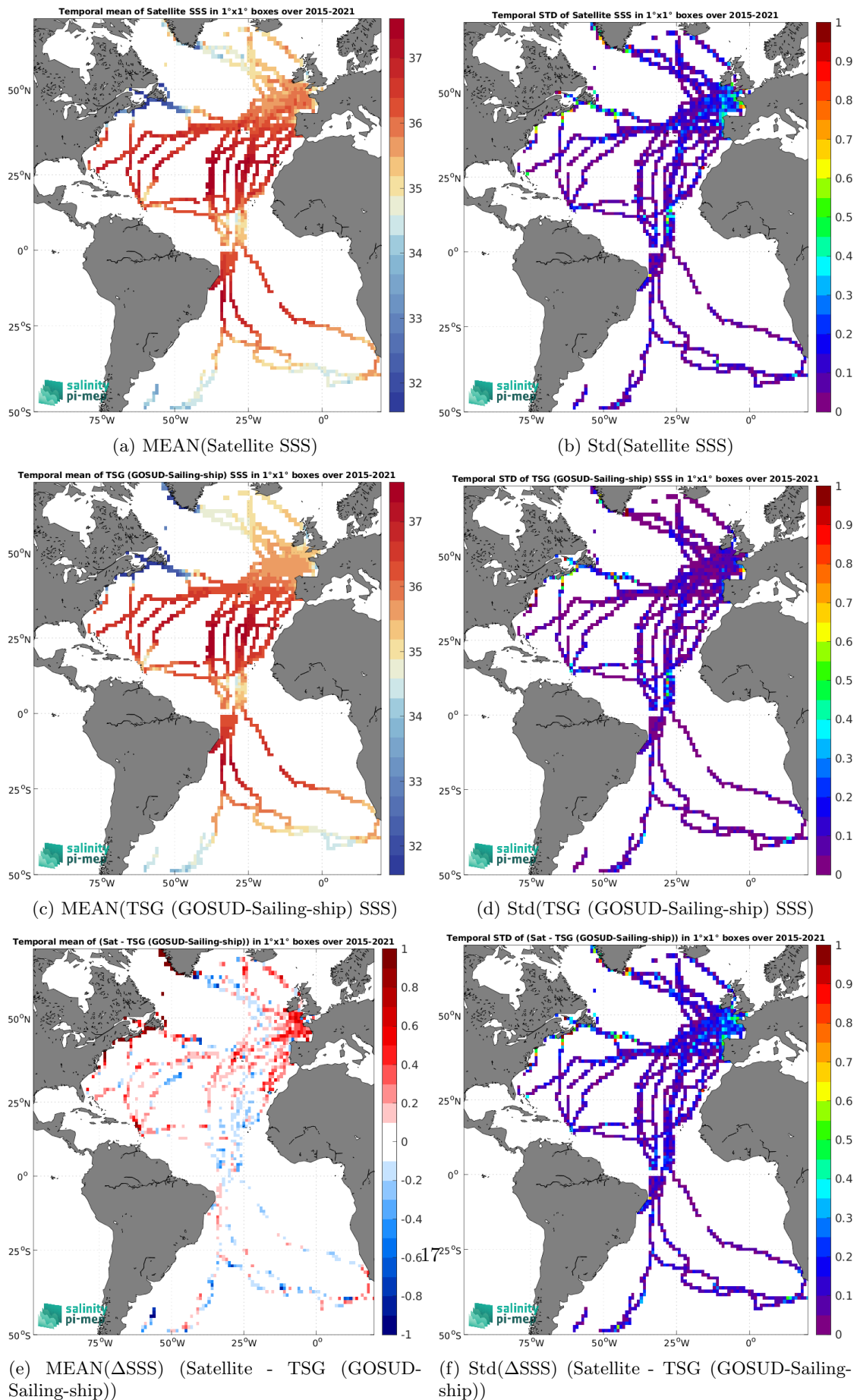
Figure 6: Temporal mean (left) and Std (right) of SSS from SMAP SSS L3 v5 - 8-Day running (RSS) (top), TSG (GOSUD-Sailing-ship) (middle), and of \Delta\text{SSS} (Satellite - TSG (GOSUD-Sailing-ship)). Only match-up pairs are used to generate these maps.
