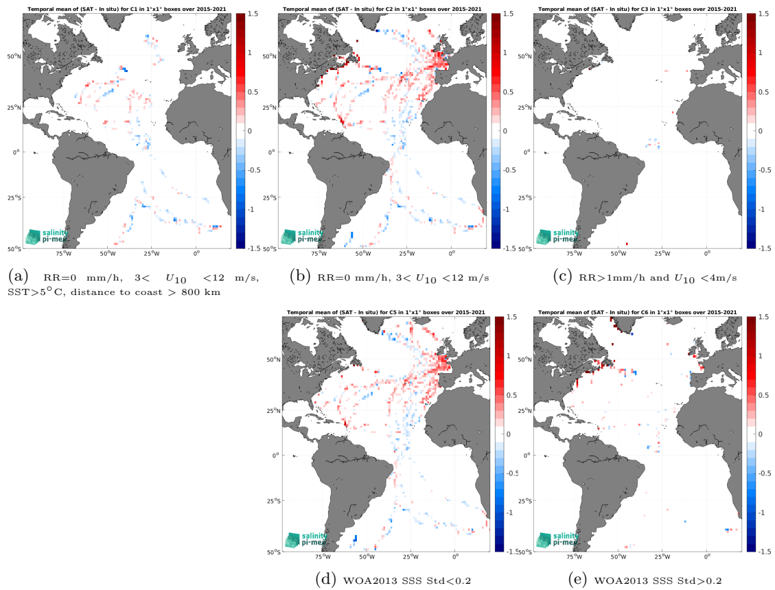
Figure 12: Temporal mean gridded over spatial boxes of size 1^\circ \times 1^\circ of \Delta\text{SSS} (SMAP SSS L3 v5 - 8-Day running (RSS) - TSG (GOSUD-Sailing-ship)) for 5 different subdatasets corresponding to:RR=0 mm/h, 3 < U_{10} < 12 m/s, SST >5^\circ\text{C} , distance to coast > 800 km (a), RR=0 mm/h, 3 < U_{10} < 12 m/s (b), RR >1 mm/h and U_{10} < 4 m/s (c), WOA2013 SSS Std <0.2 (d), WOA2013 SSS Std >0.2 (e).
