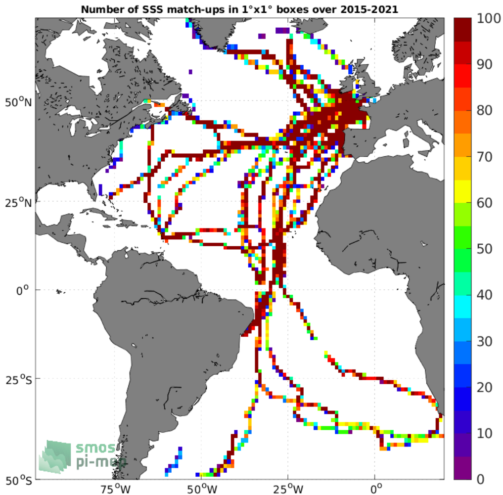
Figure 4: Number of SSS match-ups between TSG (GOSUD-Sailing-ship) SSS and the SMAP SSS L3 v5 - 8-Day running (RSS) SSS product for the Atlantic Ocean Pi-MEP region over 1^\circ \times 1^\circ boxes and for the full satellite product period.
