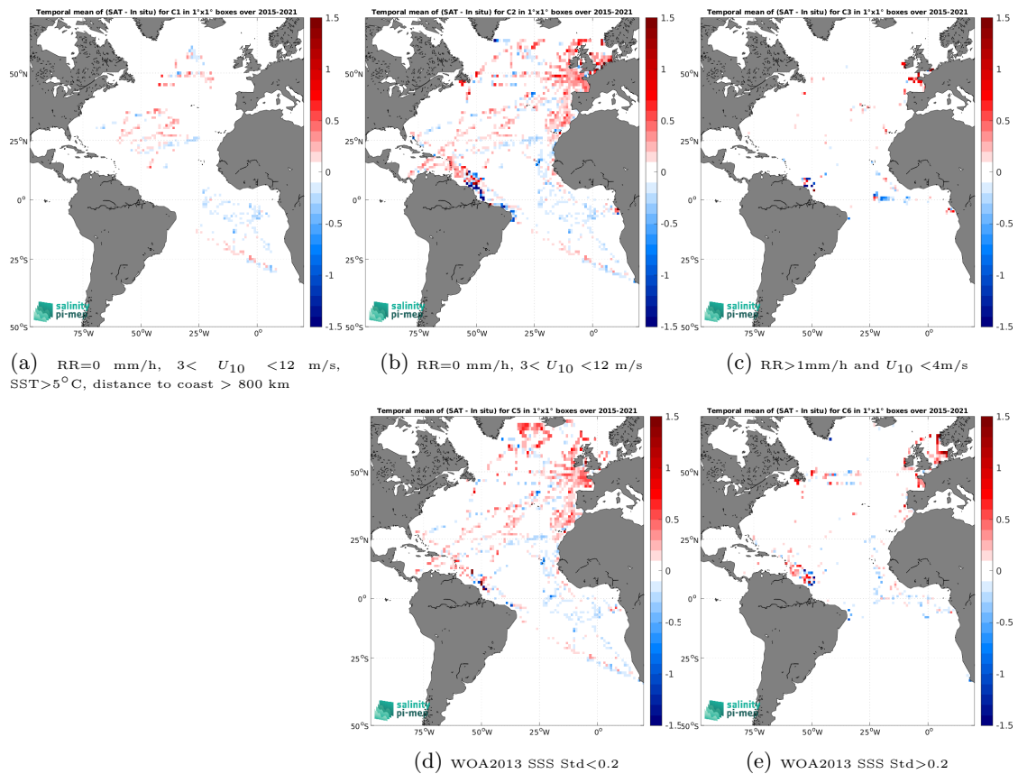
Figure 12: Temporal mean gridded over spatial boxes of size 1^\circ \times 1^\circ of \Delta\text{SSS} (SMAP SSS L3 v5 - 8-Day running (RSS) - TSG (GOSUD-Research-vessel)) for 5 different subdatasets corresponding to:RR=0 mm/h, 3 < U_{10} < 12 m/s, SST >5^\circ\text{C} , distance to coast > 800 km (a), RR=0 mm/h, 3 < U_{10} < 12 m/s (b), RR >1 mm/h and U_{10} < 4 m/s (c), WOA2013 SSS Std <0.2 (d), WOA2013 SSS Std >0.2 (e).
