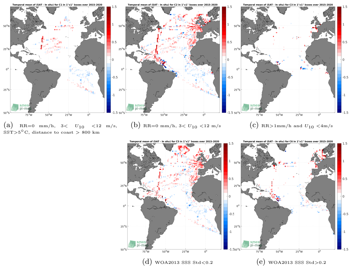
Figure 12: Temporal mean gridded over spatial boxes of size 1^\circ \times 1^\circ of \Delta SSS (SMAP SSS L3 v5 - 8-Day running (RSS) - TSG (GOSUD-Research-vessel)) for 5 different subdatasets corresponding to:RR=0 mm/h, 3 < U_{10} < 12 m/s, SST>5°C, distance to coast > 800 km (a), RR=0 mm/h, 3 < U_{10} < 12 m/s (b), RR>1mm/h and U_{10} < 4 m/s (c), WOA2013 SSS Std<0.2 (d), WOA2013 SSS Std>0.2 (e).
