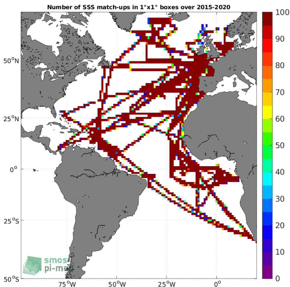
Figure 4: Number of SSS match-ups between TSG (GOSUD-Research-vessel) SSS and the SMAP SSS L3 v5 - 8-Day running (RSS) SSS product for the Atlantic Ocean Pi-MEP region over 1°x1° boxes and for the full satellite product period.
