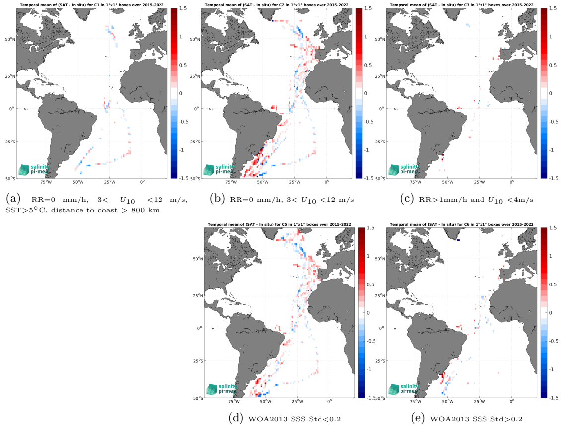
Figure 12: Temporal mean gridded over spatial boxes of size 1^\circ \times 1^\circ of \Delta SSS (SMAP SSS L3 v5 - 8-Day running (RSS) - TSG (CSIC-UTM)) for 5 different subdatasets corresponding to:RR=0 mm/h, 3 < U_{10} < 12 m/s, SST >5^\circ\text{C} , distance to coast > 800 km (a), RR=0 mm/h, 3 < U_{10} < 12 m/s (b), RR >1 mm/h and U_{10} < 4 m/s (c), WOA2013 SSS Std <0.2 (d), WOA2013 SSS Std >0.2 (e).
