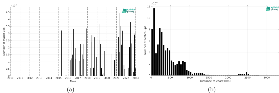
Figure 1: Number of match-ups between TSG (CSIC-UTM) and SMAP SSS L3 v5 - 8-Day running (RSS) SSS as a function of time (a) and as function of the distance to coast (b) over the Atlantic Ocean Pi-MEP region and for the full satellite product period.
