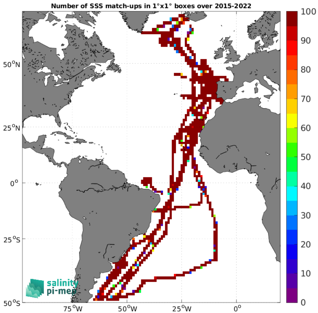
Figure 4: Number of SSS match-ups between TSG (CSIC-UTM) SSS and the SMAP SSS L3 v5 - 8-Day running (RSS) SSS product for the Atlantic Ocean Pi-MEP region over 1°×1° boxes and for the full satellite product period.
