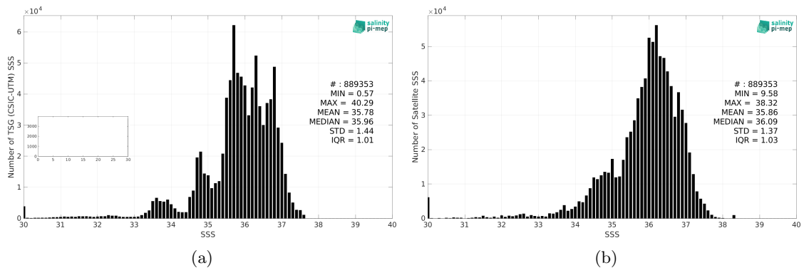
Figure 2: Histograms of SSS from TSG (CSIC-UTM) (a) and SMAP SSS L3 v5 - 8-Day running (RSS) (b) considering all match-up pairs per bins of 0.1 over the Atlantic Ocean Pi-MEP region and for the full satellite product period.
