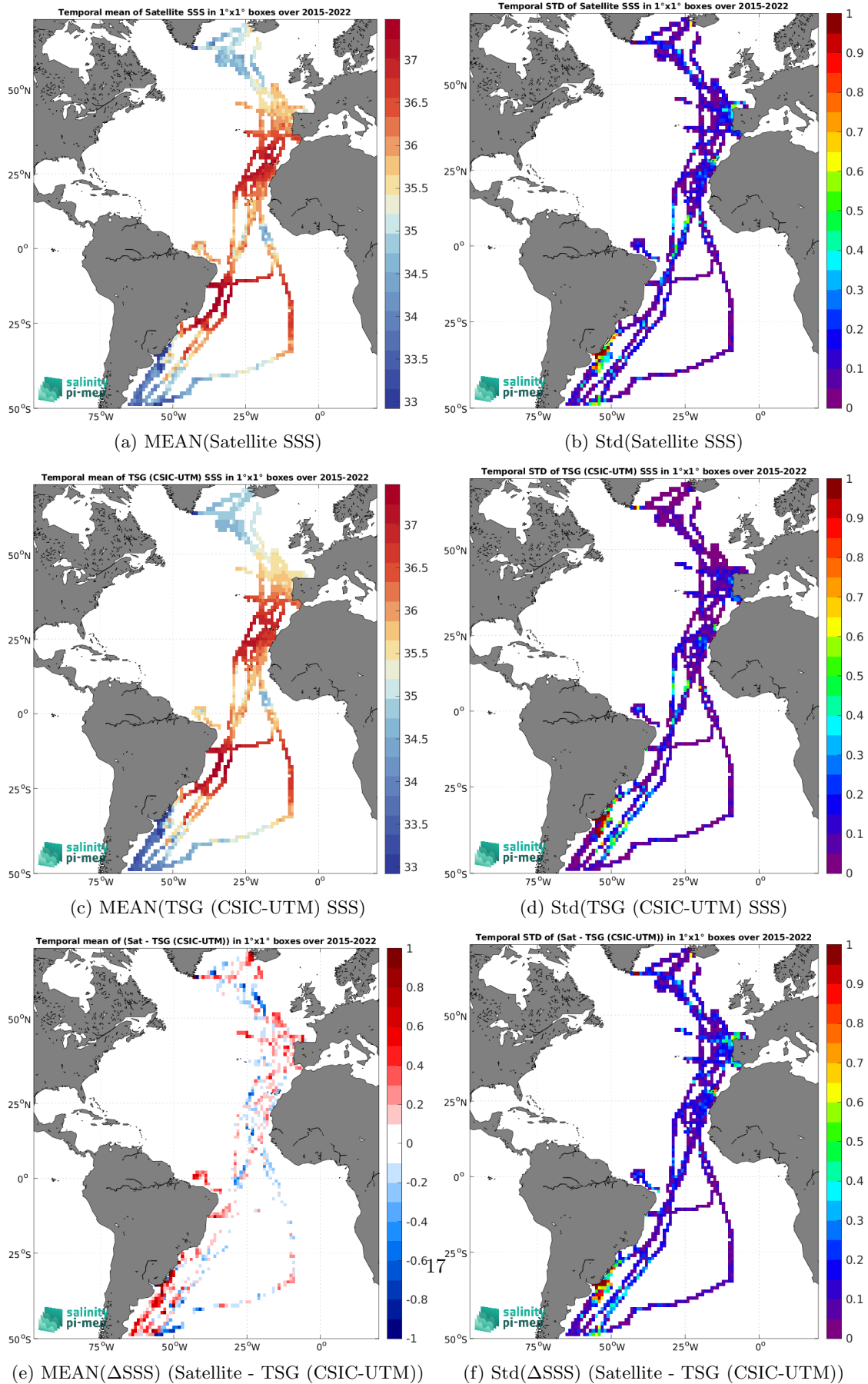
Figure 6: Temporal mean (left) and Std (right) of SSS from SMAP SSS L3 v5 - 8-Day running (RSS) (top), TSG (CSIC-UTM) (middle), and of \Delta SSS (Satellite - TSG (CSIC-UTM)). Only match-up pairs are used to generate these maps.
