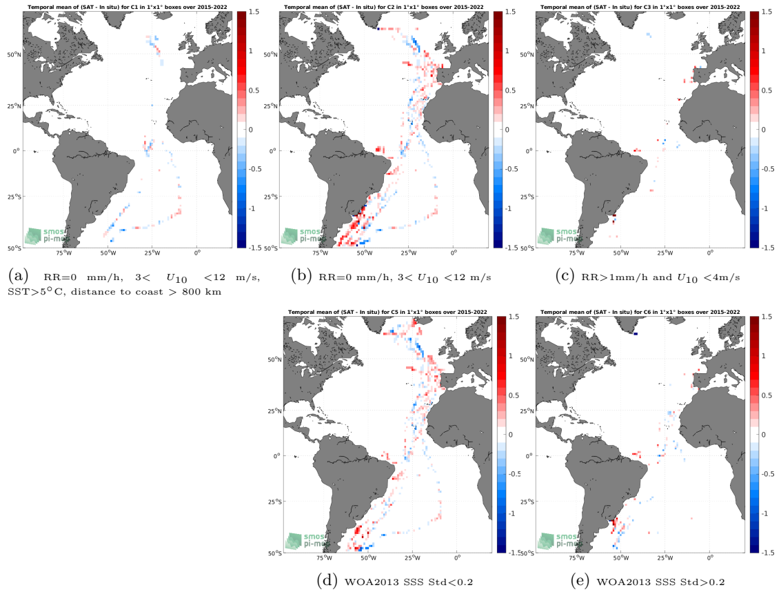
Figure 12: Temporal mean gridded over spatial boxes of size 1^\circ \times 1^\circ of \Delta SSS (SMAP SSS L3 v5 - 8-Day running (RSS) - TSG (CSIC-UTM)) for 5 different subdatasets corresponding to:RR=0 mm/h, 3 < U_{10} < 12 m/s, SST >5^\circ\text{C} , distance to coast > 800 km (a), RR=0 mm/h, 3 < U_{10} < 12 m/s (b), RR >1 mm/h and U_{10} < 4 m/s (c), WOA2013 SSS Std <0.2 (d), WOA2013 SSS Std >0.2 (e).
