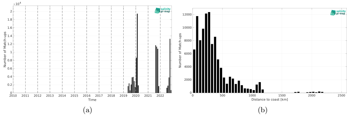
Figure 1: Number of match-ups between Saildrone and SMAP SSS L3 v5 - 8-Day running (RSS) SSS as a function of time (a) and as function of the distance to coast (b) over the Atlantic Ocean Pi-MEP region and for the full satellite product period.
