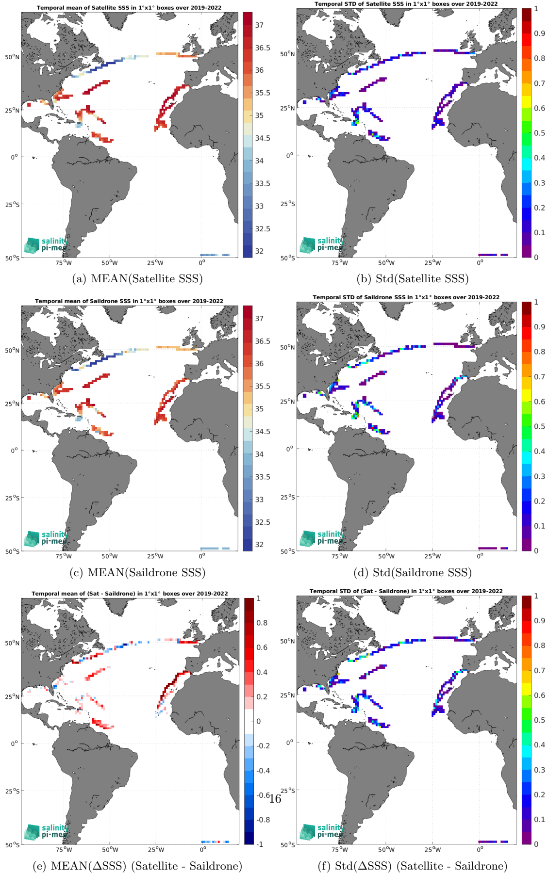
Figure 6: Temporal mean (left) and Std (right) of SSS from SMAP SSS L3 v5 - 8-Day running (RSS) (top), Saildrone (middle), and of \Delta SSS (Satellite - Saildrone). Only match-up pairs are used to generate these maps.
