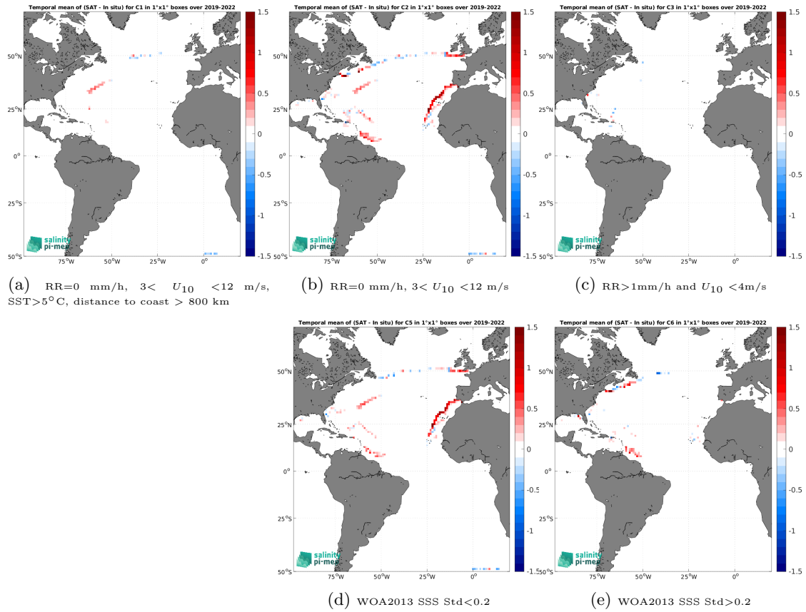
Figure 12: Temporal mean gridded over spatial boxes of size 1^\circ \times 1^\circ of \Delta\text{SSS} (SMAP SSS L3 v5 - 8-Day running (RSS) - Saildrone) for 5 different subdatasets corresponding to:RR=0 mm/h, 3 < U_{10} < 12 m/s, SST >5^\circ\text{C} , distance to coast > 800 km (a), RR=0 mm/h, 3 < U_{10} < 12 m/s (b), RR >1 mm/h and U_{10} < 4 m/s (c), WOA2013 SSS Std <0.2 (d), WOA2013 SSS Std >0.2 (e).
