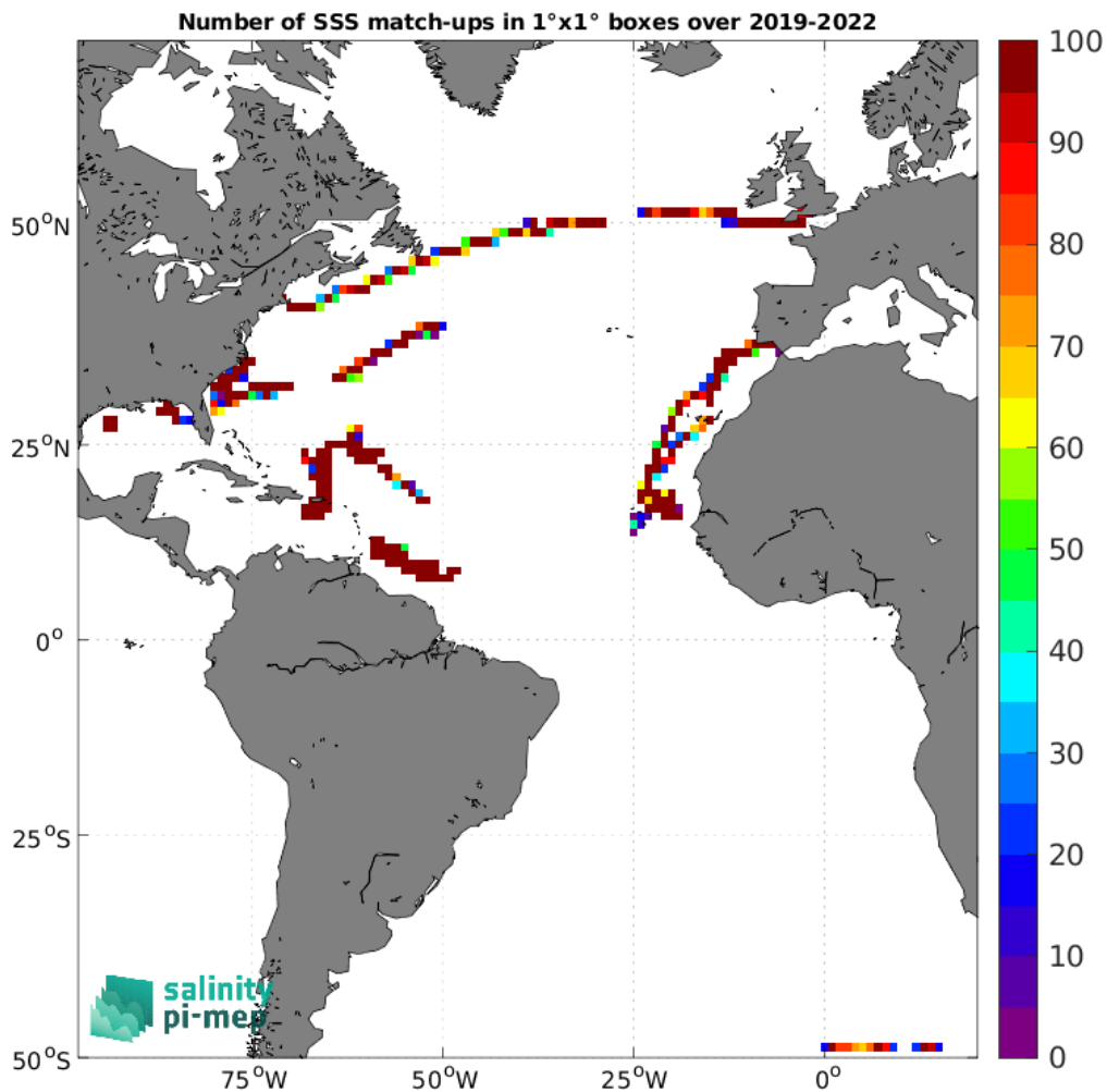
Figure 4: Number of SSS match-ups between Saildrone SSS and the SMAP SSS L3 v5 - 8-Day running (RSS) SSS product for the Atlantic Ocean Pi-MEP region over 1^\circ \times 1^\circ boxes and for the full satellite product period.
