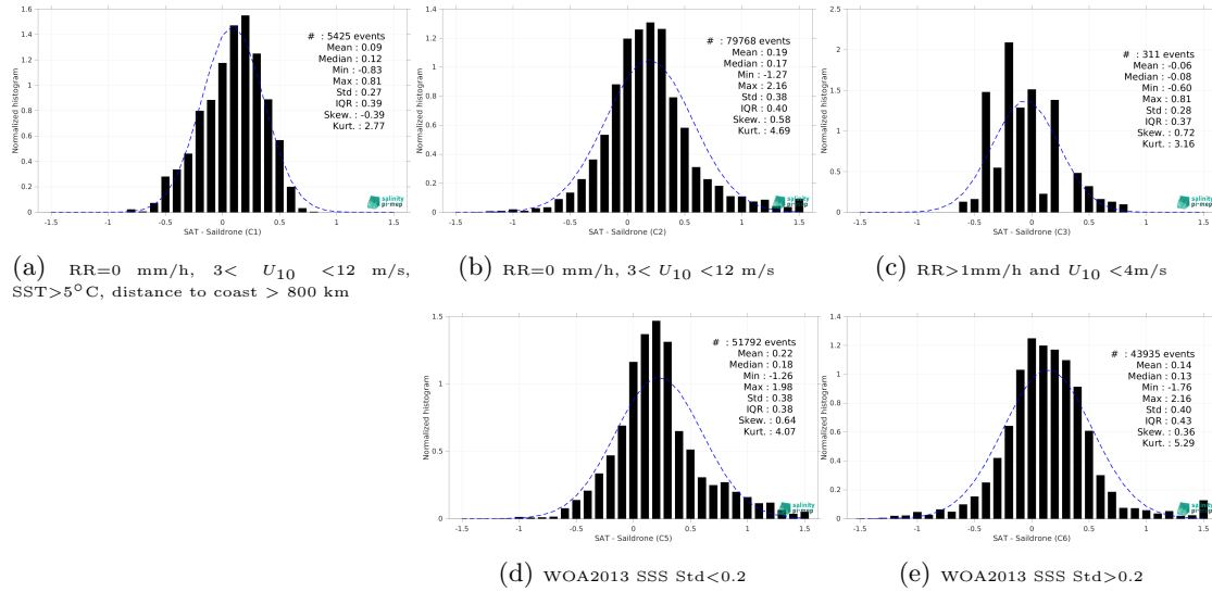
Figure 13: Normalized histogram of \Delta SSS (SMAP SSS L3 v5 - 8-Day running (RSS) - Sairdrone) for 5 different subdatasets corresponding to: RR=0 mm/h, 3 < U_{10} < 12 m/s, SST>5°C, distance to coast > 800 km (a), RR=0 mm/h, 3 < U_{10} < 12 m/s (b), RR>1mm/h and U_{10} < 4 m/s (c), WOA2013 SSS Std<0.2 (d), WOA2013 SSS Std>0.2 (e).
