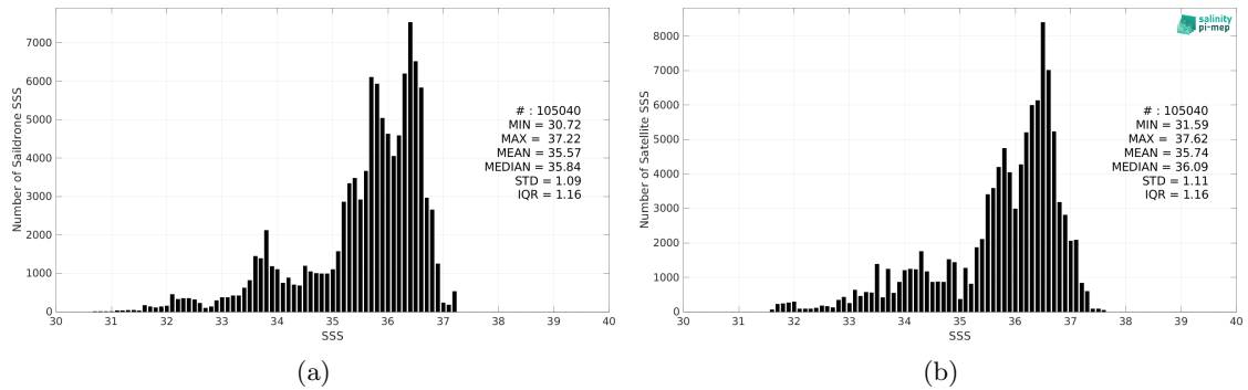
Figure 2: Histograms of SSS from Saildrone (a) and SMAP SSS L3 v5 - 8-Day running (RSS) (b) considering all match-up pairs per bins of 0.1 over the Atlantic Ocean Pi-MEP region and for the full satellite product period.
