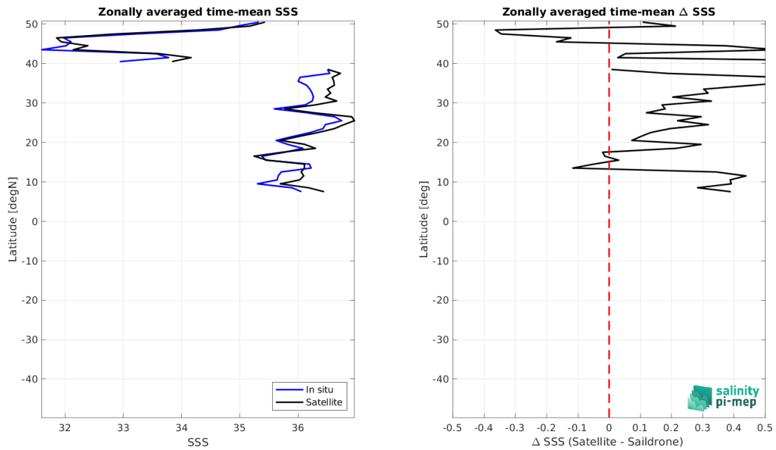
Figure 8: Left panel: Zonal mean SSS from SMAP SSS L3 v5 - 8-Day running (RSS) satellite product (black) and from Saikdrone (blue). Right panel: Zonal mean of \Delta SSS (Satellite - Saikdrone) for all the collected Pi-MEP match-up pairs estimated over the full satellite product period.
