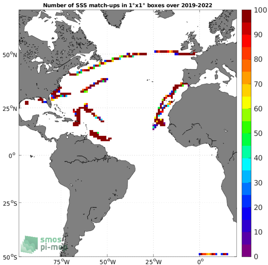
Figure 4: Number of SSS match-ups between Sairdrone SSS and the SMAP SSS L3 v5 - 8-Day running (RSS) SSS product for the Atlantic Ocean Pi-MEP region over 1^\circ \times 1^\circ boxes and for the full satellite product period.
