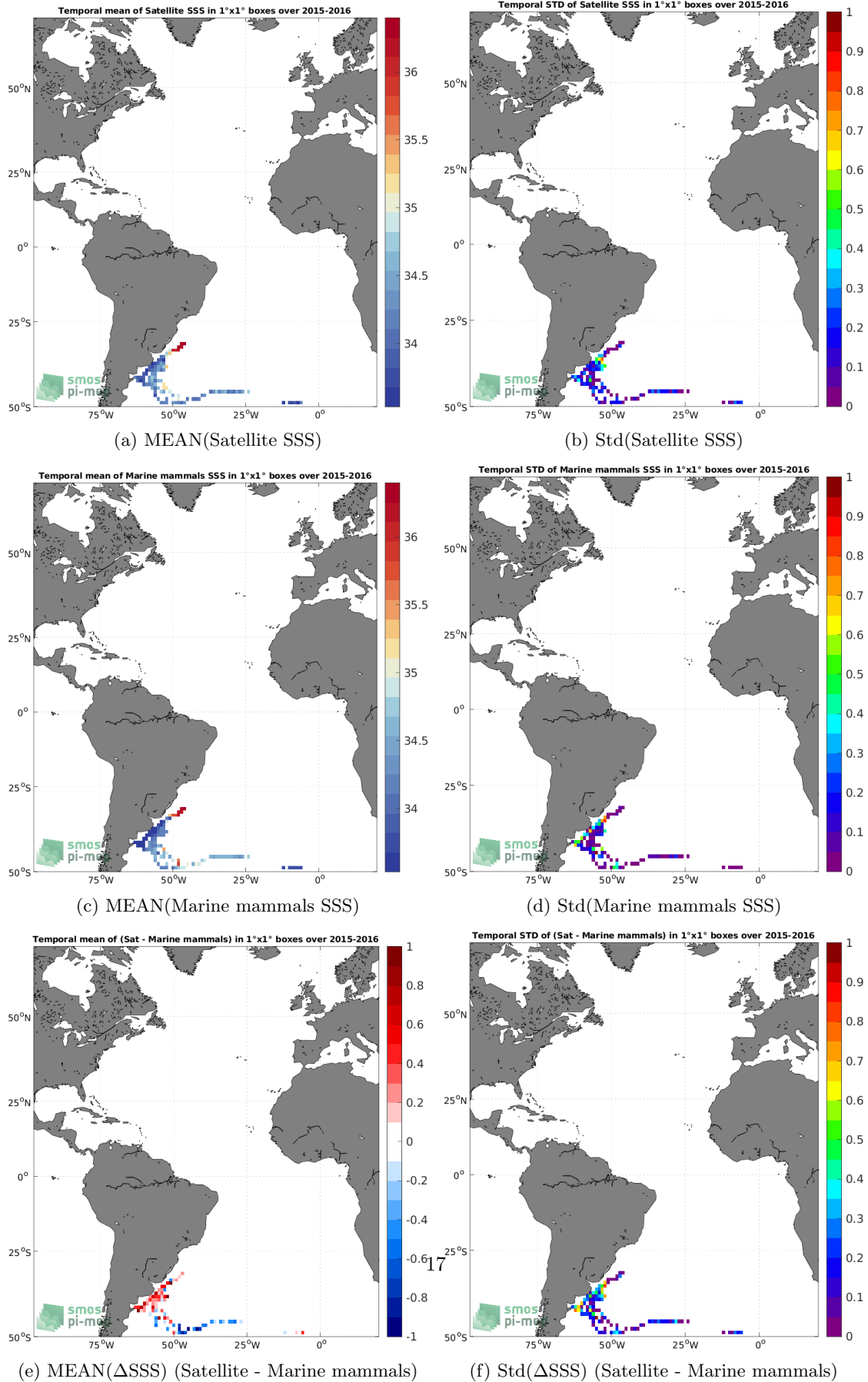
Figure 6: Temporal mean (left) and Std (right) of SSS from SMAP SSS L3 v5 - 8-Day running (RSS) (top), Marine mammals (middle), and of \Delta SSS (Satellite - Marine mammals). Only match-up pairs are used to generate these maps.
