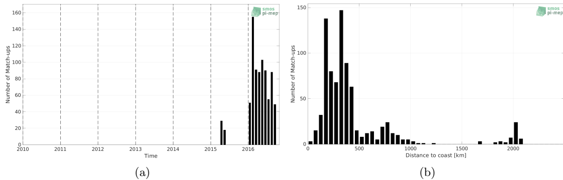
Figure 1: Number of match-ups between Marine mammals and SMAP SSS L3 v5 - 8-Day running (RSS) SSS as a function of time (a) and as function of the distance to coast (b) over the Atlantic Ocean Pi-MEP region and for the full satellite product period.
