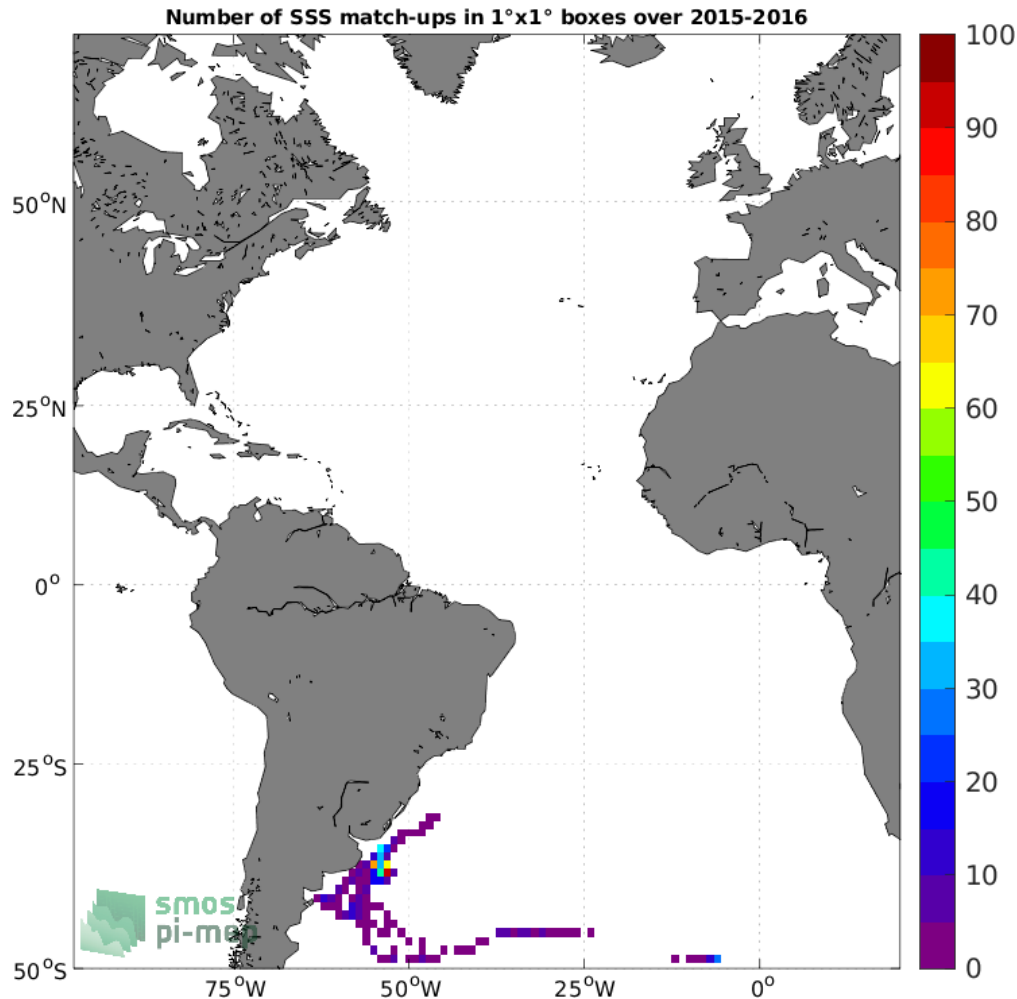
Figure 4: Number of SSS match-ups between Marine mammals SSS and the SMAP SSS L3 v5 - 8-Day running (RSS) SSS product for the Atlantic Ocean Pi-MEP region over 1^\circ \times 1^\circ boxes and for the full satellite product period.
