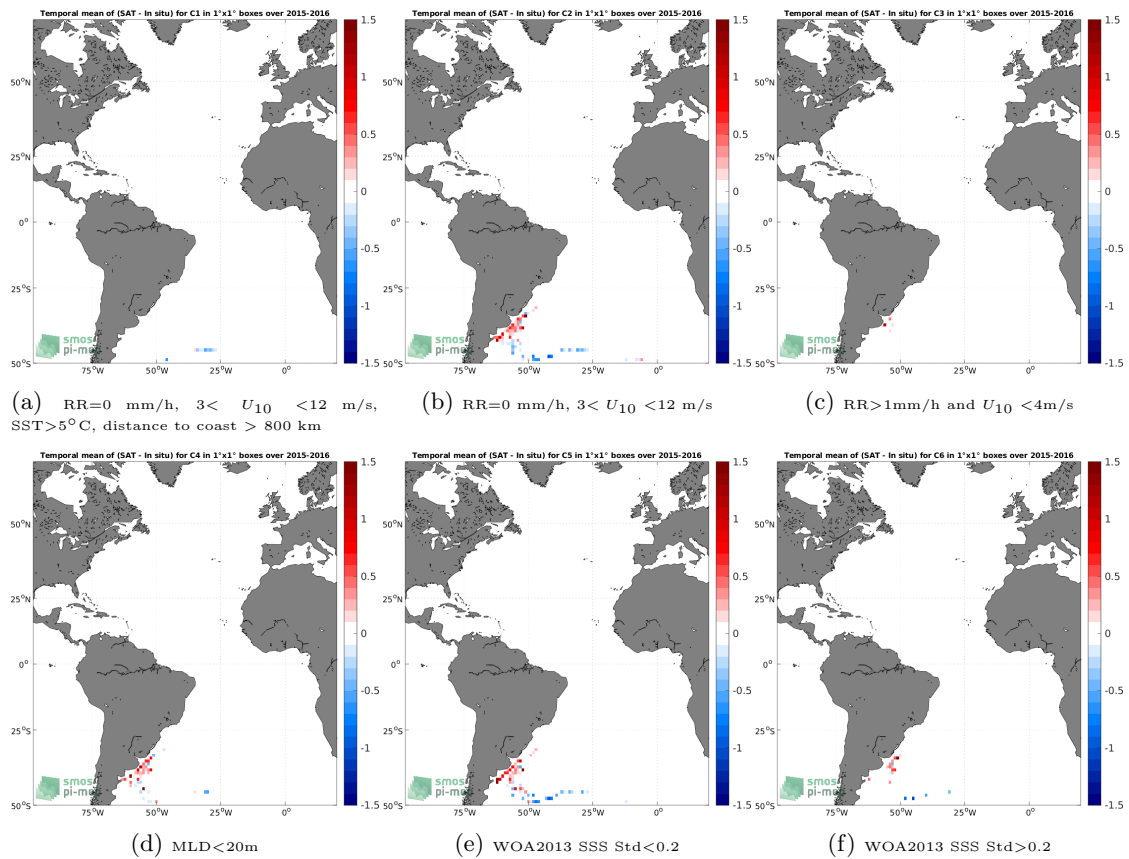
Figure 12: Temporal mean gridded over spatial boxes of size 1^\circ \times 1^\circ of \Delta SSS (SMAP SSS L3 v5 - 8-Day running (RSS) - Marine mammals) for 6 different subdatasets corresponding to:RR=0 mm/h, 3 < U_{10} < 12 m/s, SST >5^\circ C, distance to coast > 800 km (a), RR=0 mm/h, 3 < U_{10} < 12 m/s (b), RR >1 mm/h and U_{10} < 4 m/s (c),MLD <20 m (d),WOA2013 SSS Std <0.2 (e),WOA2013 SSS Std >0.2 (f).
