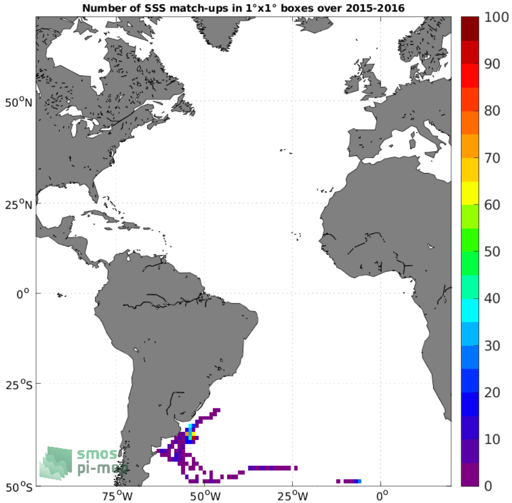
Figure 4: Number of SSS match-ups between Marine mammals SSS and the SMAP SSS L3 v5 - 8-Day running (RSS) SSS product for the Atlantic Ocean Pi-MEP region over 1°x1° boxes and for the full satellite product period.
