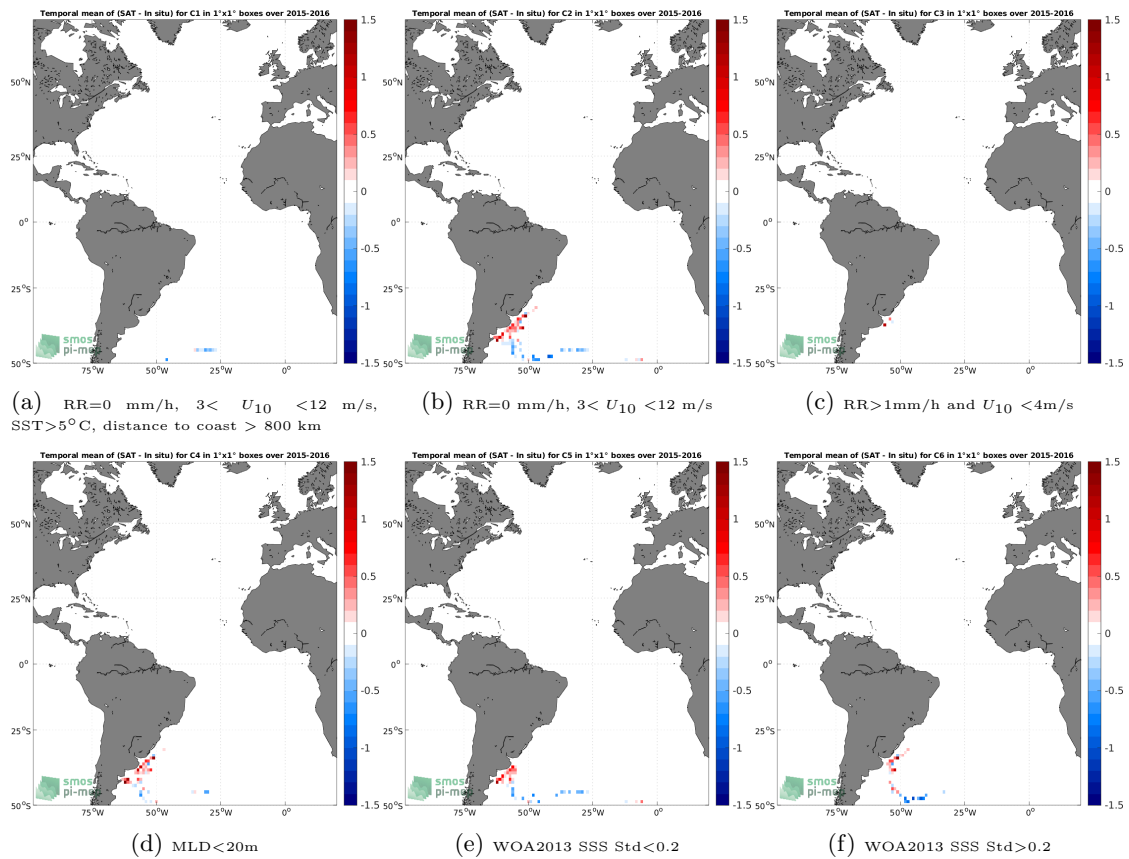
Figure 12: Temporal mean gridded over spatial boxes of size 1^\circ \times 1^\circ of \Delta SSS (SMAP SSS L3 v5 - 8-Day running (RSS) - Marine mammals) for 6 different subdatasets corresponding to: RR=0 mm/h, 3 < U_{10} < 12 m/s, SST > 5°C, distance to coast > 800 km (a), RR=0 mm/h, 3 < U_{10} < 12 m/s (b), RR > 1mm/h and U_{10} < 4 m/s (c), MLD < 20m (d), WOA2013 SSS Std < 0.2 (e), WOA2013 SSS Std > 0.2 (f).
