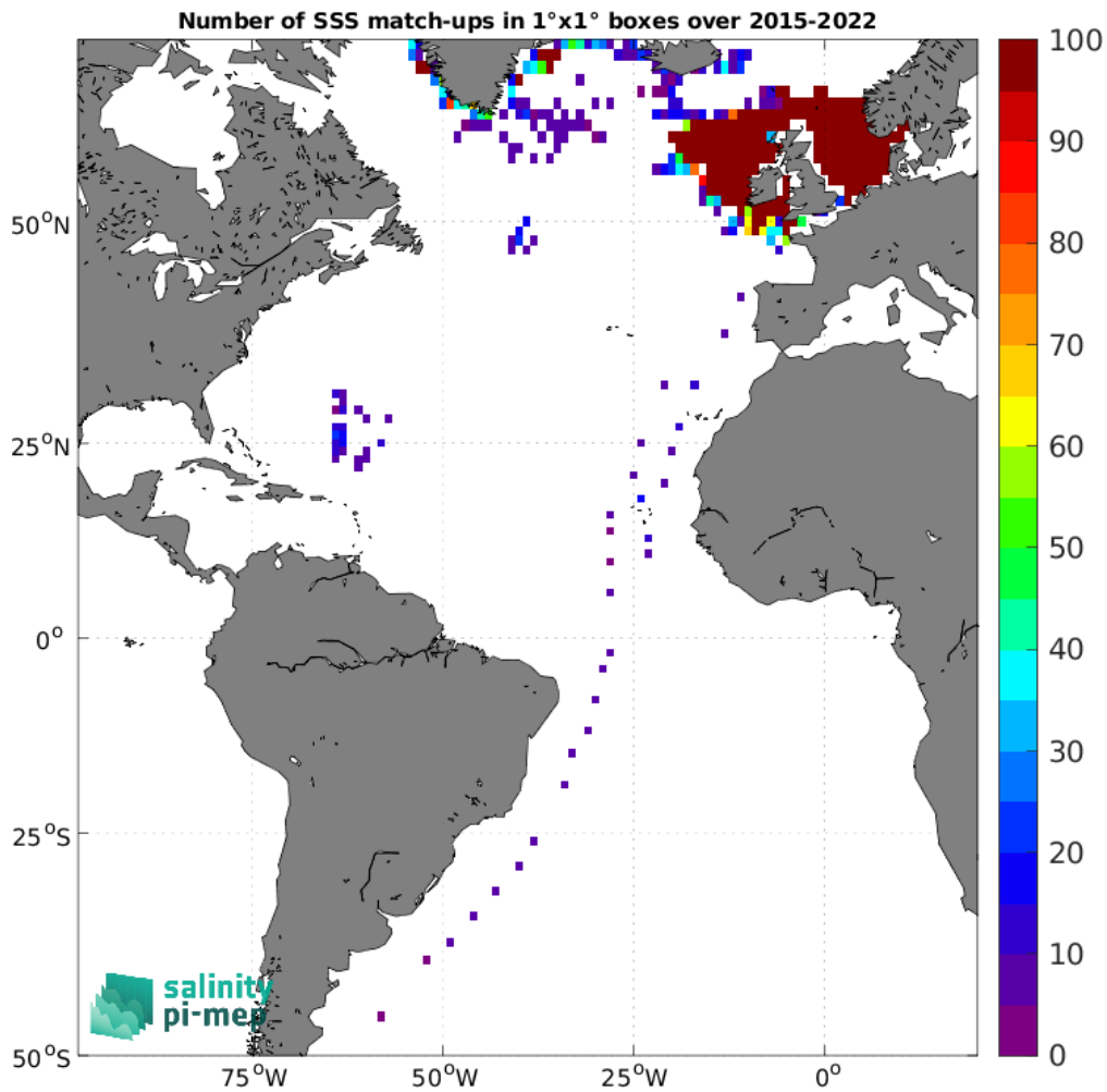
Figure 4: Number of SSS match-ups between ICES SSS and the SMAP SSS L3 v5 - 8-Day running (RSS) SSS product for the Atlantic Ocean Pi-MEP region over 1^\circ \times 1^\circ boxes and for the full satellite product period.
