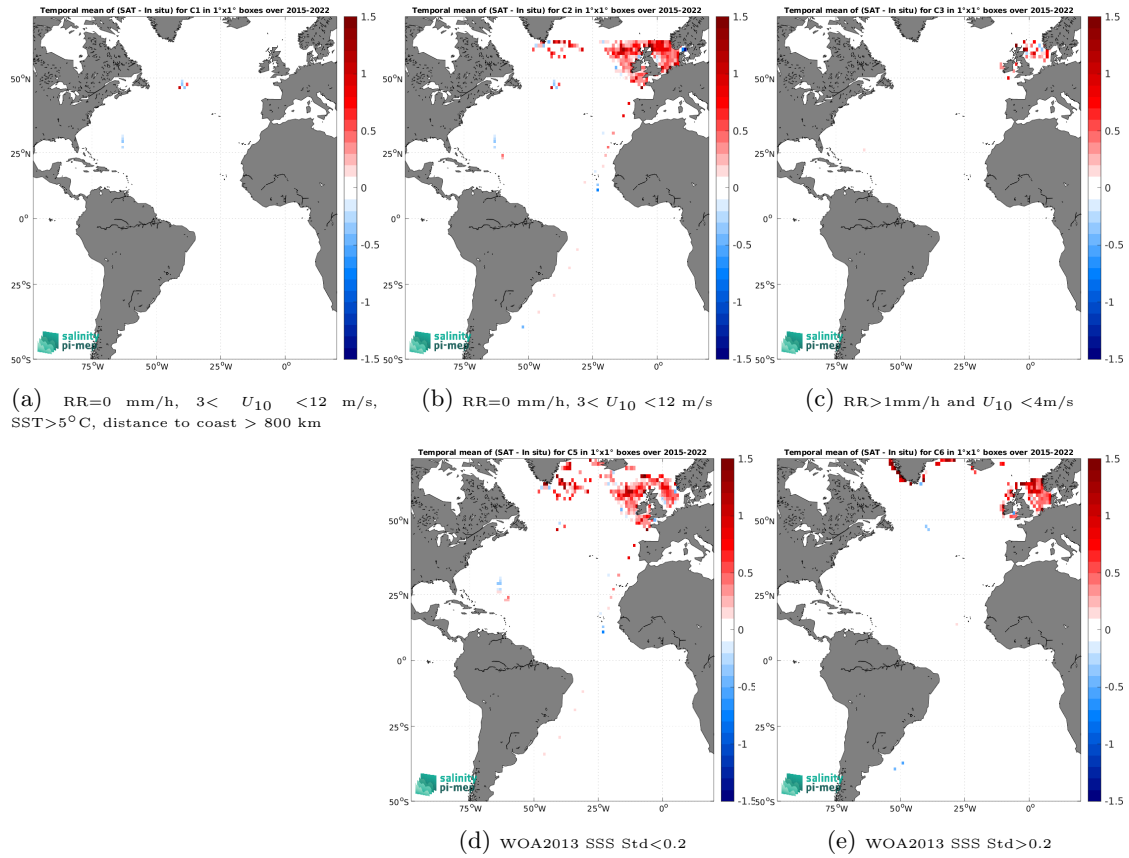
Figure 12: Temporal mean gridded over spatial boxes of size 1^\circ \times 1^\circ of \Delta SSS (SMAP SSS L3 v5 - 8-Day running (RSS) - ICES) for 5 different subdatasets corresponding to:RR=0 mm/h, 3 < U_{10} < 12 m/s, SST >5^\circ\text{C} , distance to coast > 800 km (a), RR=0 mm/h, 3 < U_{10} < 12 m/s (b), RR >1 mm/h and U_{10} < 4 m/s (c), WOA2013 SSS Std <0.2 (d), WOA2013 SSS Std >0.2 (e).
