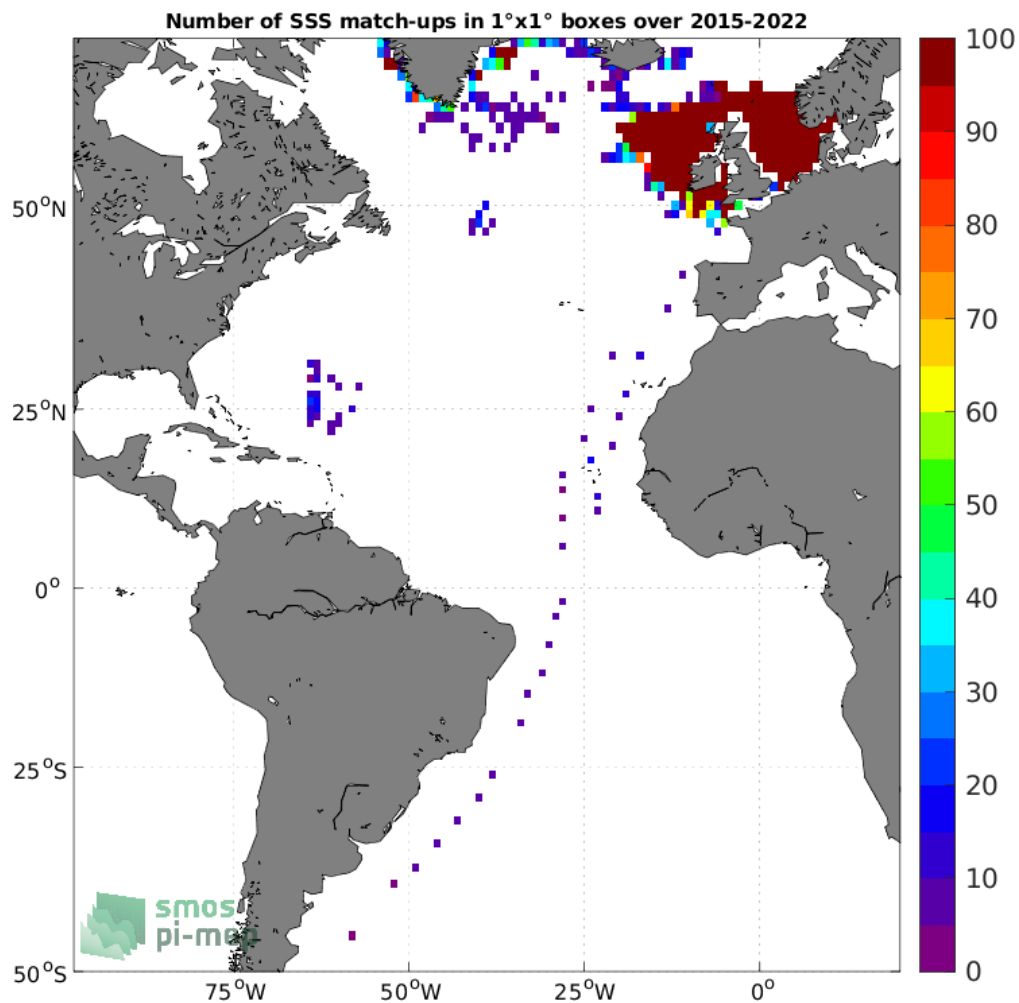
Figure 4: Number of SSS match-ups between ICES SSS and the SMAP SSS L3 v5 - 8-Day running (RSS) SSS product for the Atlantic Ocean Pi-MEP region over 1°x1° boxes and for the full satellite product period.
