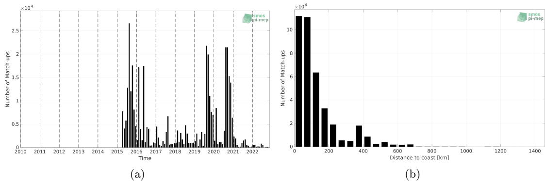
Figure 1: Number of match-ups between ICES and SMAP SSS L3 v5 - 8-Day running (RSS) SSS as a function of time (a) and as function of the distance to coast (b) over the Atlantic Ocean Pi-MEP region and for the full satellite product period.
