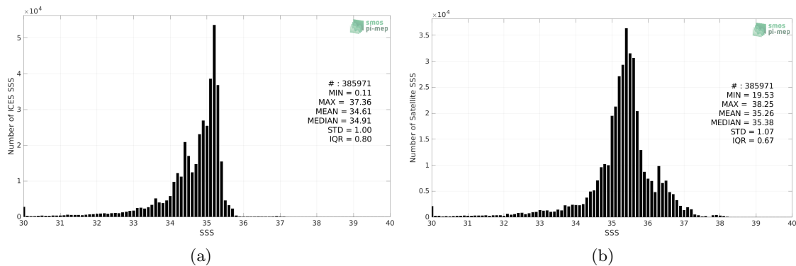
Figure 2: Histograms of SSS from ICES (a) and SMAP SSS L3 v5 - 8-Day running (RSS) (b) considering all match-up pairs per bins of 0.1 over the Atlantic Ocean Pi-MEP region and for the full satellite product period.
