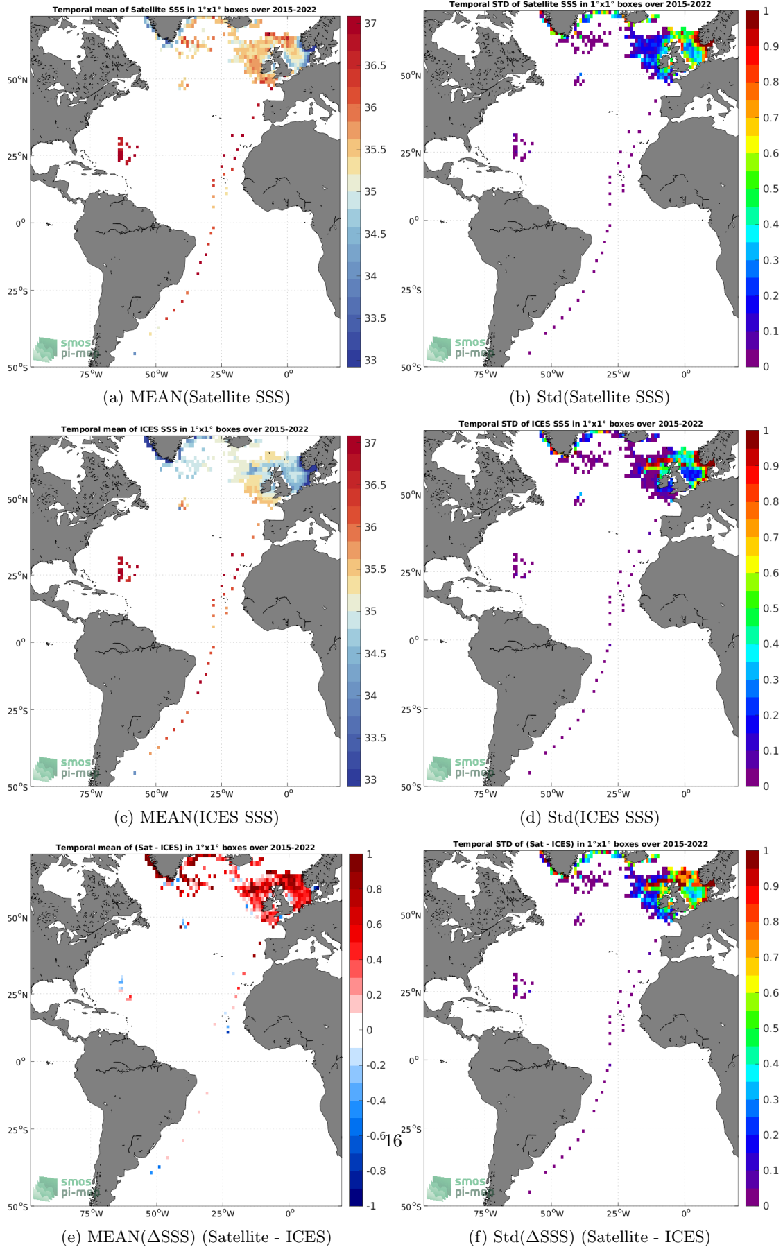
Figure 6: Temporal mean (left) and Std (right) of SSS from SMAP SSS L3 v5 - 8-Day running (RSS) (top), ICES (middle), and of \Delta SSS (Satellite - ICES). Only match-up pairs are used to generate these maps.
