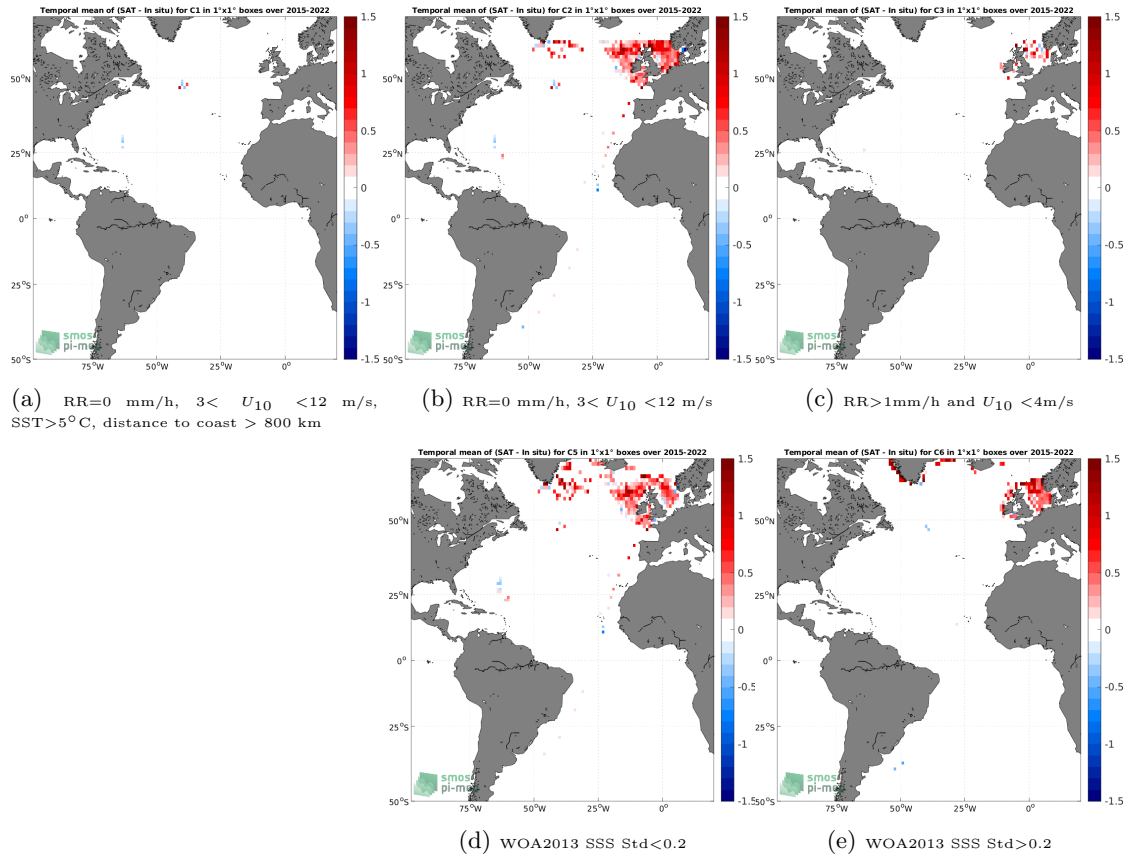
Figure 12: Temporal mean gridded over spatial boxes of size 1^\circ \times 1^\circ of \Delta SSS (SMAP SSS L3 v5 - 8-Day running (RSS) - ICES) for 5 different subdatasets corresponding to:RR=0 mm/h, 3 < U_{10} < 12 m/s, SST >5^\circ\text{C} , distance to coast > 800 km (a), RR=0 mm/h, 3 < U_{10} < 12 m/s (b), RR >1 mm/h and U_{10} < 4 m/s (c), WOA2013 SSS Std <0.2 (d), WOA2013 SSS Std >0.2 (e).
