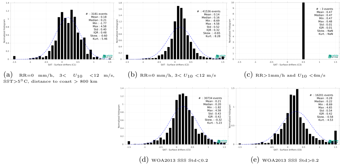
Figure 12: Normalized histogram of \Delta\text{SSS} (SMAP SSS L3 v5 - 8-Day running (RSS) - Surface drifters) for 5 different subdatasets corresponding to: RR=0 mm/h, 3 < U_{10} < 12 m/s, SST>5°C, distance to coast > 800 km (a), RR=0 mm/h, 3 < U_{10} < 12 m/s (b), RR>1mm/h and U_{10} < 4 m/s (c), WOA2013 SSS Std<0.2 (d), WOA2013 SSS Std>0.2 (e).
