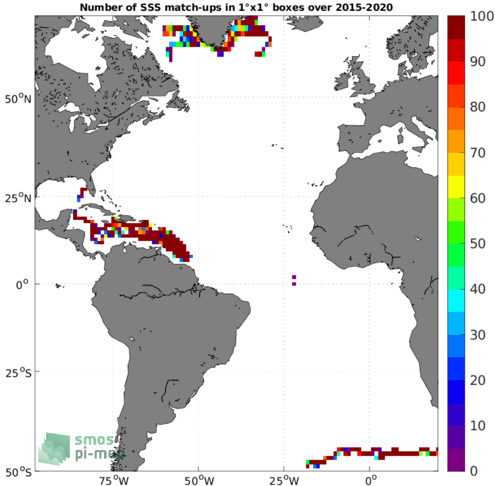
Figure 3: Number of SSS match-ups between Surface drifters SSS and the SMAP SSS L3 v5 - 8-Day running (RSS) SSS product for the Atlantic Ocean Pi-MEP region over 1^\circ \times 1^\circ boxes and for the full satellite product period.
