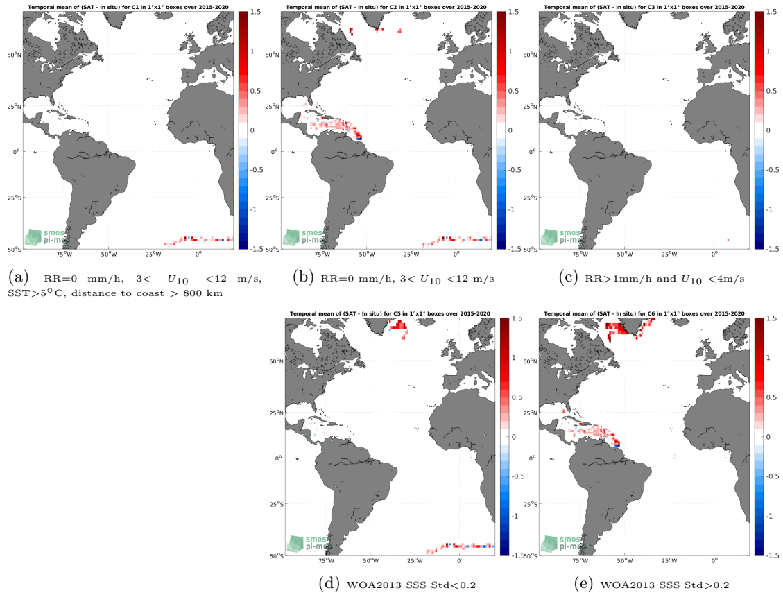
Figure 11: Temporal mean gridded over spatial boxes of size 1^\circ \times 1^\circ of \Delta SSS (SMAP SSS L3 v5 - 8-Day running (RSS) - Surface drifters) for 5 different subdatasets corresponding to:RR=0 mm/h, 3 < U_{10} < 12 m/s, SST >5^\circ\text{C} , distance to coast > 800 km (a), RR=0 mm/h, 3 < U_{10} < 12 m/s (b), RR >1 mm/h and U_{10} < 4 m/s (c), WOA2013 SSS Std <0.2 (d), WOA2013 SSS Std >0.2 (e).
