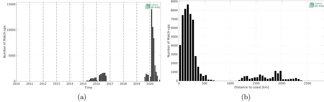
Figure 1: Number of match-ups between Surface drifters and SMAP SSS L3 v5 - 8-Day running (RSS) SSS as a function of time (a) and as function of the distance to coast (b) over the Atlantic Ocean Pi-MEP region and for the full satellite product period.
