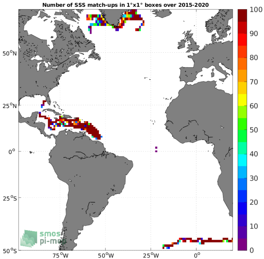
Figure 3: Number of SSS match-ups between Surface drifters SSS and the SMAP SSS L3 v5 - 8-Day running (RSS) SSS product for the Atlantic Ocean Pi-MEP region over 1°×1° boxes and for the full satellite product period.
