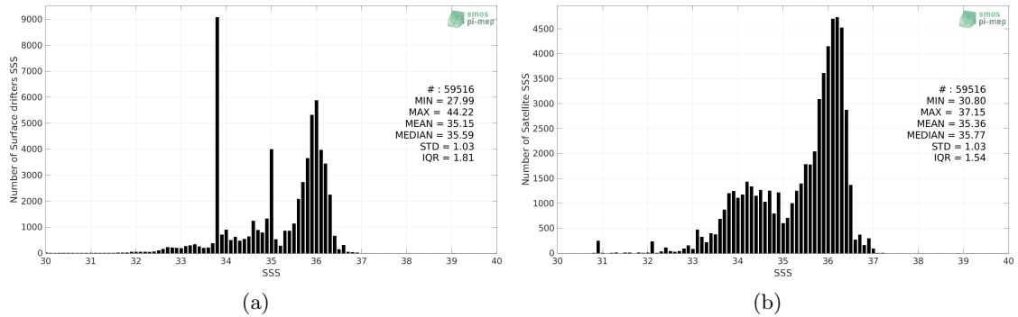
Figure 2: Histograms of SSS from Surface drifters (a) and SMAP SSS L3 v5 - 8-Day running (RSS) (b) considering all match-up pairs per bins of 0.1 over the Atlantic Ocean Pi-MEP region and for the full satellite product period.
