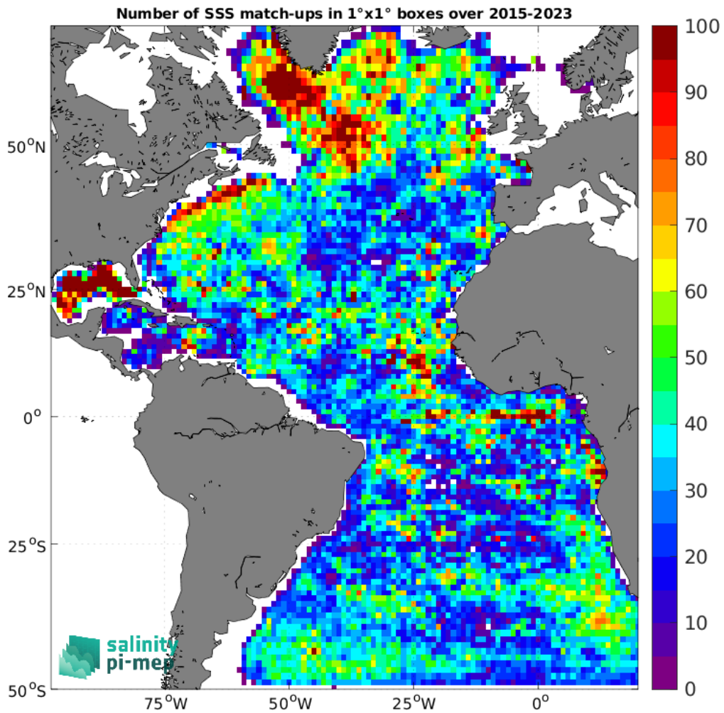
Figure 4: Number of SSS match-ups between Argo SSS and the SMAP SSS L3 v5 - 8-Day running (RSS) SSS product for the Atlantic Ocean Pi-MEP region over 1^{\circ} \times 1^{\circ} boxes and for the full satellite product period.
