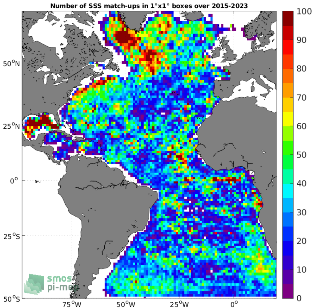
Figure 4: Number of SSS match-ups between Argo SSS and the SMAP SSS L3 v5 - 8-Day running (RSS) SSS product for the Atlantic Ocean Pi-MEP region over 1°×1° boxes and for the full satellite product period.
