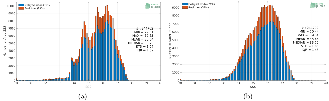
Figure 2: Histograms of SSS from Argo (a) and SMAP SSS L3 v5 - 8-Day running (RSS) (b) considering all match-up pairs per bins of 0.1 over the Atlantic Ocean Pi-MEP region and for the full satellite product period.
