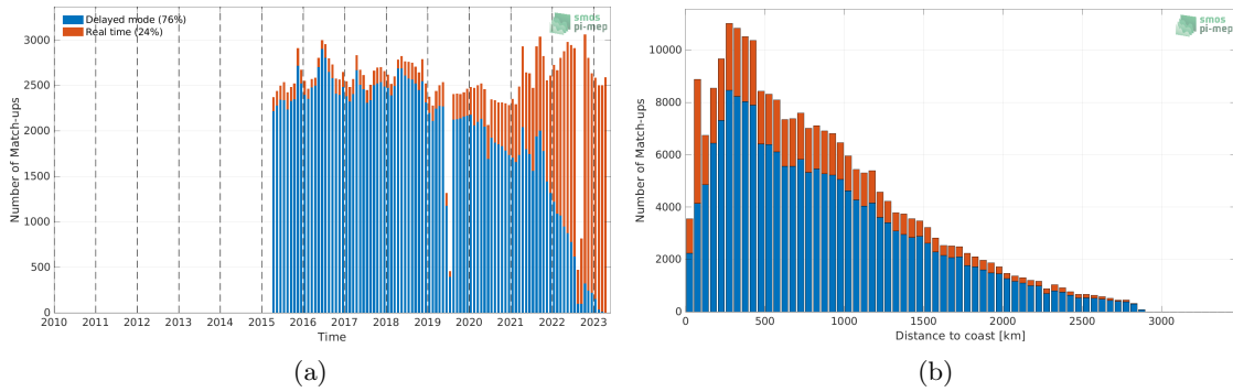
Figure 1: Number of match-ups between Argo and SMAP SSS L3 v5 - 8-Day running (RSS) SSS as a function of time (a) and as function of the distance to coast (b) over the Atlantic Ocean Pi-MEP region and for the full satellite product period.
