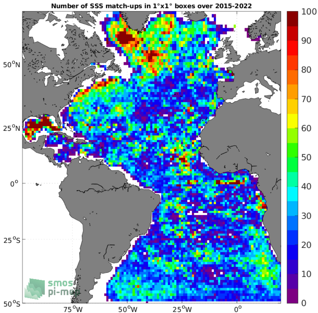
Figure 4: Number of SSS match-ups between Argo SSS and the SMAP SSS L3 v5 - 8-Day running (RSS) SSS product for the Atlantic Ocean Pi-MEP region over 1^\circ \times 1^\circ boxes and for the full satellite product period.
