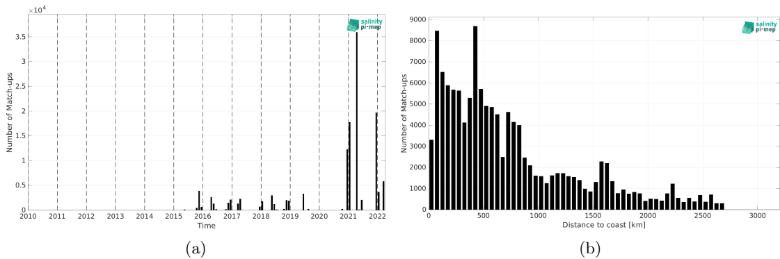
Figure 1: Number of match-ups between TSG (Polarstern) and SMAP SSS L3 v5 - Monthly (RSS) SSS as a function of time (a) and as function of the distance to coast (b) over the Atlantic Ocean Pi-MEP region and for the full satellite product period.
