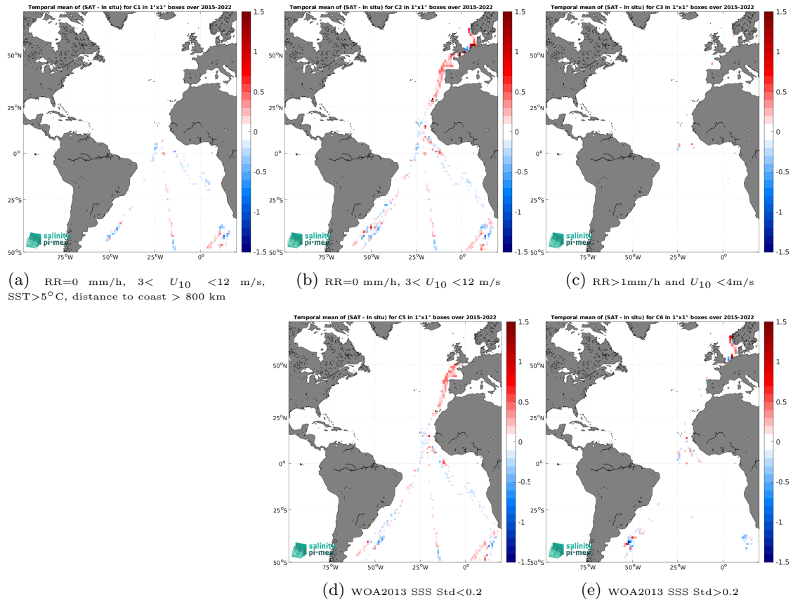
Figure 12: Temporal mean gridded over spatial boxes of size 1^\circ \times 1^\circ of \Delta SSS (SMAP SSS L3 v5 - Monthly (RSS) - TSG (Polarstern)) for 5 different subdatasets corresponding to:RR=0 mm/h, 3 < U_{10} < 12 m/s, SST >5^\circ\text{C} , distance to coast > 800 km (a), RR=0 mm/h, 3 < U_{10} < 12 m/s (b), RR >1 mm/h and U_{10} < 4 m/s (c), WOA2013 SSS Std <0.2 (d), WOA2013 SSS Std >0.2 (e).
