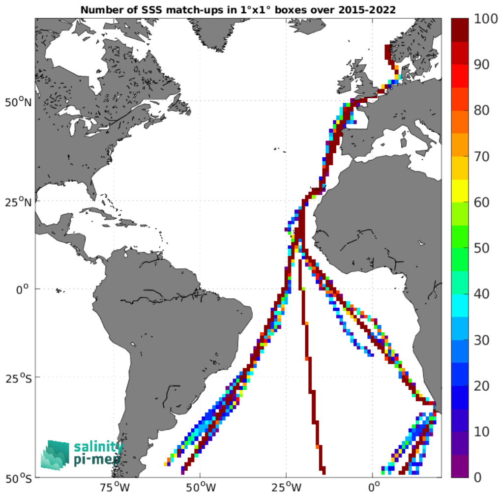
Figure 4: Number of SSS match-ups between TSG (Polarstern) SSS and the SMAP SSS L3 v5 - Monthly (RSS) SSS product for the Atlantic Ocean Pi-MEP region over 1^\circ \times 1^\circ boxes and for the full satellite product period.
