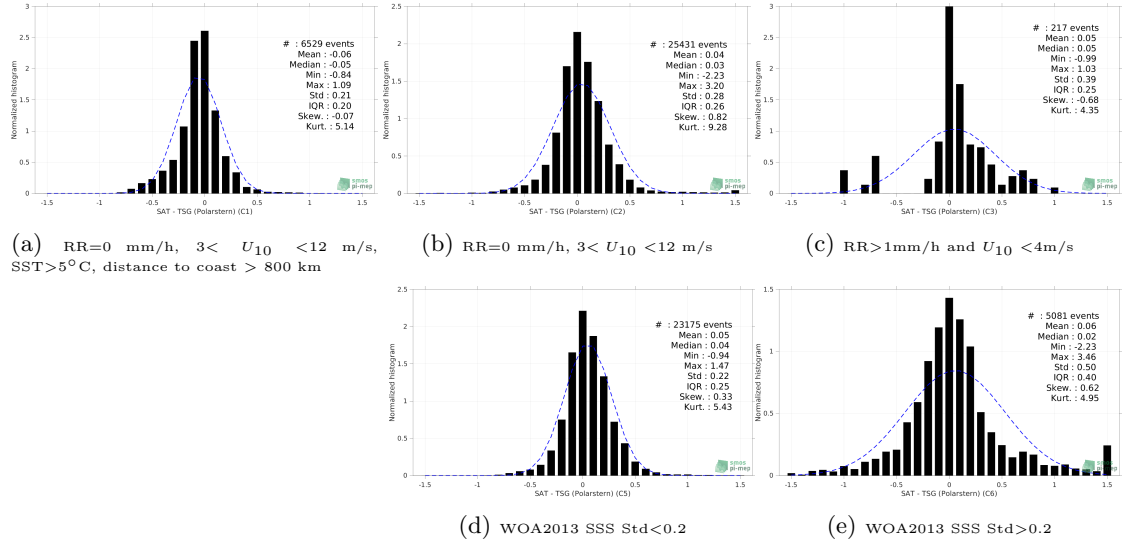
Figure 13: Normalized histogram of \Delta SSS (SMAP SSS L3 v5 - Monthly (RSS) - TSG (Polarstern)) for 5 different subdatasets corresponding to: RR=0 mm/h, 3 < U_{10} < 12 m/s, SST >5^{\circ}\text{C} , distance to coast > 800 km (a), RR=0 mm/h, 3 < U_{10} < 12 m/s (b), RR >1 mm/h and U_{10} < 4 m/s (c), WOA2013 SSS Std <0.2 (d), WOA2013 SSS Std >0.2 (e).
