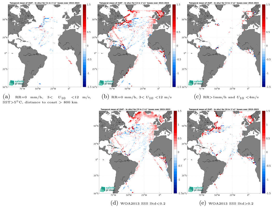
Figure 12: Temporal mean gridded over spatial boxes of size 1^\circ \times 1^\circ of \Delta SSS (SMAP SSS L3 v5 - Monthly (RSS) - TSG (LEGOS-DM)) for 5 different subdatasets corresponding to:RR=0 mm/h, 3 < U_{10} < 12 m/s, SST >5^\circ\text{C} , distance to coast > 800 km (a), RR=0 mm/h, 3 < U_{10} < 12 m/s (b), RR >1 mm/h and U_{10} < 4 m/s (c), WOA2013 SSS Std <0.2 (d), WOA2013 SSS Std >0.2 (e).
