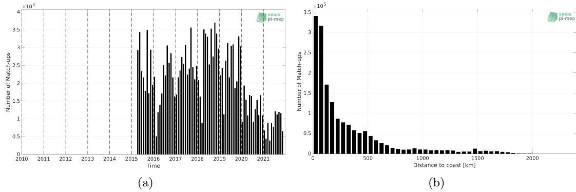
Figure 1: Number of match-ups between TSG (LEGOS-DM) and SMAP SSS L3 v5 - Monthly (RSS) SSS as a function of time (a) and as function of the distance to coast (b) over the Atlantic Ocean Pi-MEP region and for the full satellite product period.
