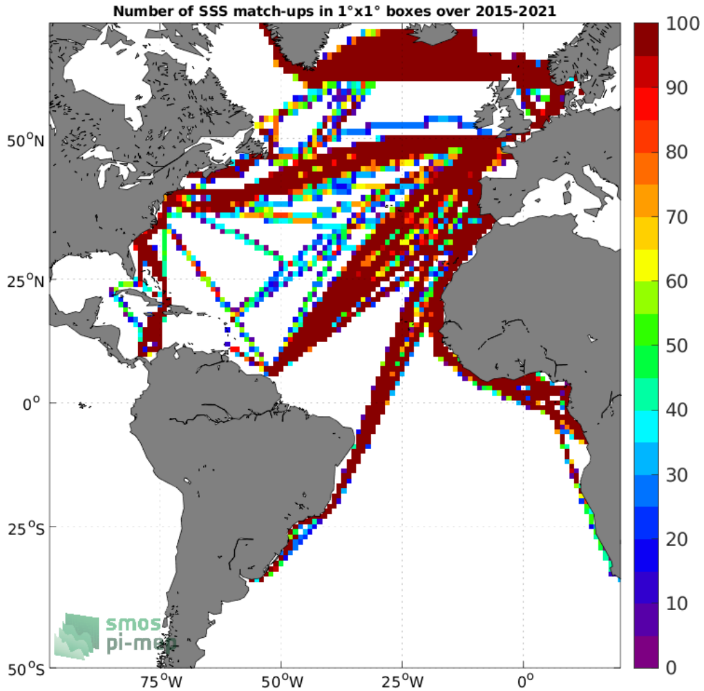
Figure 4: Number of SSS match-ups between TSG (LEGOS-DM) SSS and the SMAP SSS L3 v5 - Monthly (RSS) SSS product for the Atlantic Ocean Pi-MEP region over 1°x1° boxes and for the full satellite product period.
