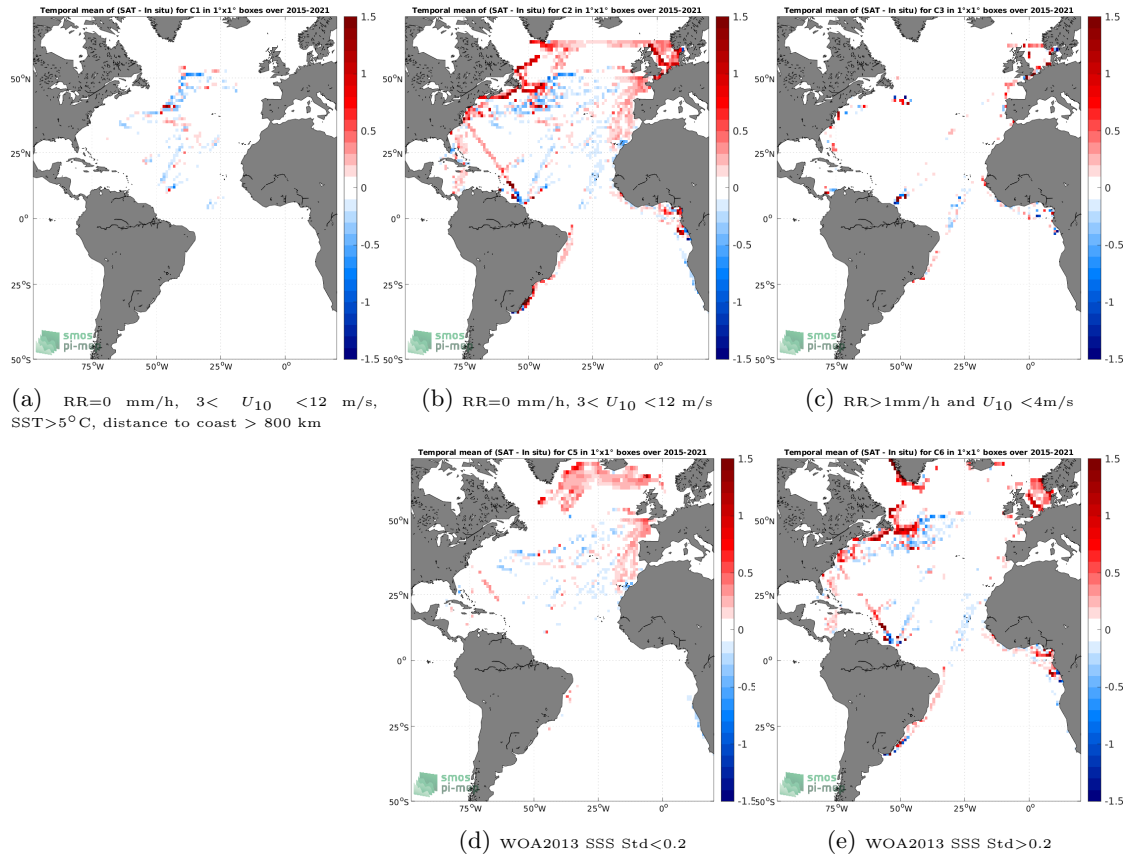
Figure 12: Temporal mean gridded over spatial boxes of size 1^\circ \times 1^\circ of \Delta\text{SSS} (SMAP SSS L3 v5 - Monthly (RSS) - TSG (LEGOS-DM)) for 5 different subdatasets corresponding to:RR=0 mm/h, 3 < U_{10} < 12 m/s, SST >5^\circ\text{C} , distance to coast > 800 km (a), RR=0 mm/h, 3 < U_{10} < 12 m/s (b), RR >1 mm/h and U_{10} < 4 m/s (c), WOA2013 SSS Std <0.2 (d), WOA2013 SSS Std >0.2 (e).
