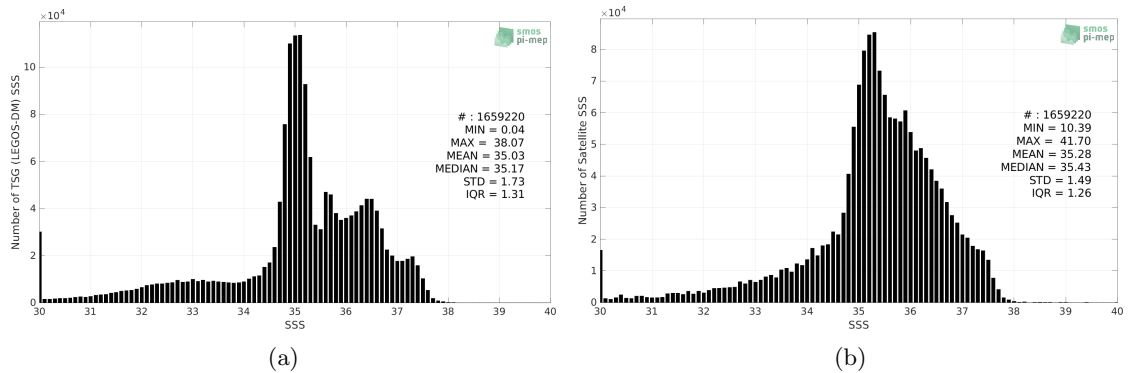
Figure 2: Histograms of SSS from TSG (LEGOS-DM) (a) and SMAP SSS L3 v5 - Monthly (RSS) (b) considering all match-up pairs per bins of 0.1 over the Atlantic Ocean Pi-MEP region and for the full satellite product period.
