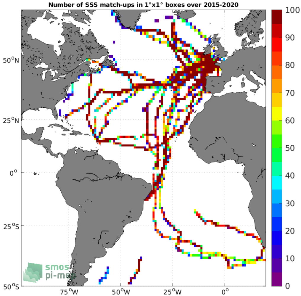
Figure 4: Number of SSS match-ups between TSG (GOSUD-Sailing-ship) SSS and the SMAP SSS L3 v5 - Monthly (RSS) SSS product for the Atlantic Ocean Pi-MEP region over 1°x1° boxes and for the full satellite product period.
