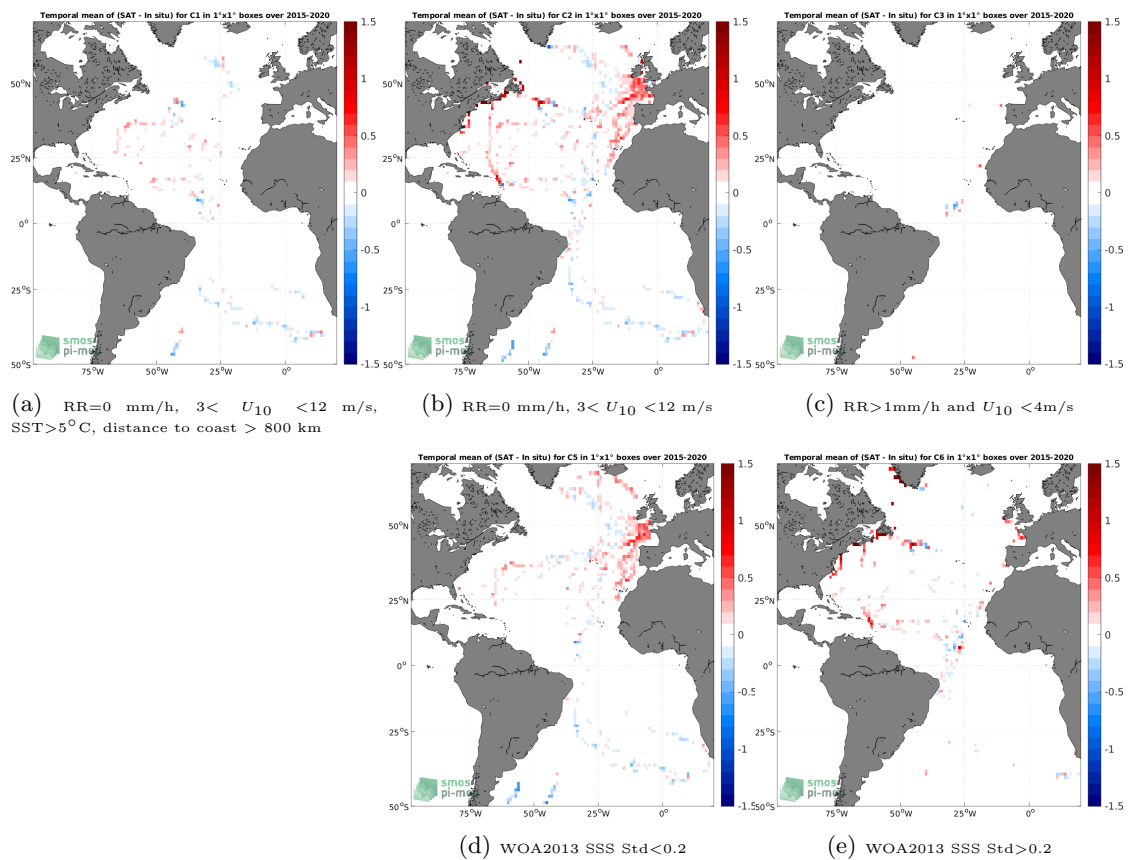
Figure 12: Temporal mean gridded over spatial boxes of size 1^\circ \times 1^\circ of \Delta SSS (SMAP SSS L3 v5 - Monthly (RSS) - TSG (GOSUD-Sailing-ship)) for 5 different subdatasets corresponding to:RR=0 mm/h, 3 < U_{10} < 12 m/s, SST>5°C, distance to coast > 800 km (a), RR=0 mm/h, 3 < U_{10} < 12 m/s (b), RR>1mm/h and U_{10} < 4 m/s (c), WOA2013 SSS Std<0.2 (d), WOA2013 SSS Std>0.2 (e).
