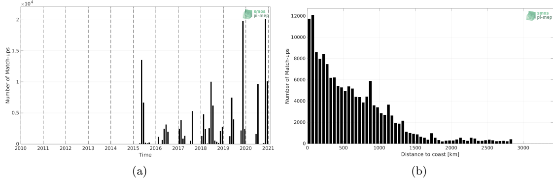
Figure 1: Number of match-ups between TSG (GOSUD-Sailing-ship) and SMAP SSS L3 v5 - Monthly (RSS) SSS as a function of time (a) and as function of the distance to coast (b) over the Atlantic Ocean Pi-MEP region and for the full satellite product period.
