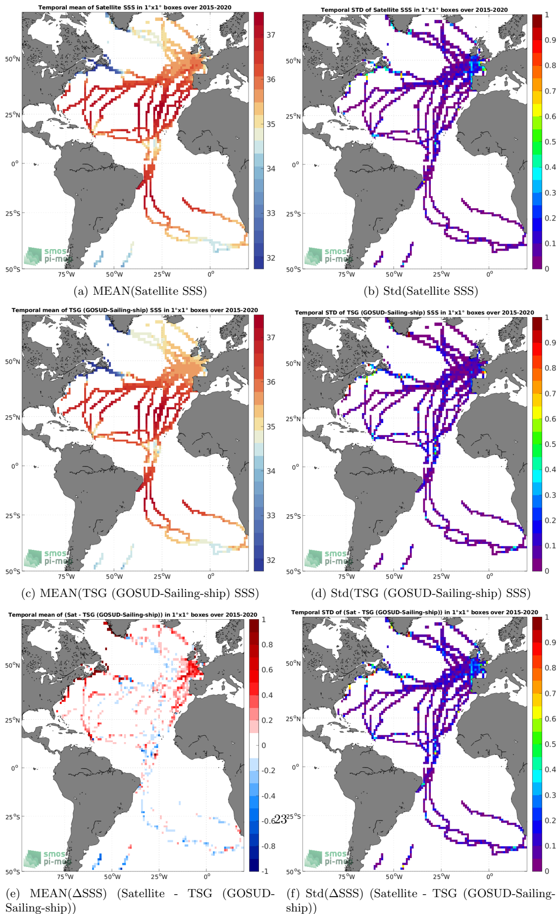
Figure 6: Temporal mean (left) and Std (right) of SSS from SMAP SSS L3 v5 - Monthly (RSS) (top), TSG (GOSUD-Sailing-ship) (middle), and of \Delta SSS (Satellite - TSG (GOSUD-Sailing-ship)). Only match-up pairs are used to generate these maps.
