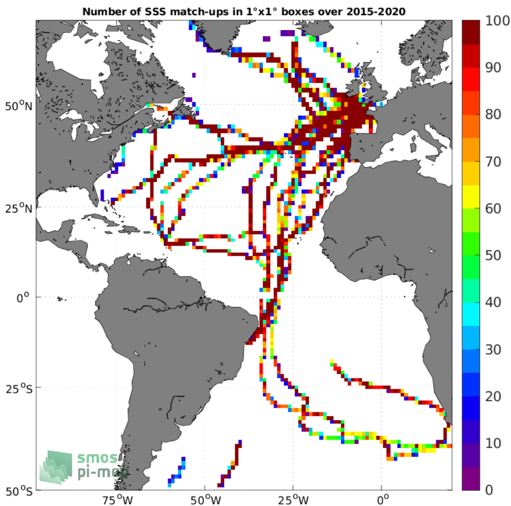
Figure 4: Number of SSS match-ups between TSG (GOSUD-Sailing-ship) SSS and the SMAP SSS L3 v5 - Monthly (RSS) SSS product for the Atlantic Ocean Pi-MEP region over 1^\circ \times 1^\circ boxes and for the full satellite product period.
