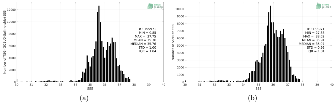
Figure 2: Histograms of SSS from TSG (GOSUD-Sailing-ship) (a) and SMAP SSS L3 v5 - Monthly (RSS) (b) considering all match-up pairs per bins of 0.1 over the Atlantic Ocean Pi-MEP region and for the full satellite product period.
