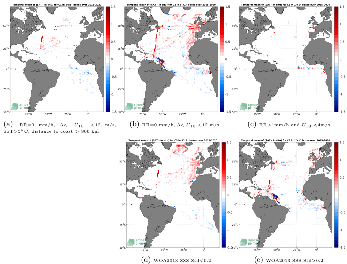
Figure 12: Temporal mean gridded over spatial boxes of size 1^\circ \times 1^\circ of \Delta\text{SSS} (SMAP SSS L3 v5 - Monthly (RSS) - TSG (GOSUD-Research-vessel)) for 5 different subdatasets corresponding to:RR=0 mm/h, 3 < U_{10} < 12 m/s, SST>5°C, distance to coast > 800 km (a), RR=0 mm/h, 3 < U_{10} < 12 m/s (b), RR>1mm/h and U_{10} < 4 m/s (c), WOA2013 SSS Std<0.2 (d), WOA2013 SSS Std>0.2 (e).
