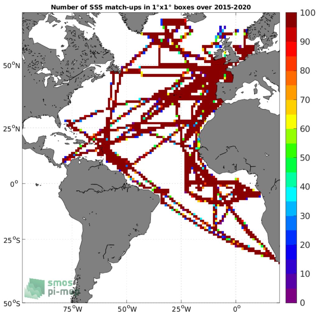
Figure 4: Number of SSS match-ups between TSG (GOSUD-Research-vessel) SSS and the SMAP SSS L3 v5 - Monthly (RSS) SSS product for the Atlantic Ocean Pi-MEP region over 1°x1° boxes and for the full satellite product period.
