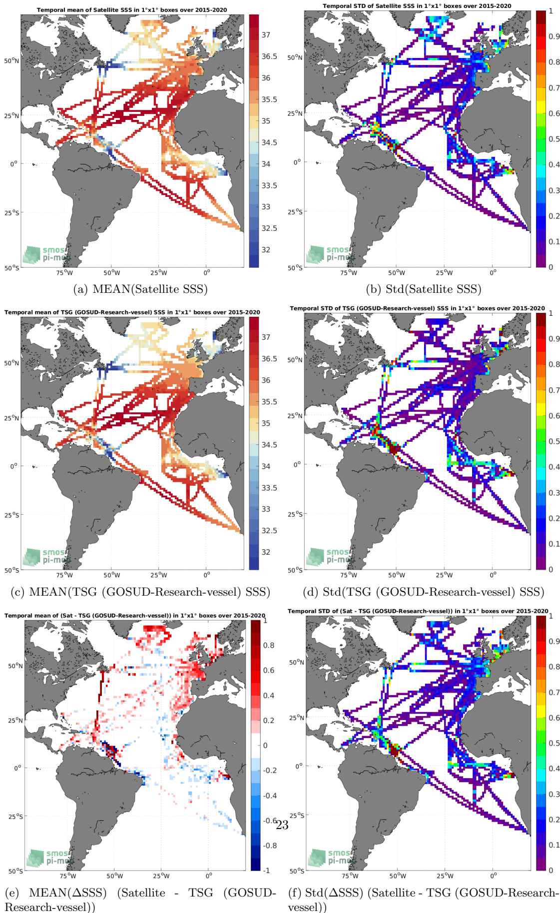
Figure 6: Temporal mean (left) and Std (right) of SSS from SMAP SSS L3 v5 - Monthly (RSS) (top), TSG (GOSUD-Research-vessel) (middle), and of \Delta SSS (Satellite - TSG (GOSUD-Research-vessel)). Only match-up pairs are used to generate these maps.
