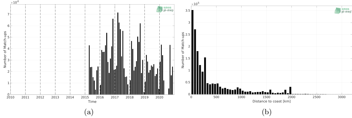
Figure 1: Number of match-ups between TSG (GOSUD-Research-vessel) and SMAP SSS L3 v5 - Monthly (RSS) SSS as a function of time (a) and as function of the distance to coast (b) over the Atlantic Ocean Pi-MEP region and for the full satellite product period.
