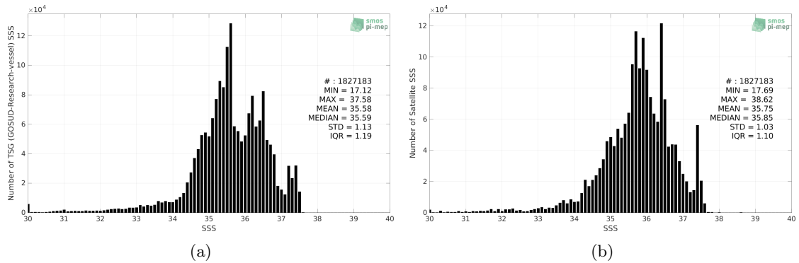
Figure 2: Histograms of SSS from TSG (GOSUD-Research-vessel) (a) and SMAP SSS L3 v5 - Monthly (RSS) (b) considering all match-up pairs per bins of 0.1 over the Atlantic Ocean Pi-MEP region and for the full satellite product period.
