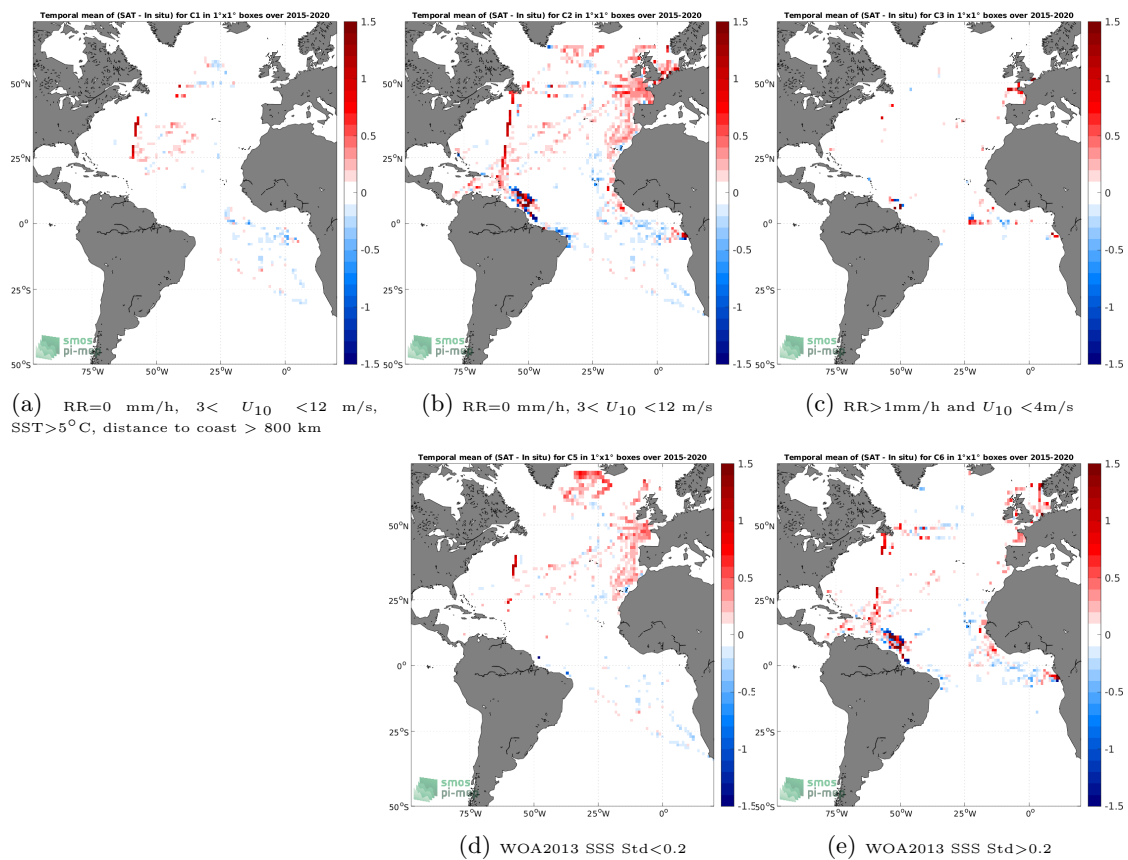
Figure 12: Temporal mean gridded over spatial boxes of size 1^\circ \times 1^\circ of \Delta SSS (SMAP SSS L3 v5 - Monthly (RSS) - TSG (GOSUD-Research-vessel)) for 5 different subdatasets corresponding to:RR=0 mm/h, 3 < U_{10} < 12 m/s, SST>5°C, distance to coast > 800 km (a), RR=0 mm/h, 3 < U_{10} < 12 m/s (b), RR>1mm/h and U_{10} < 4 m/s (c), WOA2013 SSS Std<0.2 (d), WOA2013 SSS Std>0.2 (e).
