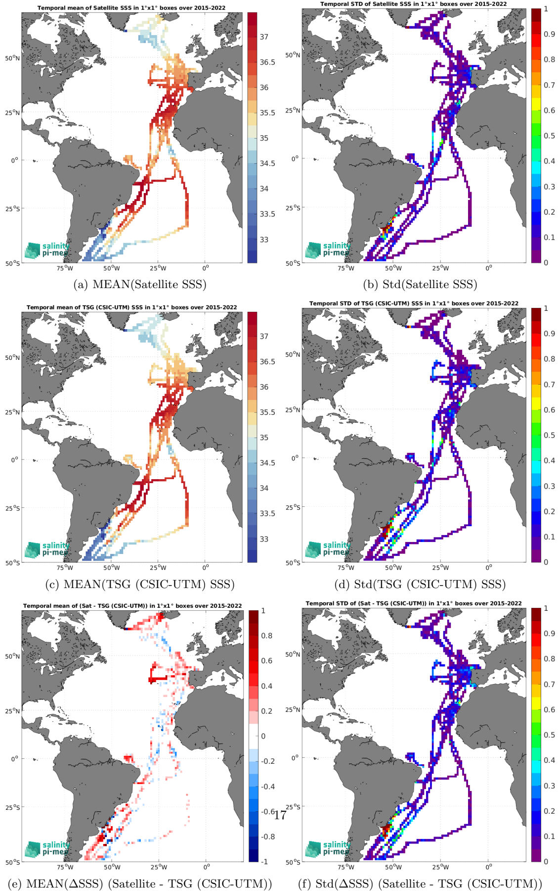
Figure 6: Temporal mean (left) and Std (right) of SSS from SMAP SSS L3 v5 - Monthly (RSS) (top), TSG (CSIC-UTM) (middle), and of \Delta SSS (Satellite - TSG (CSIC-UTM)). Only match-up pairs are used to generate these maps.
