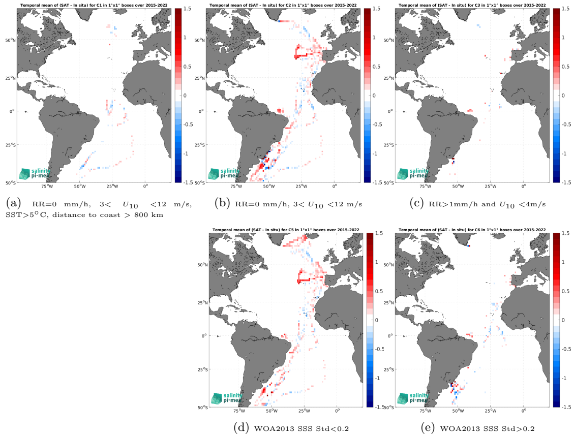
Figure 12: Temporal mean gridded over spatial boxes of size 1^\circ \times 1^\circ of \Delta SSS (SMAP SSS L3 v5 - Monthly (RSS) - TSG (CSIC-UTM)) for 5 different subdatasets corresponding to:RR=0 mm/h, 3 < U_{10} < 12 m/s, SST >5^\circ\text{C} , distance to coast > 800 km (a), RR=0 mm/h, 3 < U_{10} < 12 m/s (b), RR >1 mm/h and U_{10} < 4 m/s (c), WOA2013 SSS Std <0.2 (d), WOA2013 SSS Std >0.2 (e).
