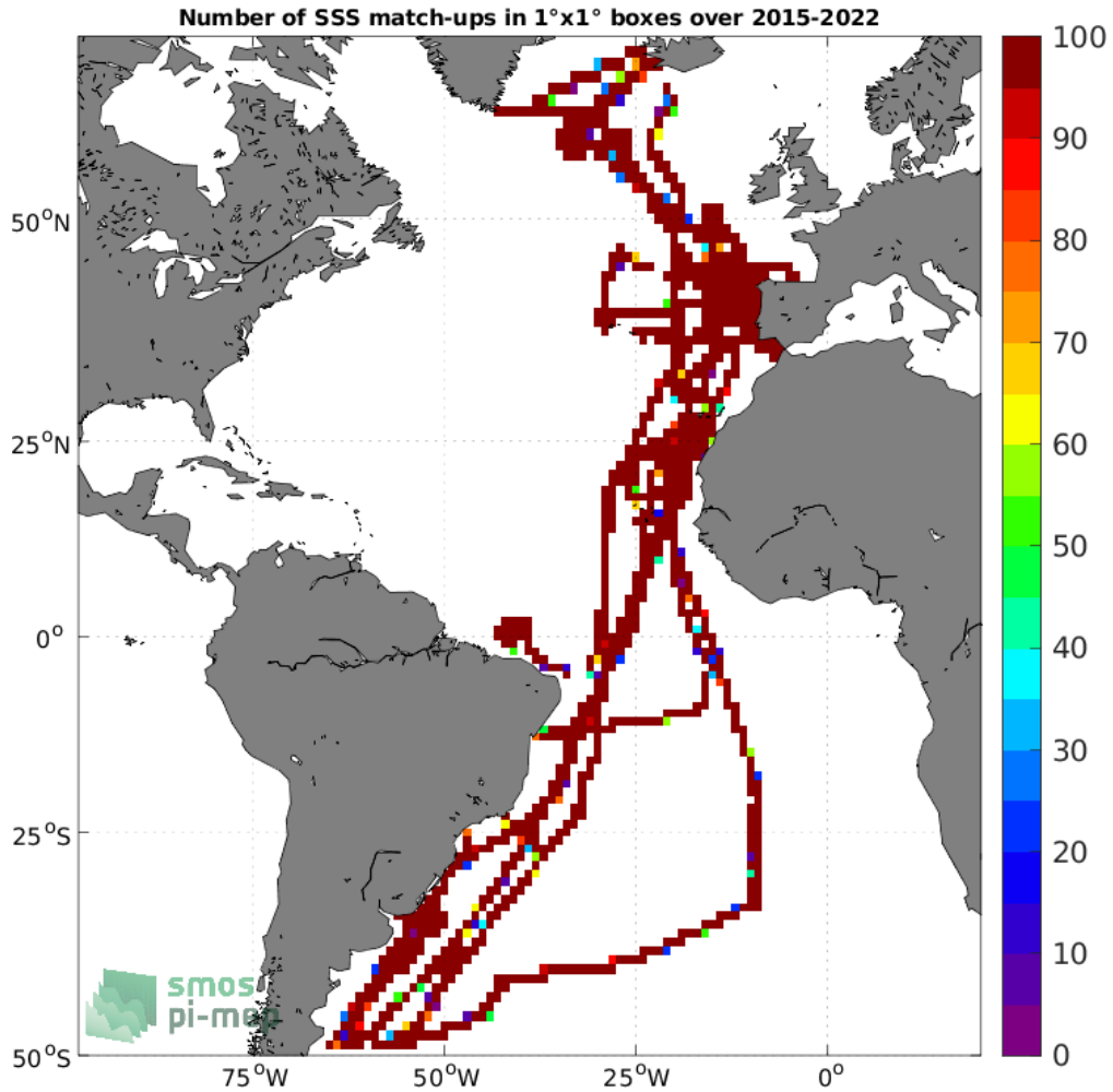
Figure 4: Number of SSS match-ups between TSG (CSIC-UTM) SSS and the SMAP SSS L3 v5 - Monthly (RSS) SSS product for the Atlantic Ocean Pi-MEP region over 1°x1° boxes and for the full satellite product period.
