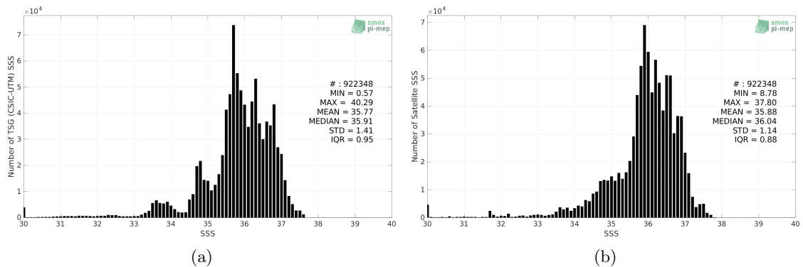
Figure 2: Histograms of SSS from TSG (CSIC-UTM) (a) and SMAP SSS L3 v5 - Monthly (RSS) (b) considering all match-up pairs per bins of 0.1 over the Atlantic Ocean Pi-MEP region and for the full satellite product period.
