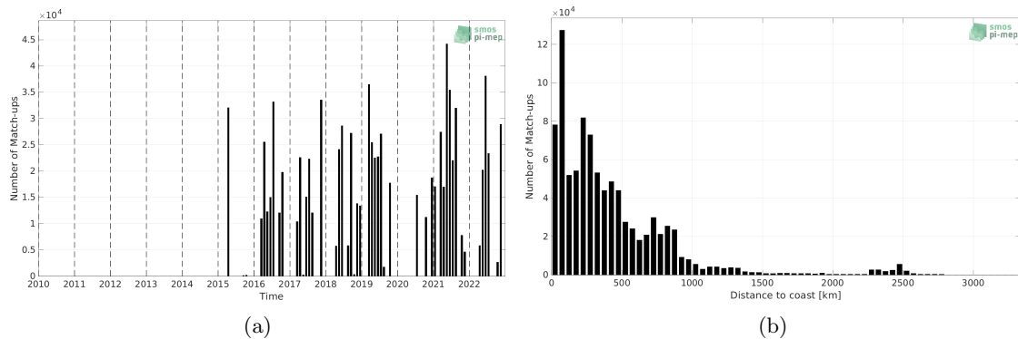
Figure 1: Number of match-ups between TSG (CSIC-UTM) and SMAP SSS L3 v5 - Monthly (RSS) SSS as a function of time (a) and as function of the distance to coast (b) over the Atlantic Ocean Pi-MEP region and for the full satellite product period.
