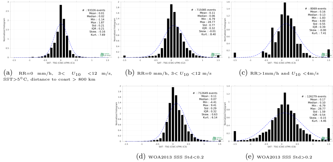
Figure 13: Normalized histogram of \Delta SSS (SMAP SSS L3 v5 - Monthly (RSS) - TSG (CSIC-UTM)) for 5 different subdatasets corresponding to: RR=0 mm/h, 3 < U_{10} < 12 m/s, SST > 5°C, distance to coast > 800 km (a), RR=0 mm/h, 3 < U_{10} < 12 m/s (b), RR > 1mm/h and U_{10} < 4 m/s (c), WOA2013 SSS Std < 0.2 (d), WOA2013 SSS Std > 0.2 (e).
