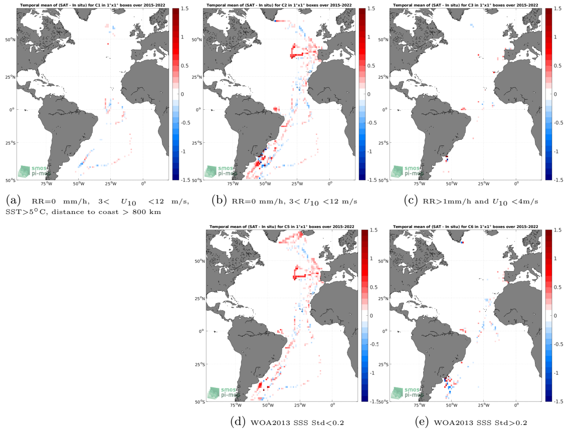
Figure 12: Temporal mean gridded over spatial boxes of size 1^\circ \times 1^\circ of \Delta SSS (SMAP SSS L3 v5 - Monthly (RSS) - TSG (CSIC-UTM)) for 5 different subdatasets corresponding to:RR=0 mm/h, 3 < U_{10} < 12 m/s, SST >5^\circ\text{C} , distance to coast > 800 km (a), RR=0 mm/h, 3 < U_{10} < 12 m/s (b), RR >1 mm/h and U_{10} < 4 m/s (c), WOA2013 SSS Std <0.2 (d), WOA2013 SSS Std >0.2 (e).
