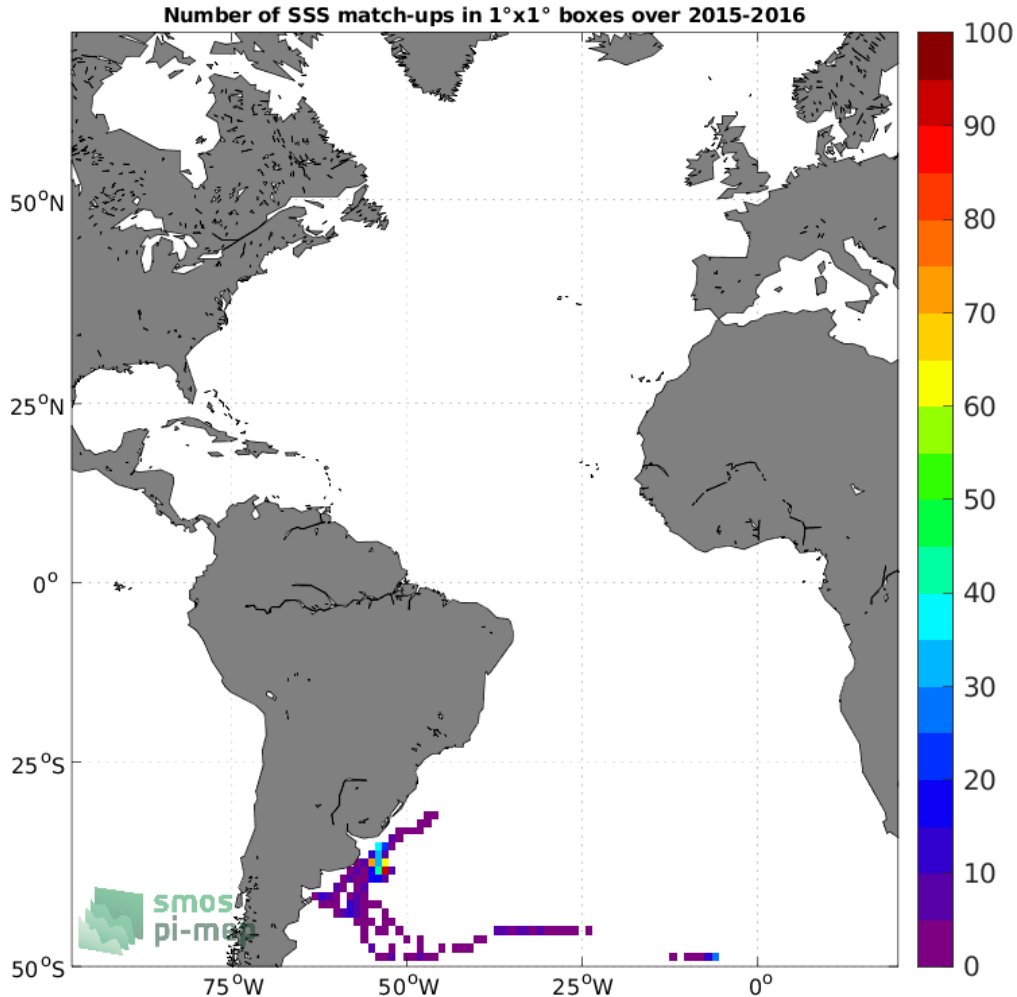
Figure 4: Number of SSS match-ups between Marine mammals SSS and the SMAP SSS L3 v5 - Monthly (RSS) SSS product for the Atlantic Ocean Pi-MEP region over 1^\circ \times 1^\circ boxes and for the full satellite product period.
