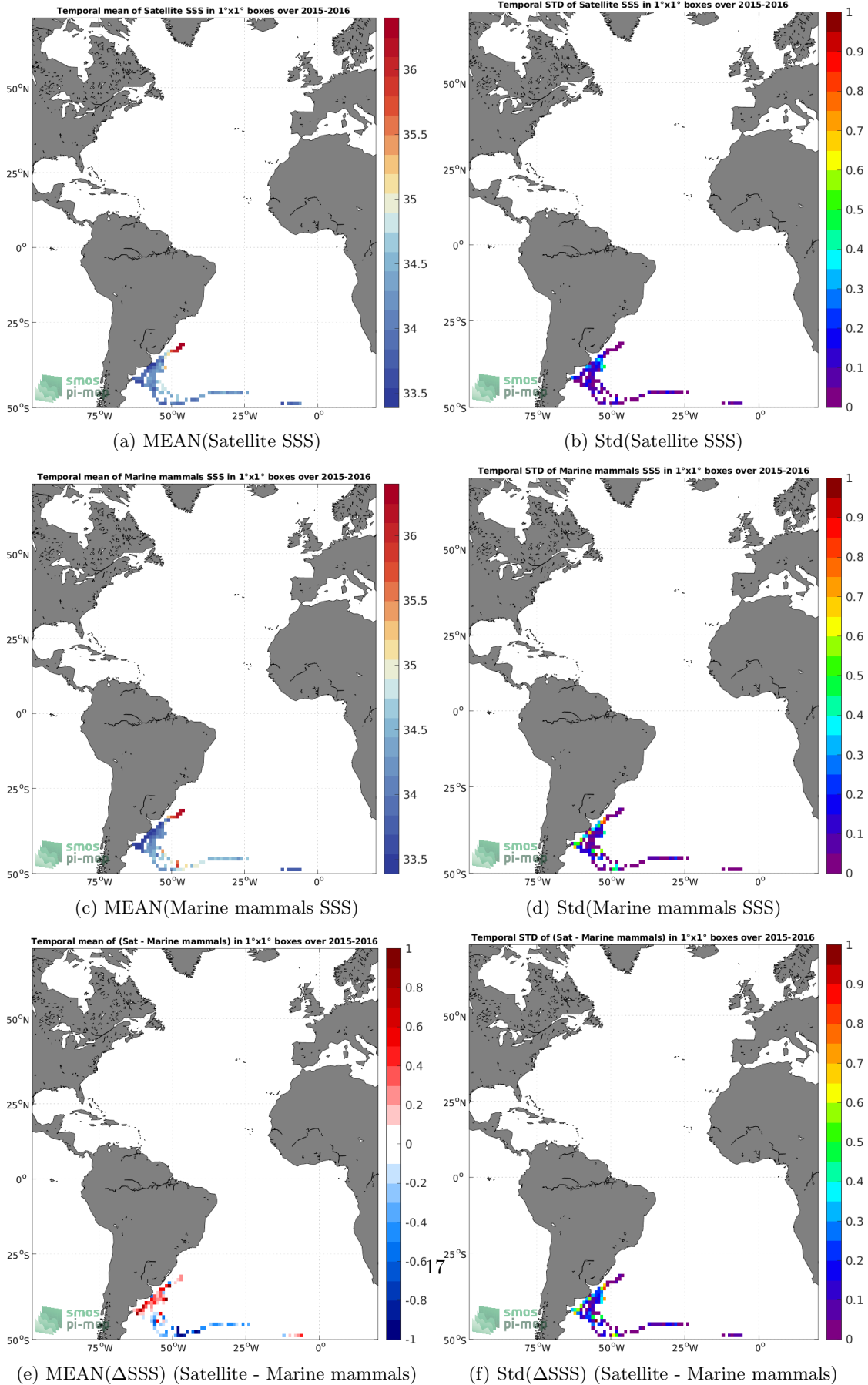
Figure 6: Temporal mean (left) and Std (right) of SSS from SMAP SSS L3 v5 - Monthly (RSS) (top), Marine mammals (middle), and of \Delta SSS (Satellite - Marine mammals). Only match-up pairs are used to generate these maps.
