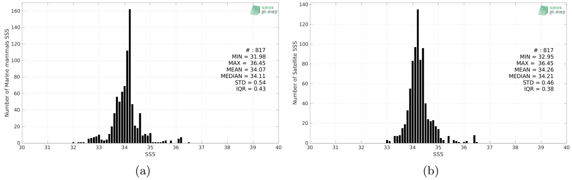
Figure 2: Histograms of SSS from Marine mammals (a) and SMAP SSS L3 v5 - Monthly (RSS) (b) considering all match-up pairs per bins of 0.1 over the Atlantic Ocean Pi-MEP region and for the full satellite product period.
